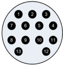
DIL13M FACE VIEW
