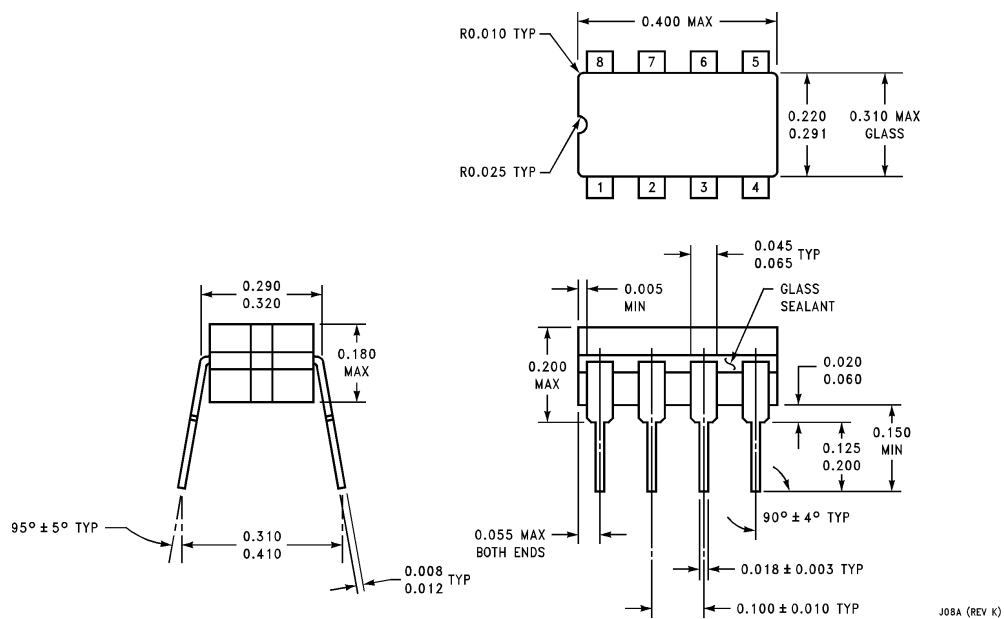
8-Pin Ceramic Dual-In-Line Package (J) Order Number LM6121J/883 NS Package Number J08A
