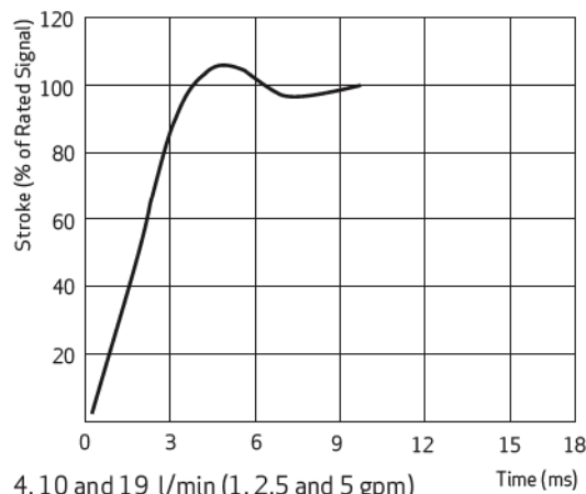
4, 10 and 19 l/min (1, 2.5 and 5 gpm) Plot @ 210 bar (3,000 psi)
