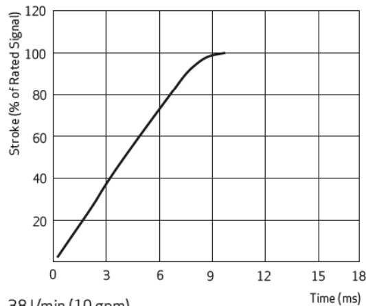
38 l/min (10 gpm) Plot @ 210 bar (3,000 psi)
