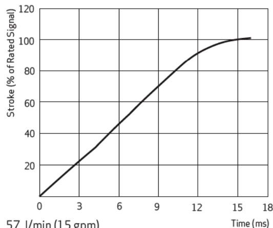
57 l/min (15 gpm) Plot @ 210 bar (3,000 psi)
