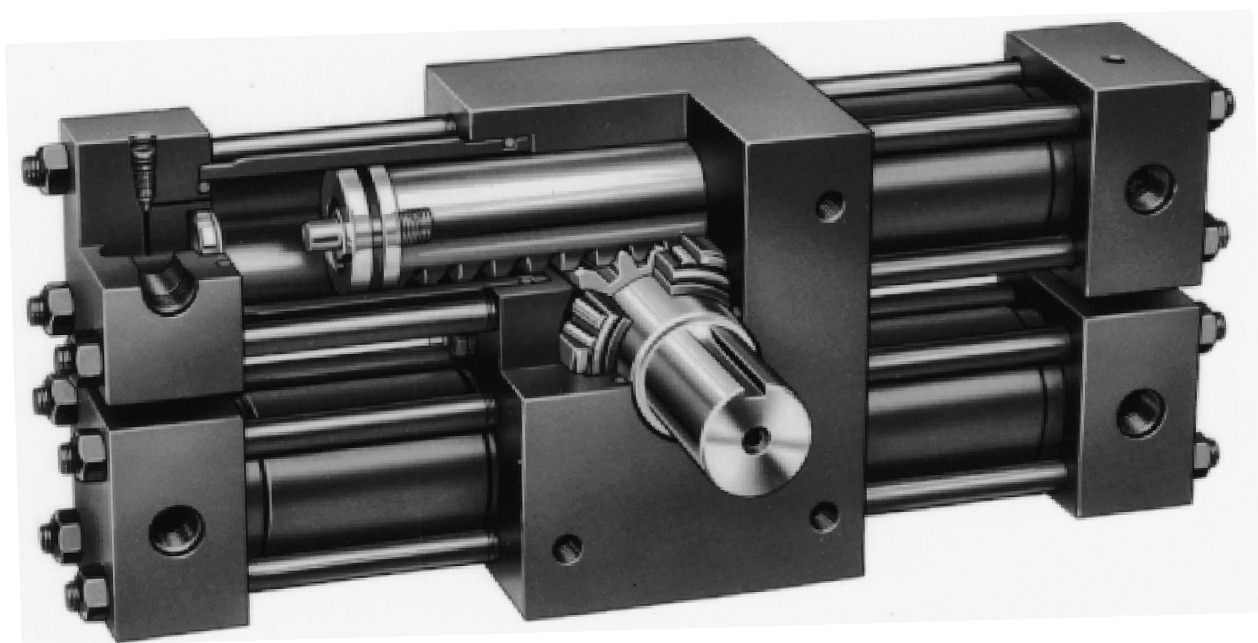
Figure 2 Rack and pinion type rotary actuator; double rack design
