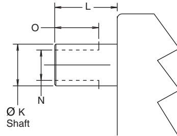
Metric Keyed Shaft
