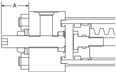
Type II Stroke Adjusters, 5°
