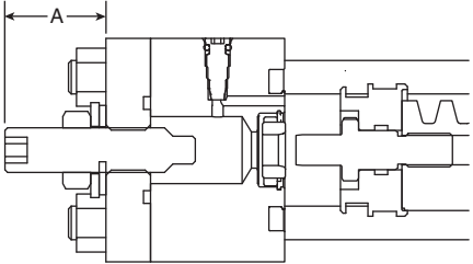
Type II Stroke Adjusters, 5°
