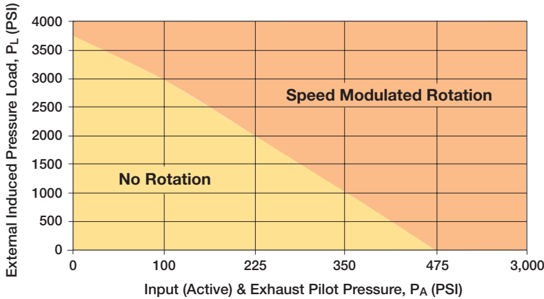
Movement of actuator with counter-balance valves
