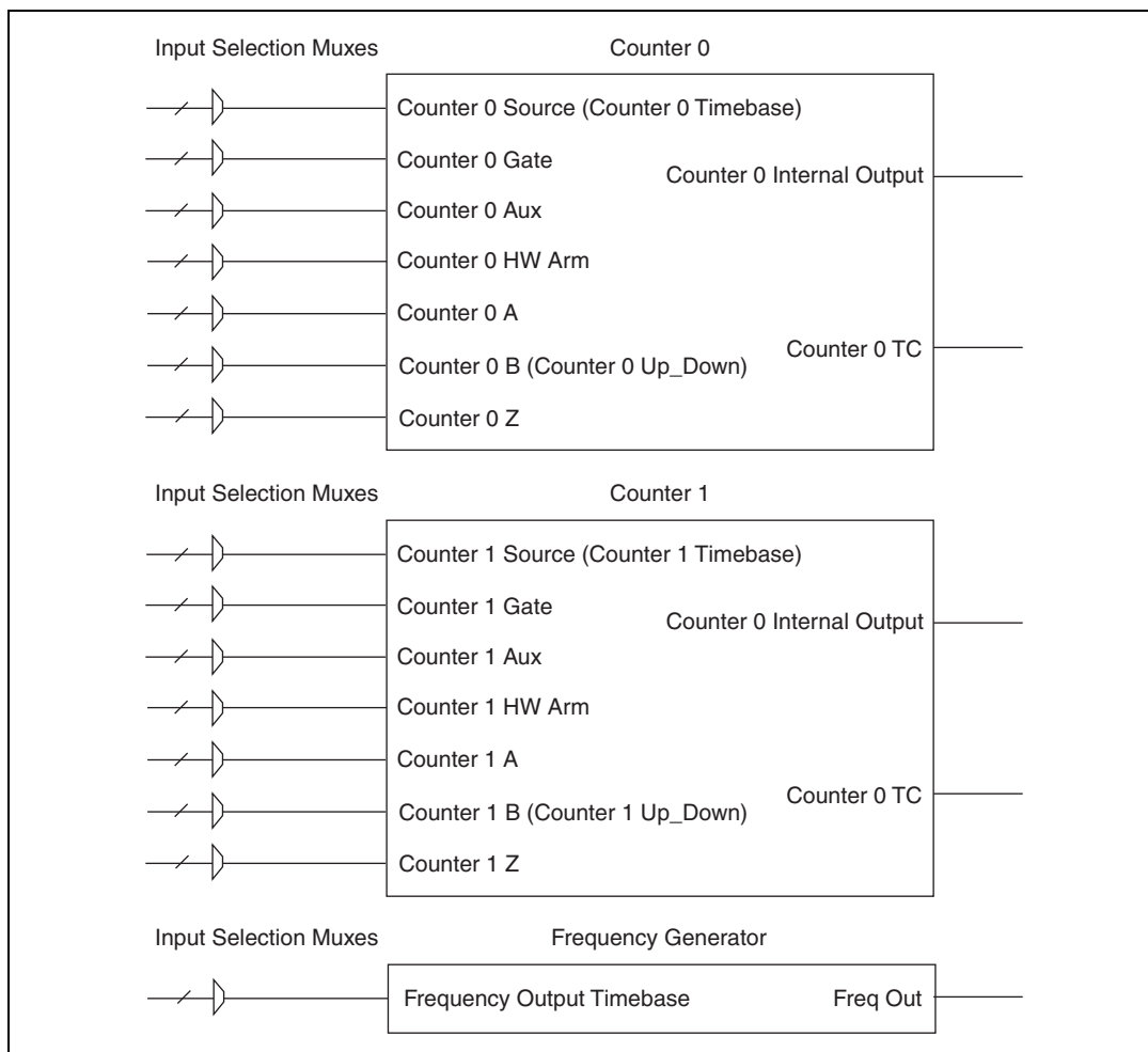
Figure 8-1. USB-621x Counters
