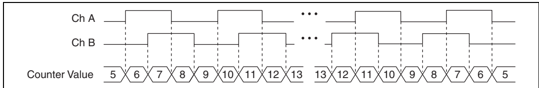
Figure 8-16. X4 Encoding
