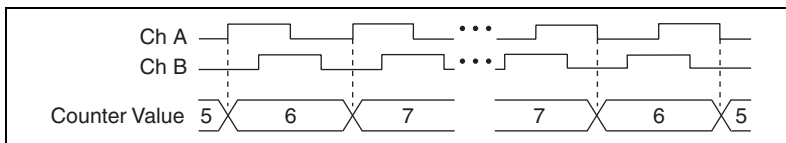
Figure 8-14. X1 Encoding
