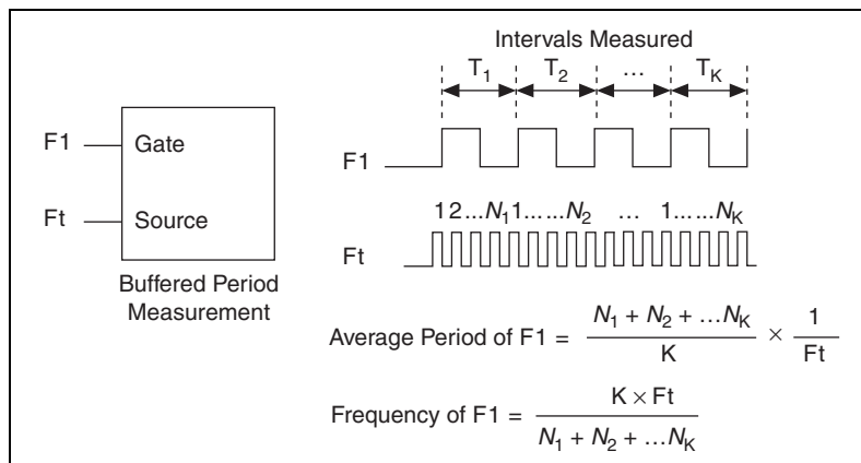
Figure 8-11. Method 1b
