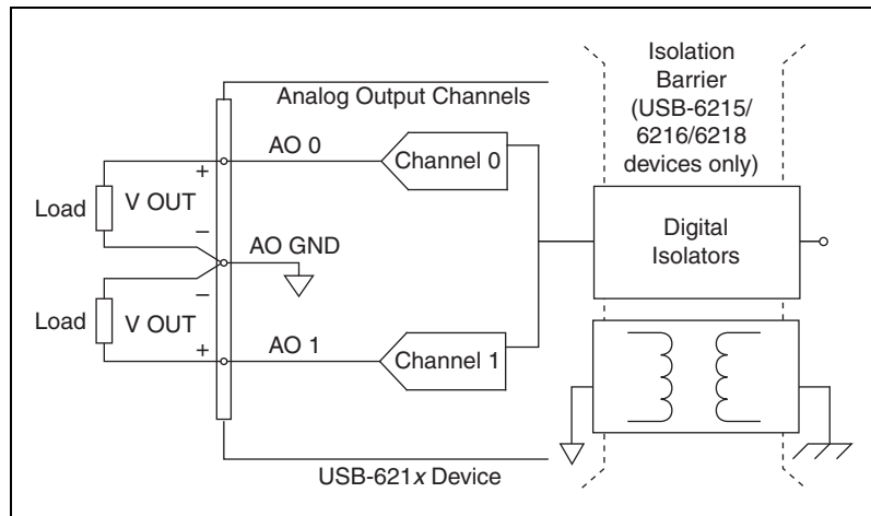
Figure 5-2. Analog Output Connections
