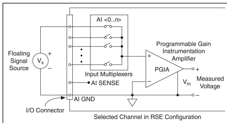
Figure 4-21. Referenced Single-Ended Connections for Floating Signal Sources
