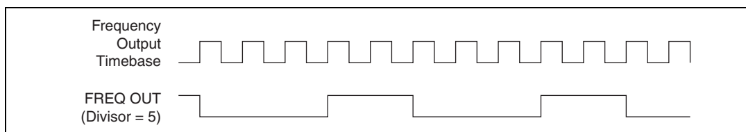
Figure 8-28. Frequency Generator Output Waveform
