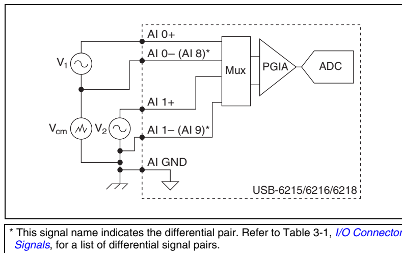
Figure 4-24. Connecting to the USB-6215/6216/6218 in Differential Mode
