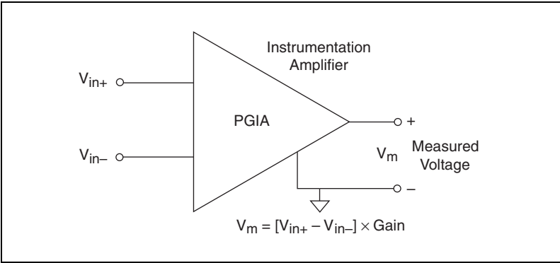
Figure 4-2. NI-PGIA
