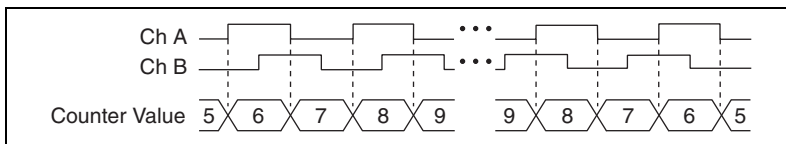
Figure 8-15. X2 Encoding
