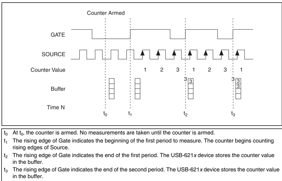
Figure 8-8. Buffered Period Measurement
