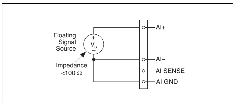
Figure 4-16. Differential Connections for Floating Signal Sources without Bias Resistors
