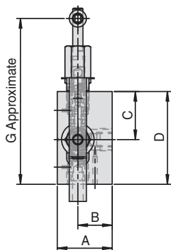
Dimensions in inches
