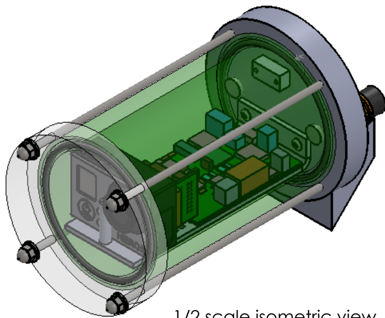
1/2 scale isometric view
