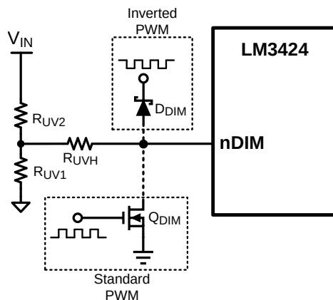
Figure 34. PWM Dimming Circuit
