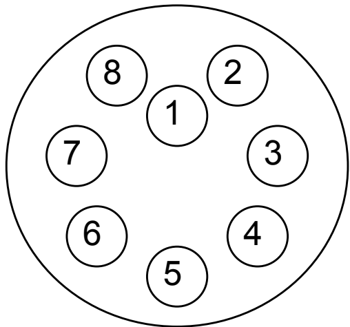
MCBHRA8MSS VIEWED FROM PIN SIDE
