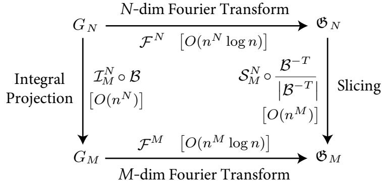
Figure 5.6: Generalized Fourier Slice Theorem (Equation 5.2). Transform relationships between an N -dimensional function G_N , an M -dimensional integral projection of it, G_M , and their respective Fourier spectra, \mathfrak{G}_N and \mathfrak{G}_M .
