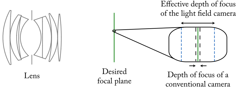
Figure 4.5: Improvement in effective depth of focus in the light field camera compared to a conventional camera. The range is 8 times wider in the light field camera, assuming that the directional resolution of the light field is 8 \times 8 .
