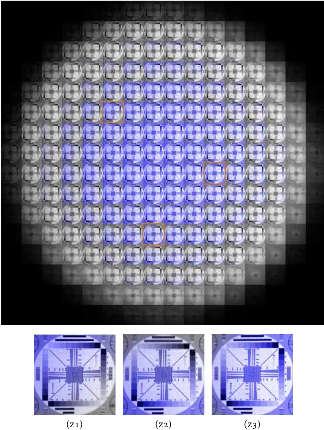
Figure 7.8: Weighting of rays (light field cells) in weighted correction. Each ray's weight is proportional to how blue it appears.
