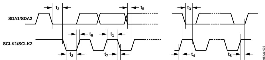
Figure 3. I²C Timing
