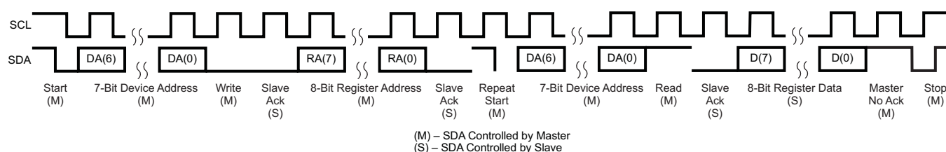
Figure 18. I²C Read
