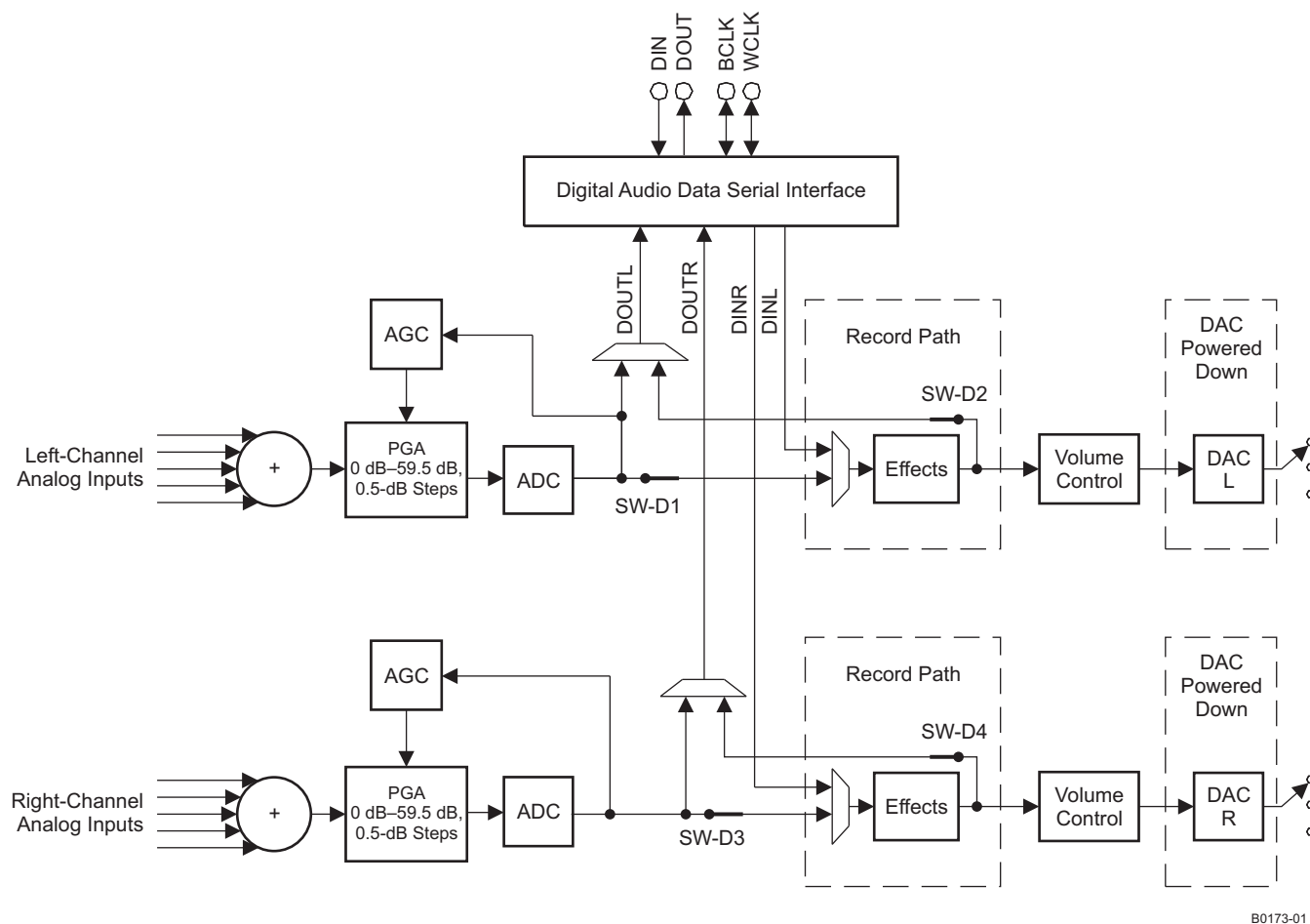
Figure 25. Record-Only Mode With Digital Processing Path Enabled
