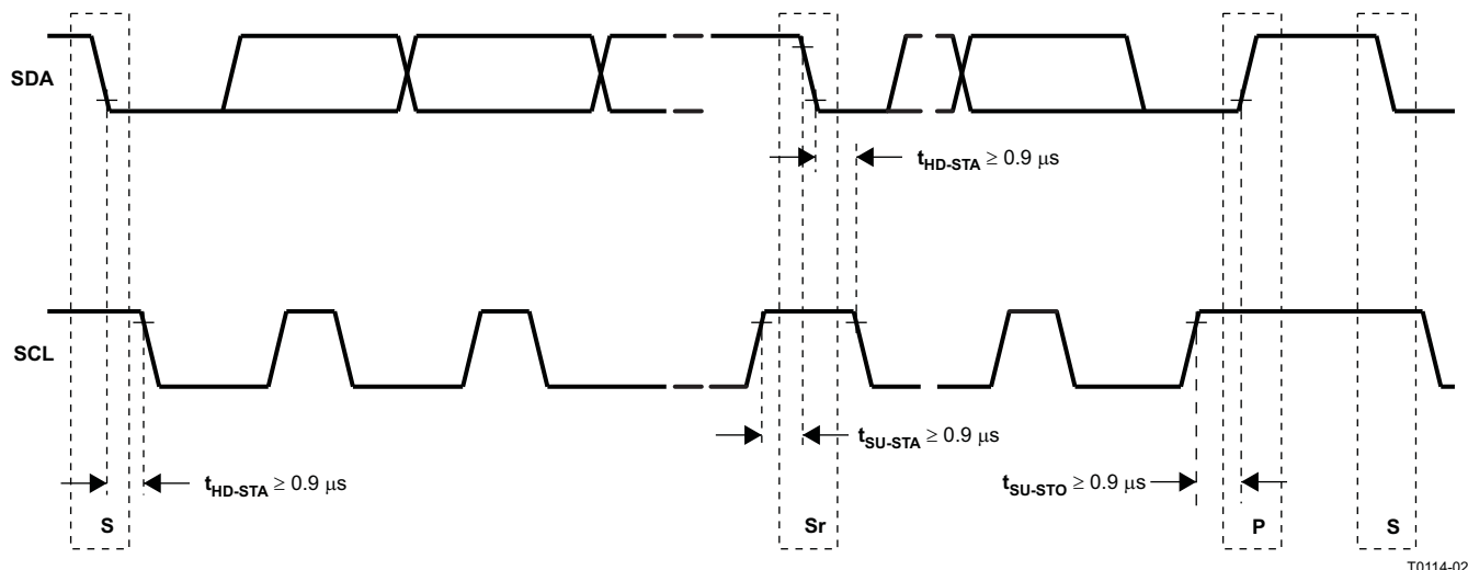
Figure 16. I²C Interface Timing
