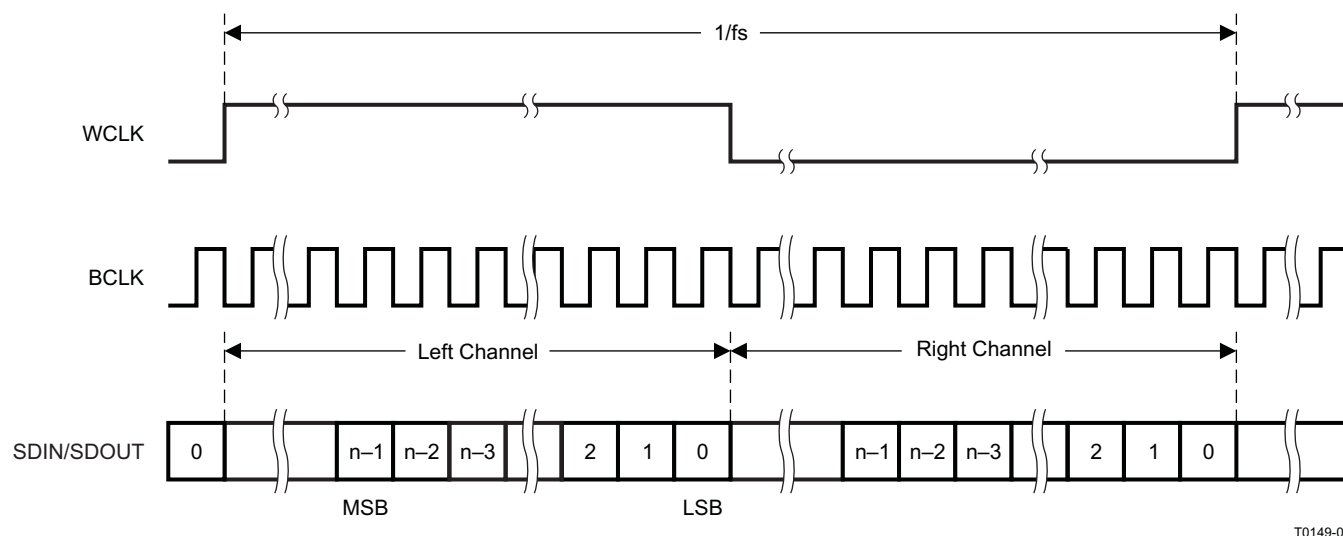
Figure 19. Right-Justified Serial Data Bus Mode Operation
