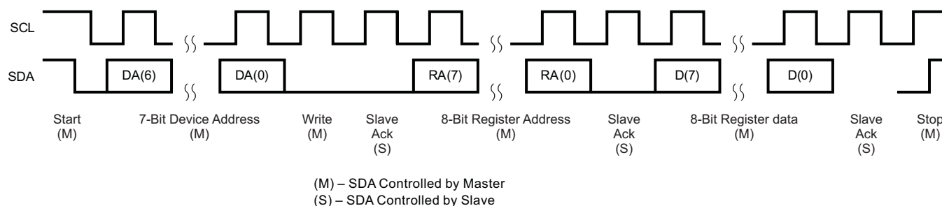
Figure 17. I²C Write
