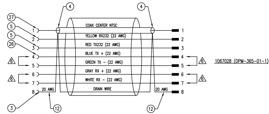
CIRCUIT DIAGRAM (FOR DOUBLE ENDED ASSEMBLY) □ = TWISTED PAIR
