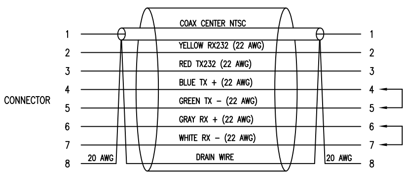
CIRCUIT DIAGRAM (FOR P/N 1067028 AND 1067029 AFTER PRESSURE TEST IS COMPLETE) □ = TWISTED PAIR
