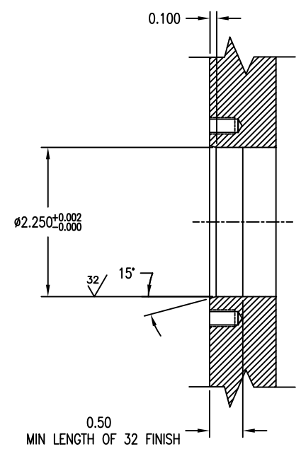
BULKHEAD PLUG MOUNTING DETAIL (1:2 SCALE)
