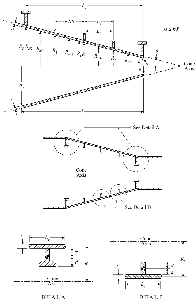
FIGURE 5 Definitions – Cones
