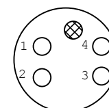
MCIL4F Female Face View
