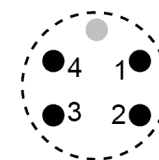
wet-pluggable connector: MCBH-4MP (WB), TI (3/8" length base, 1/2-20 thread)
