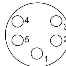
MCIL5F Female Face View
