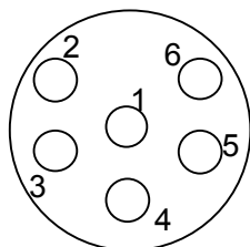
MCIL6FS Female Face View
