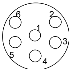
MCBH6MP Male Face View
