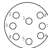
MCIL8F Female Face View
