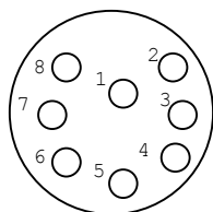
MCIL8M Male Face View
