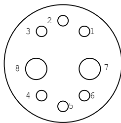
MINK8 CCPL cable connector face view
