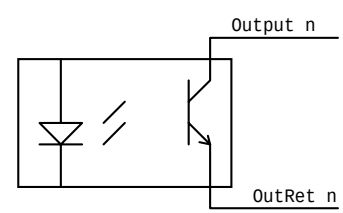
Digital Output Internal Circuit
