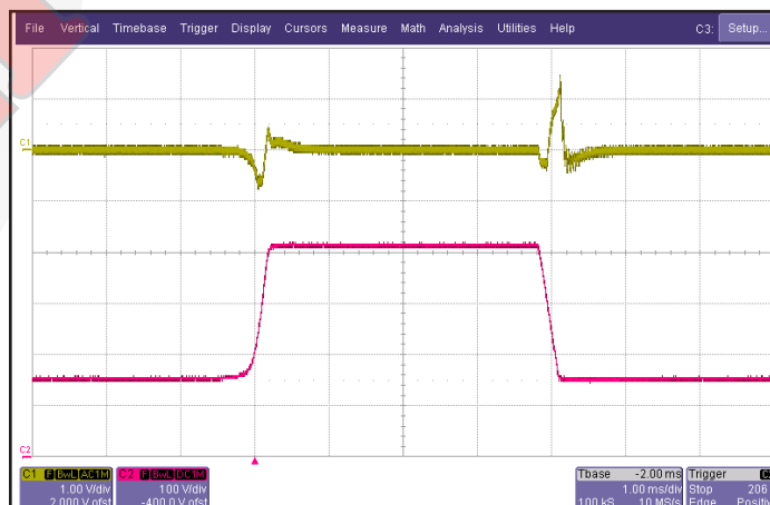
Figure 12: Output voltage response to step-change in input voltage (155V - 425V - 155V) with 250 \mu\text{s} rise / fall time. Load cap: 1 \mu\text{F} ceramic and 15 \mu\text{F} tantalum capacitors. Ch 1: V_{out} (1V/div), Ch 2: V_{in} (100V/div).
