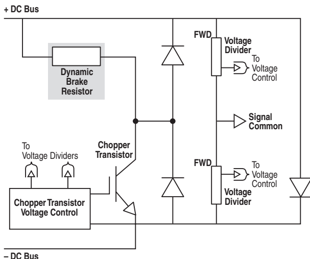
Figure 1.1 Simplified Dynamic Brake Schematic
