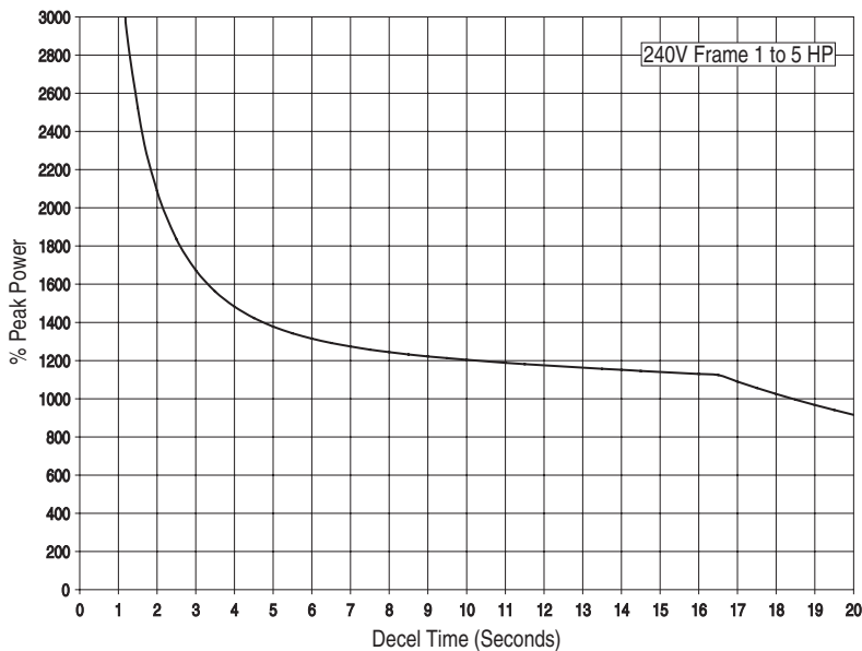
Figure 3.10 PowerFlex 700 – 240 Volt, Frame 1 to 5 HP
