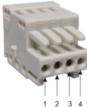
4-Pin WAGO Connector (733-104)
