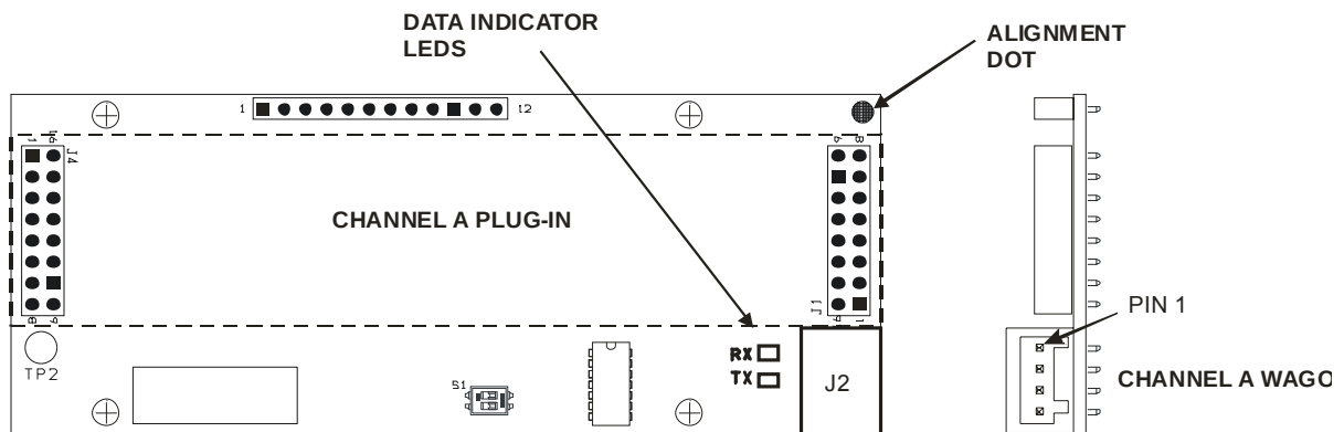
Figure 2-4: 914-AIB Adapter Card
