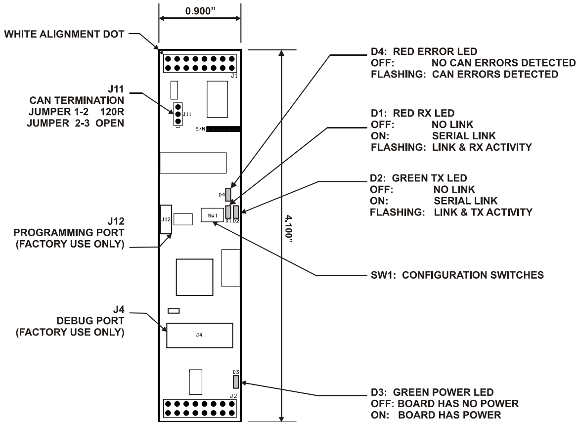
Figure 4-7: AIB-CANBUS Plug-In Module (Top View)
