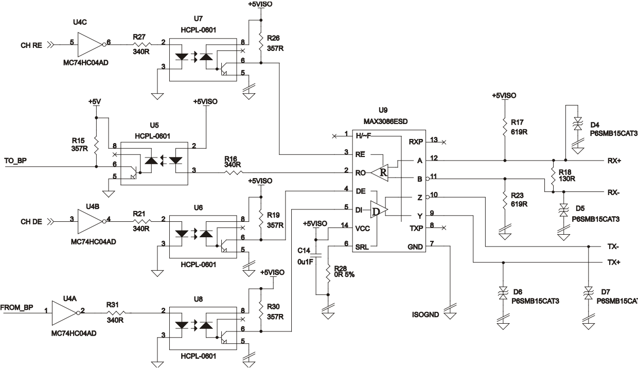
Figure 4-3: AIB RS-422 Interface Schematic
