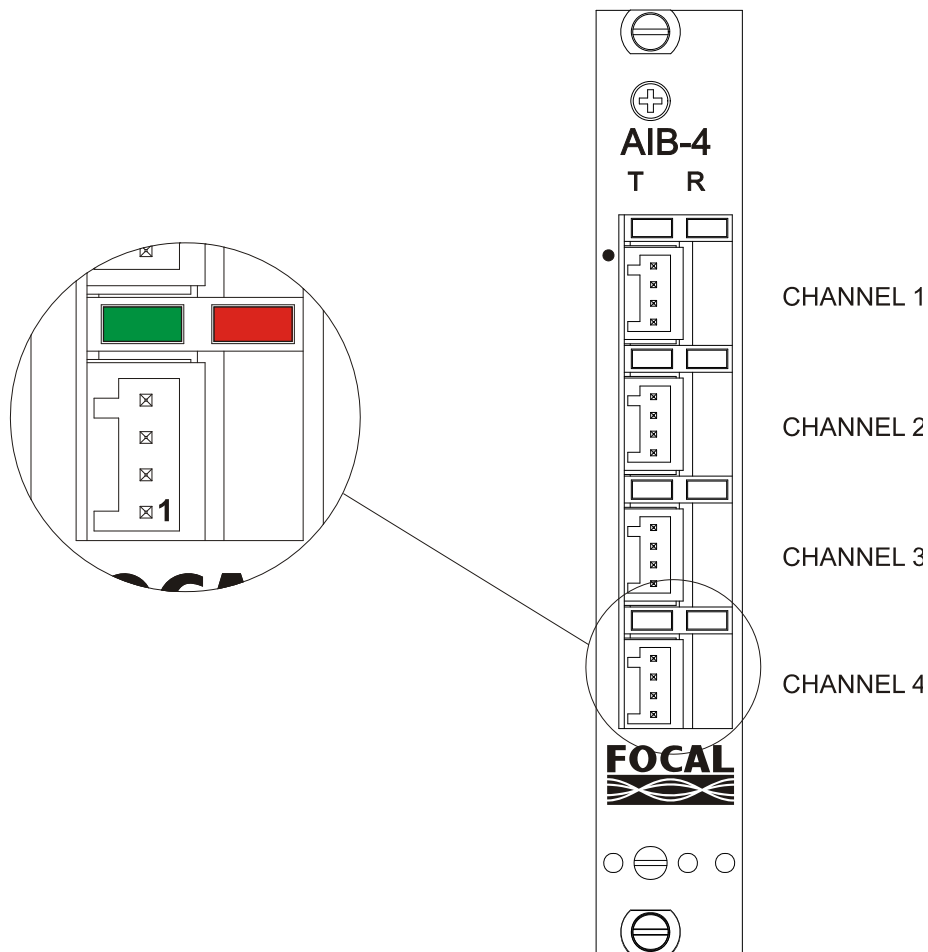
Figure 2-1: Model 903 AIB-4 Front Panel
