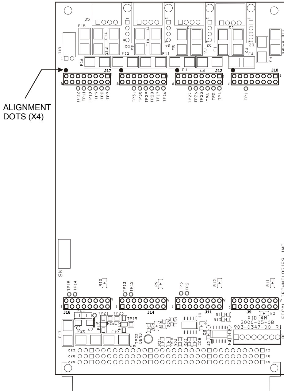
Figure 2-2: Model 903 AIB-4 Motherboard (AIB-4M)
