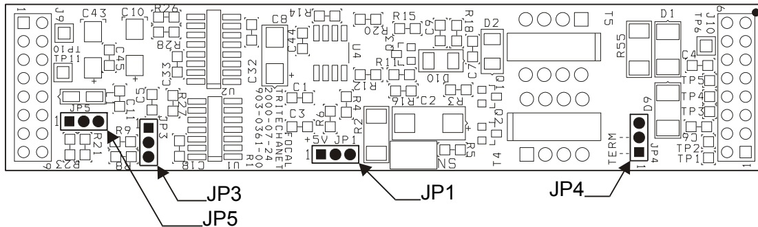
Figure 4-4: AIB Trittech ARCNET Plug-In Module
