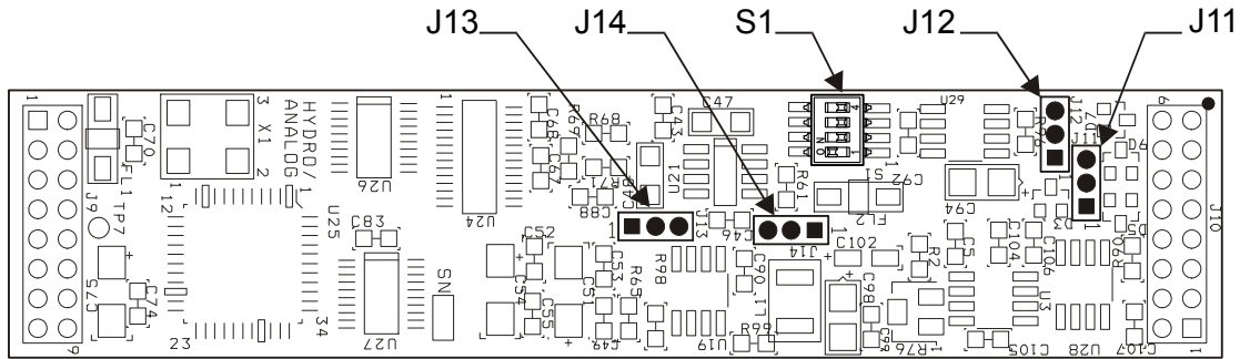
Figure 4-5: AIB Hydrophone Plug-In Module
