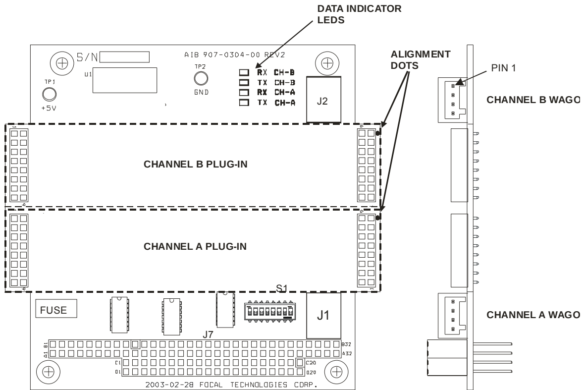
Figure 2-3: 907-AIB Adapter Card
