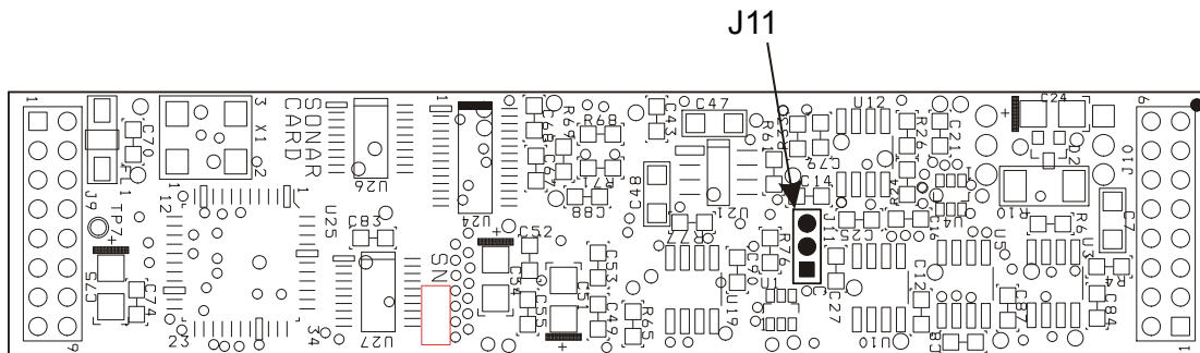
Figure 4-6: AIB MS-900 Plug-In Module (Top View)
