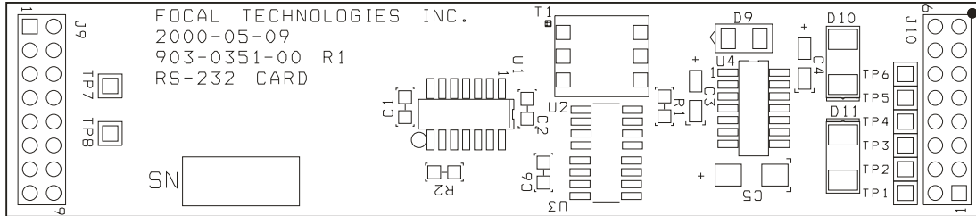
Figure 4-1: AIB RS-232 Plug-In Module
