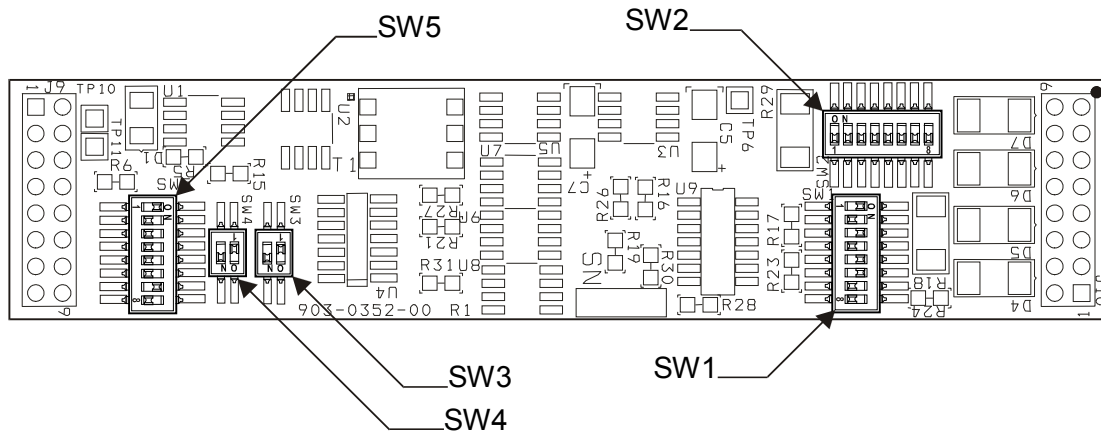
Figure 4-2: AIB RS-485 Plug-In Module
