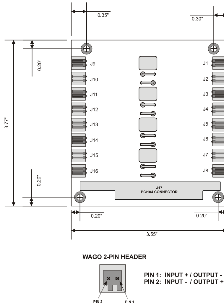
Figure 5-8: 907-AUDIO-T Expansion Card
