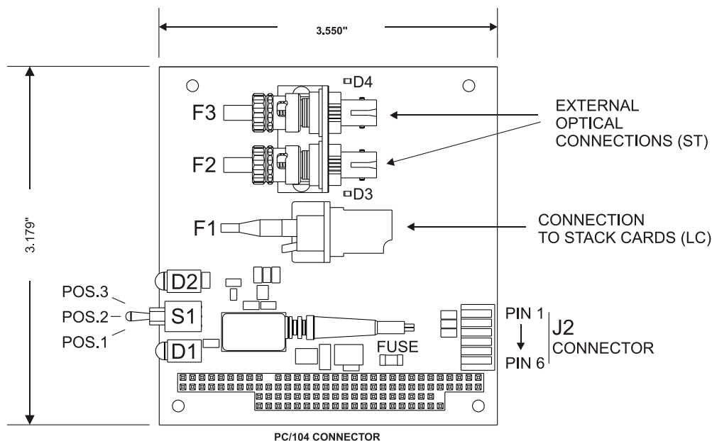
Figure 6-8: 907-FOS, 1x2 Fiber Optic Switch Card
