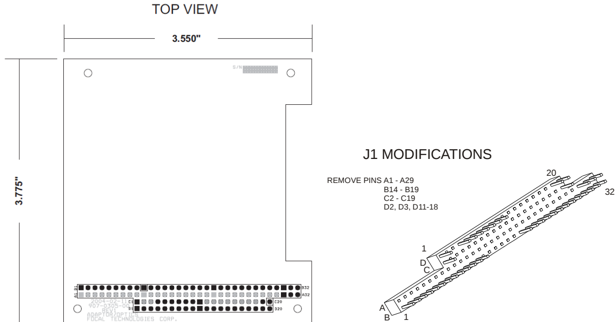
Figure 6-3: 907-PC104, 907 to Standard PC/104 Adaptor
