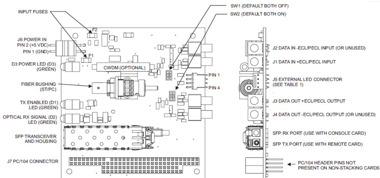
Figure 4-4: 907-ECL Media Converter Card
