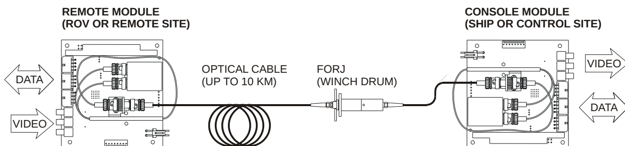
Figure 2-1: Example of a Model 907 Multiplexer System
