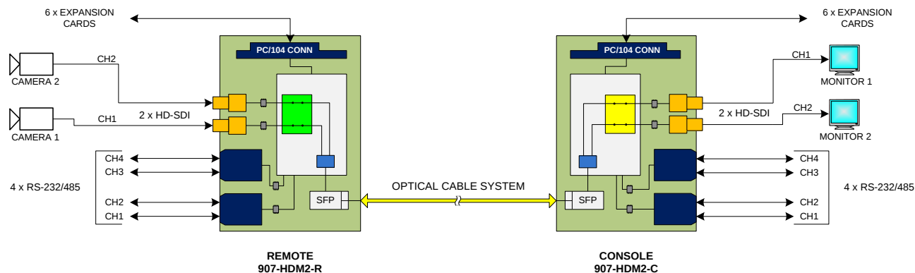
Figure 3-13: On board I/O Channels for 907-HDM2-R and 907-HDM2-C Multiplexer Motherboard Cards (Dual Video Channel – Optimized Sampling)
