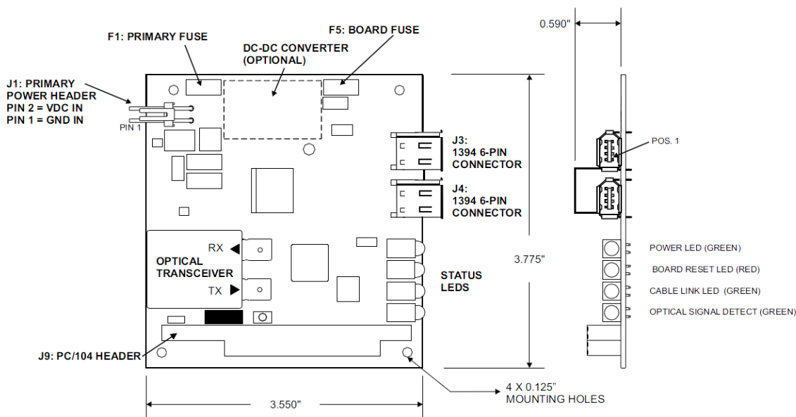
Figure 4-3: 907-1394 Media Converter Card
