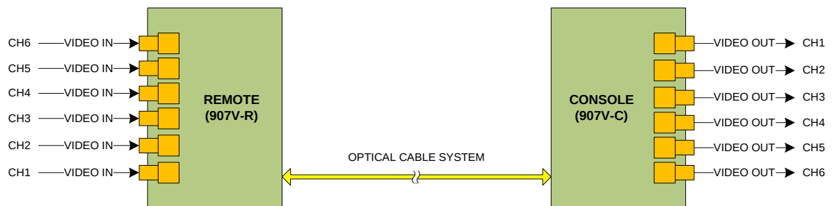
Figure 3-6: On board I/O Channels for 907V-R and 907V-C Multiplexer Motherboard Cards
