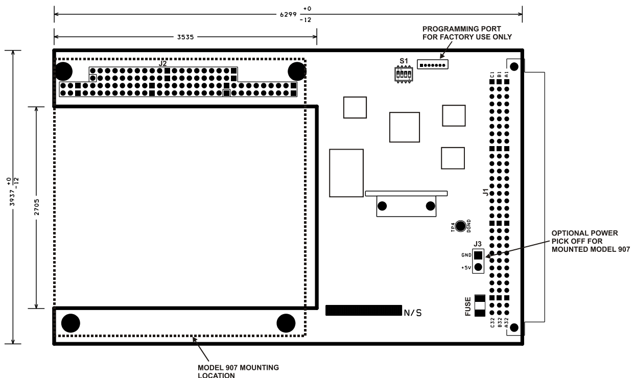
Figure 6-1: 907-EURO Eurocard Adaptor
