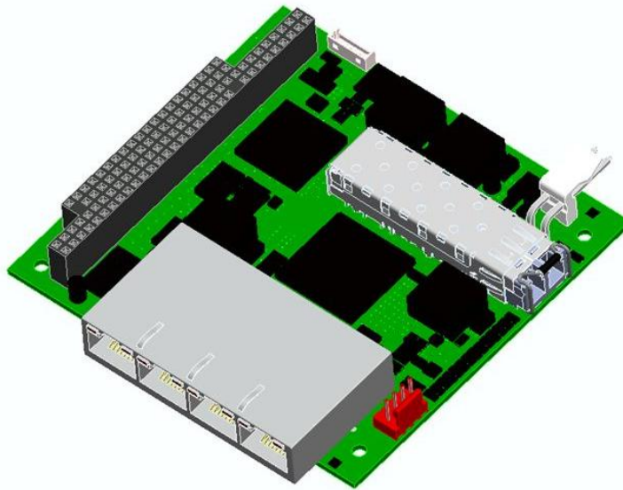
Figure 3-17: Model 907-GEM Multiplexer Motherboard
