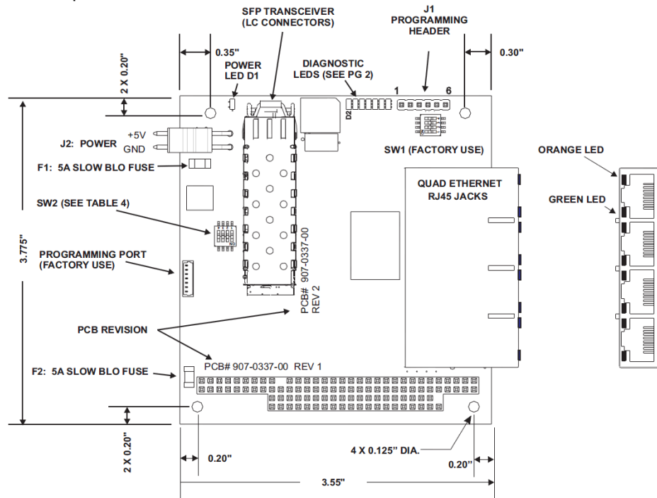
Figure 4-8: 907-GBES Media Converter Card
