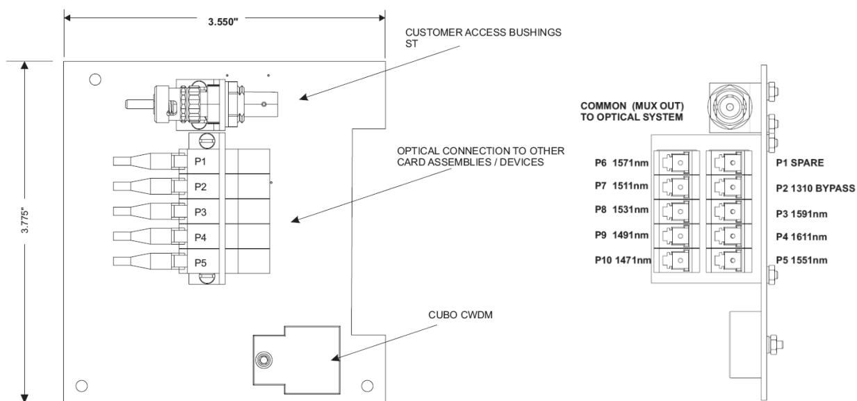
Figure 6-7: 907-CWDM-8, 8-Channel CWDM Optics Card
