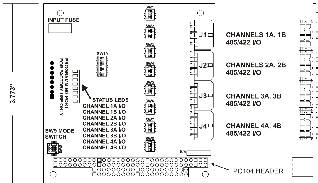
Figure 5-3: 907-485, RS-485/422 Expansion Card
