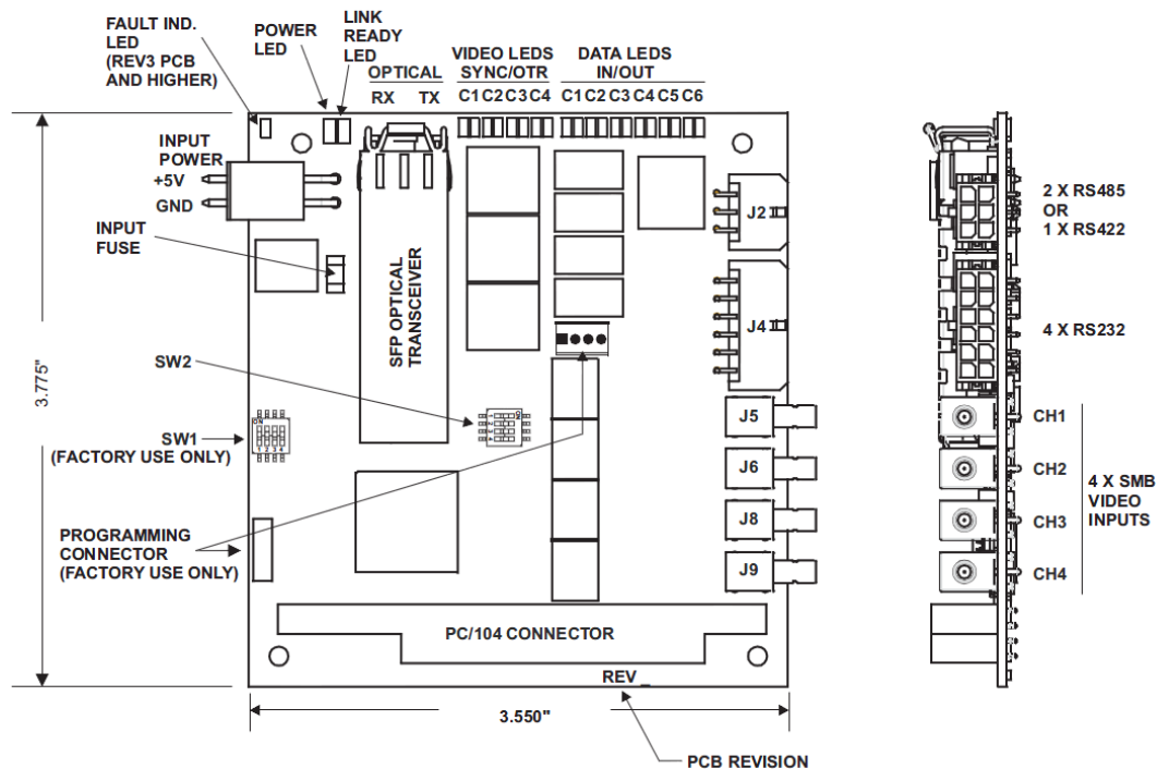
Figure 3-10: 907+R Multiplexer Card
