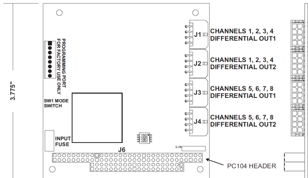
Figure 5-6: 907-DAC Expansion Card
