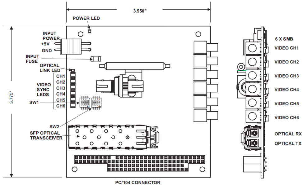
Figure 3-7: 907V-R & 907V-C Multiplexer Card
