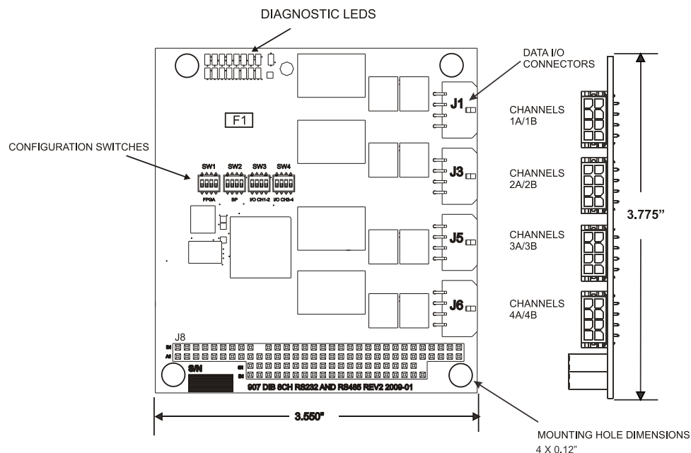
Figure 5-4: 907-SER, Serial Data Expansion Card
