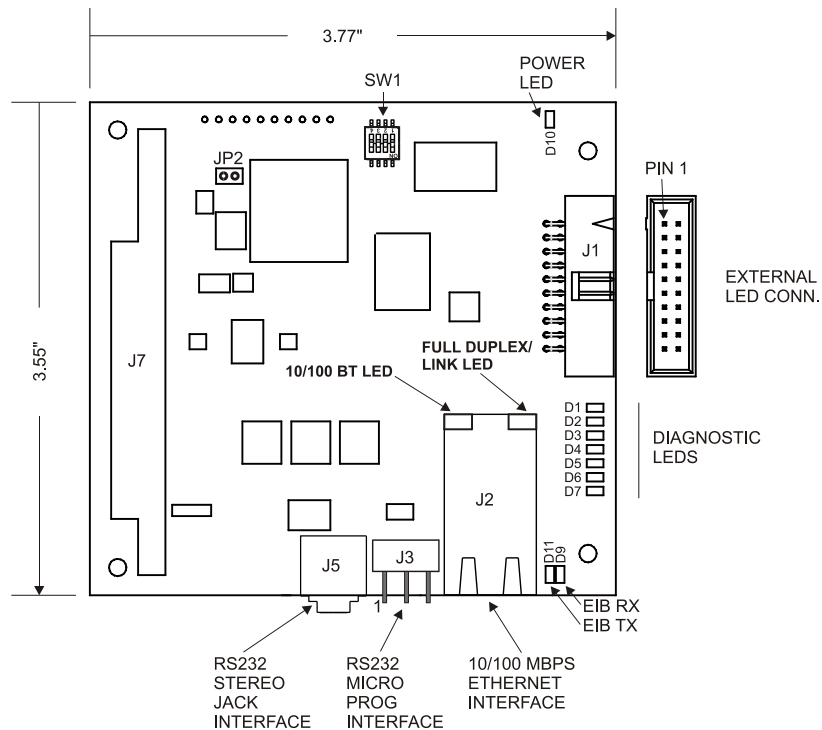
Figure 6-11: 907-DIAG-E Diagnostics Card
