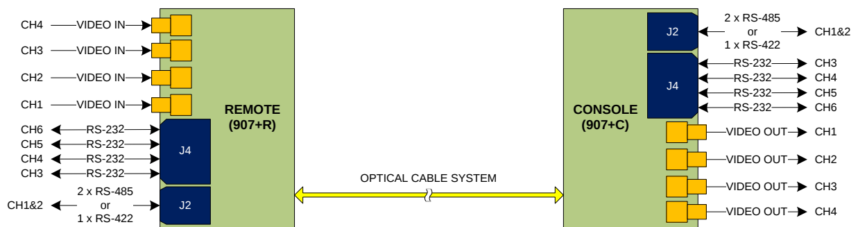
Figure 3-9: On board I/O Channels for 907+R and 907+C Multiplexer Motherboard Cards
