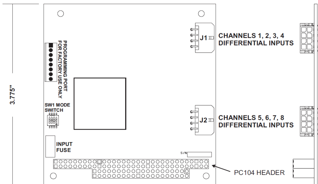
Figure 5-5: 907-ADC Expansion Card
