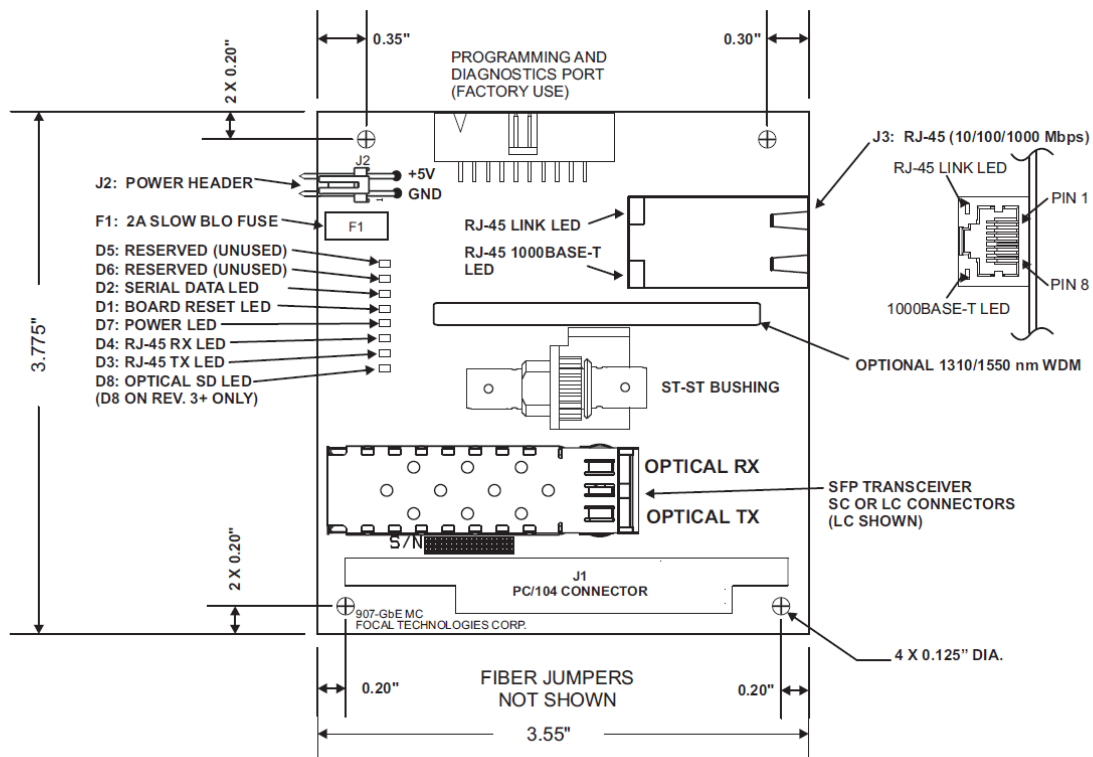
Figure 4-6: 907-GBE Media Converter Card
