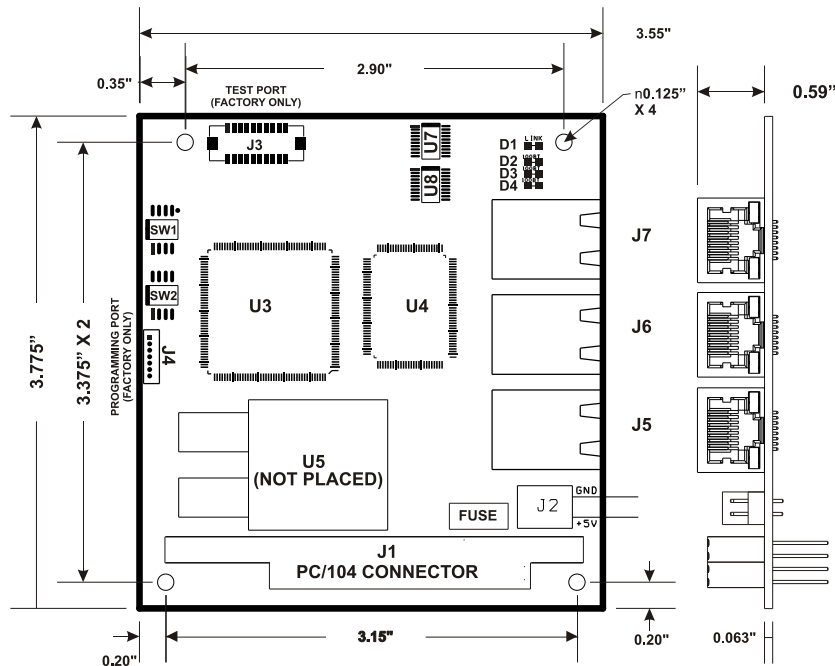
Figure 5-1: 907-EIBS Ethernet Expansion Card
