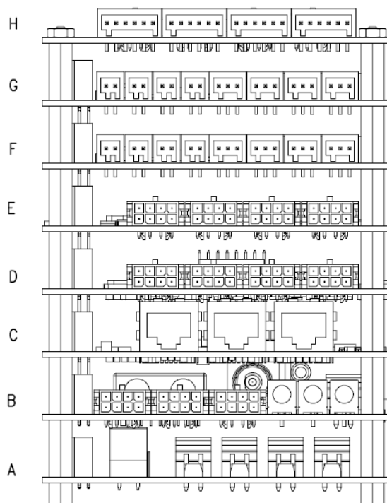
Figure 8-1: Example Model 907 Remote Stack View
