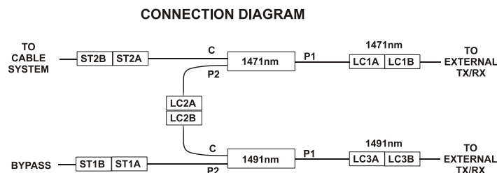
Figure 6-5: 907-CWDM Optics Card
