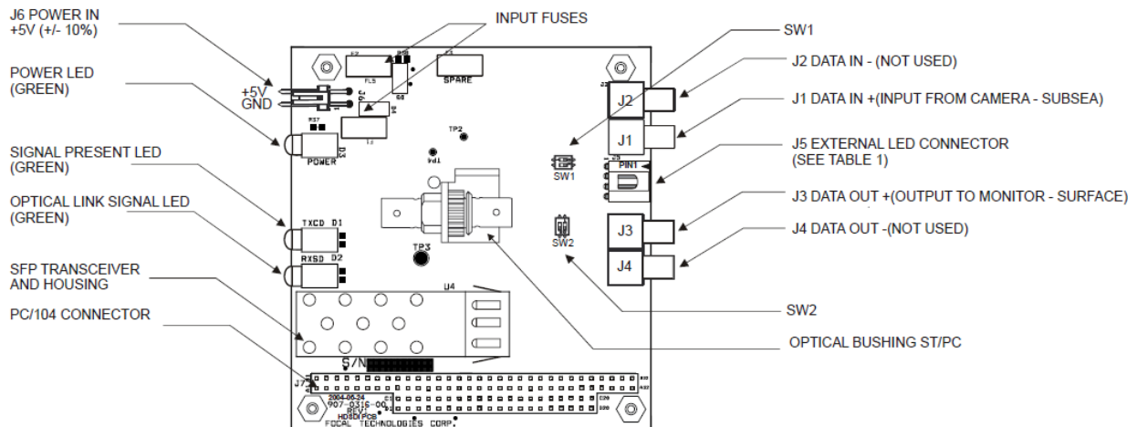
Figure 4-5: 907-HDV (HD-SDI) Media Converter card
