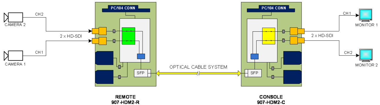
Figure 3-14: On board I/O Channels for 907-HDM2-R and 907-HDM2-C Multiplexer Motherboard Cards (Dual Video Channel – Full Sampling)
