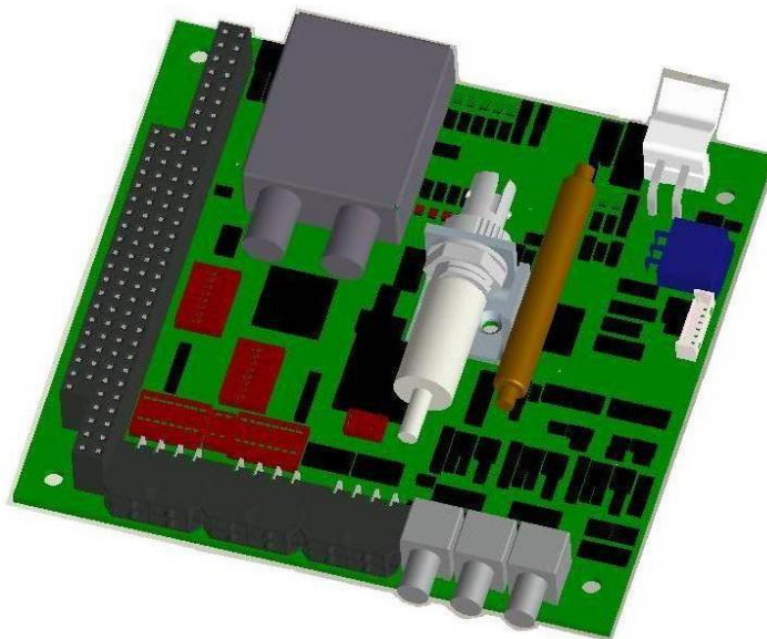
Figure 3-2: Standard Model 907 Multiplexer Motherboard with WDM
