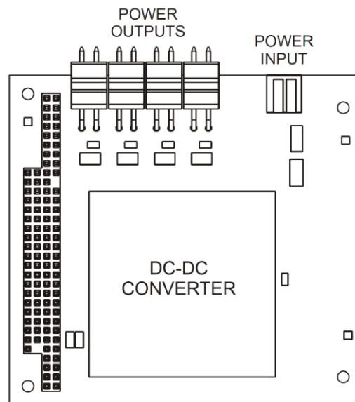
Figure 6-4: 907-DC-24 Power Distribution Card
