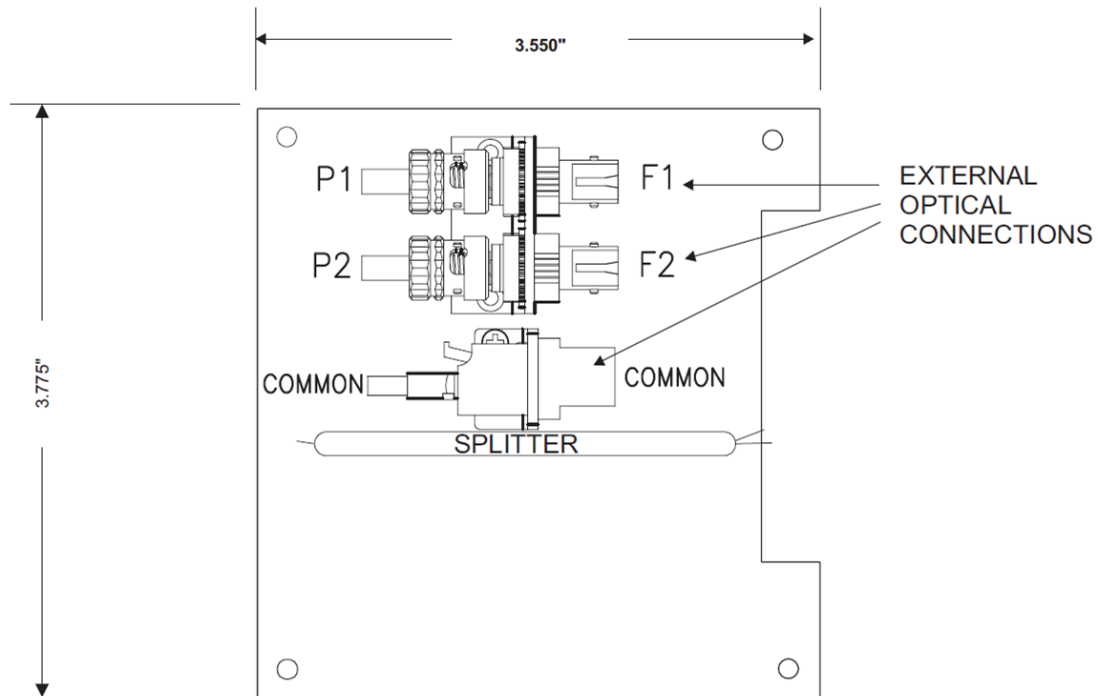
Figure 6-9: 907-SPLIT, 1x2 Optical Splitter Card
