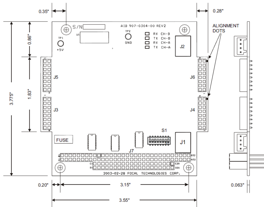
Figure 5-13: 907-AIB, Adaptable Interface Board Adaptor
