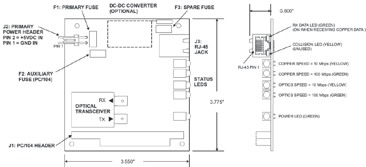
Figure 4-2: 907-MC (10/100 Ethernet) Card without WDM
