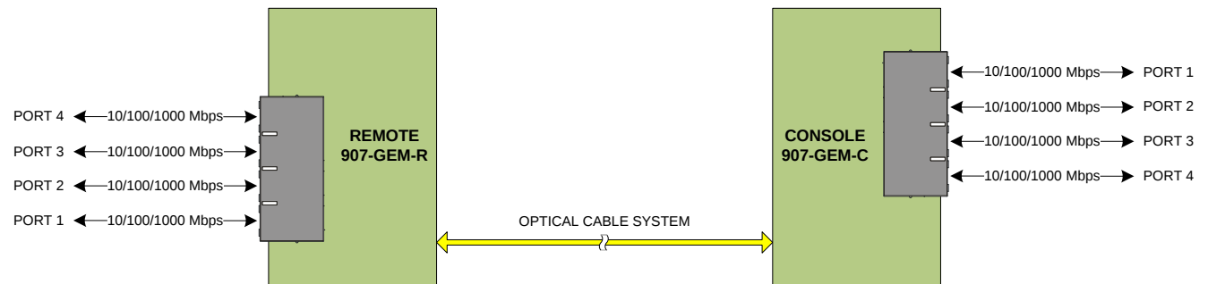
Figure 3-18: On board I/O Channels for 907-GEM-R and 907-GEM-C Multiplexer Motherboard Cards
