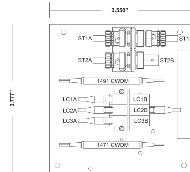
Figure 6-5: 907-CWDM Optics Card
