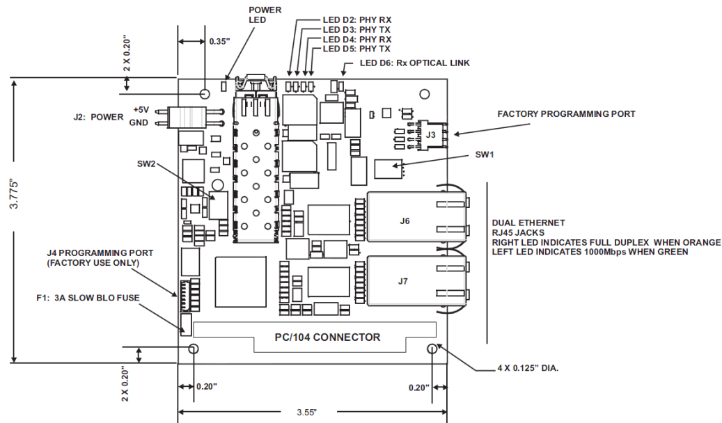
Figure 4-7: 907-GBE2, Dual Gigabit Ethernet Media Converter Card
