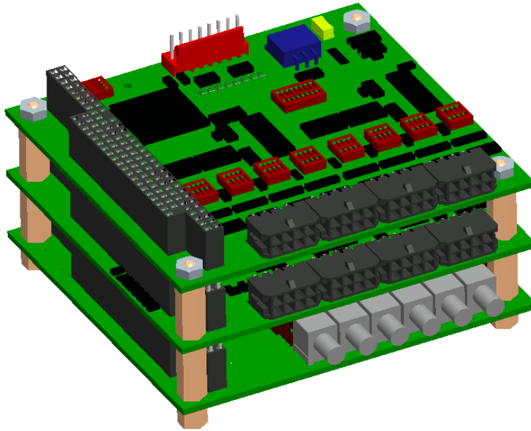
Figure 2-2: Example of a Model 907 Stack
