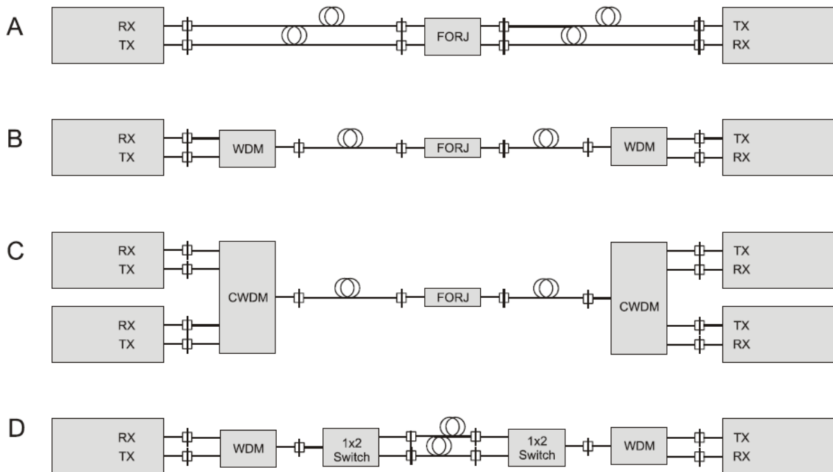
Figure 7-1: Example Optical Configurations
