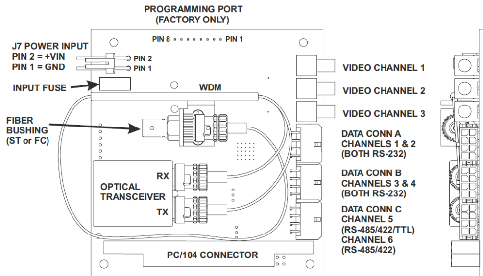
Figure 3-4: 907-R & 907-C Multiplexer Card
