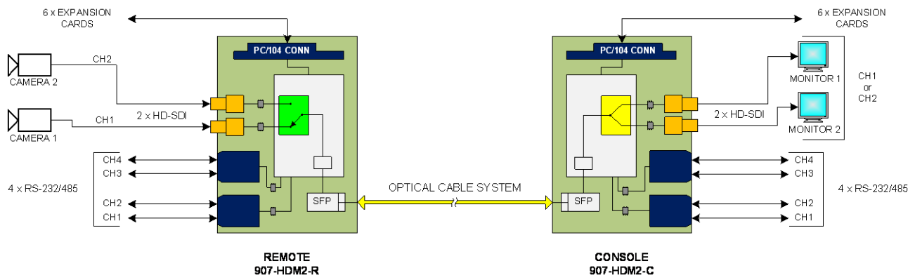
Figure 3-15: On board I/O Channels for 907-HDM2-R and 907-HDM2-C Multiplexer Motherboard Cards (Single Video Channel – Full Sampling, Switched Dual Input)
