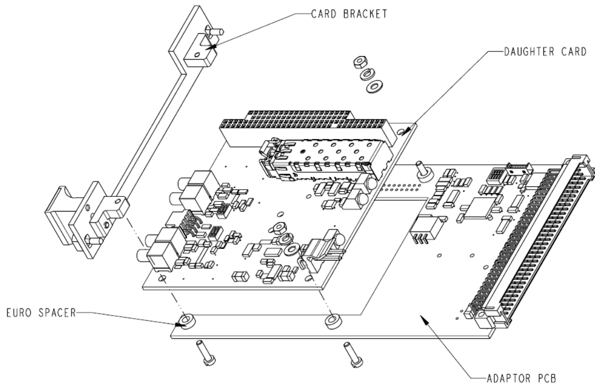
Figure 6-2: 907-EURO Eurocard Adaptor Card Assembly
