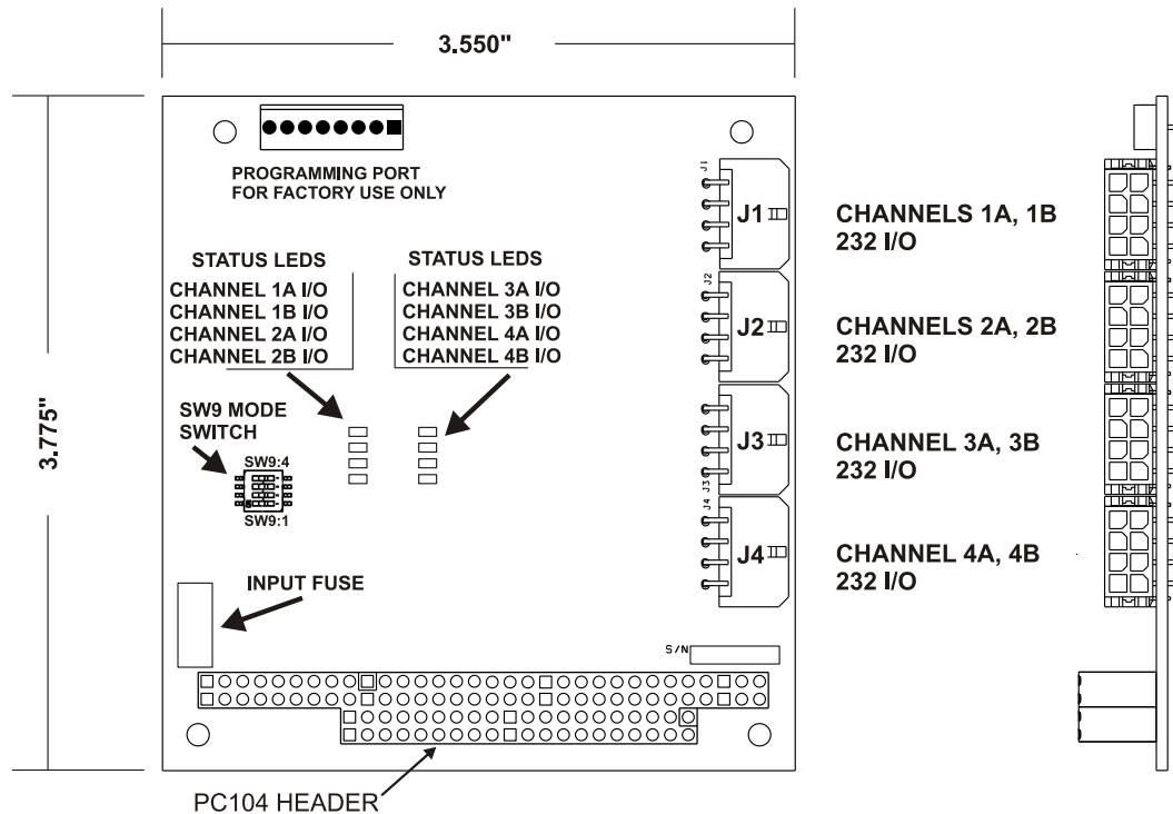
Figure 5-2: 907-232, RS-232 Expansion Card
