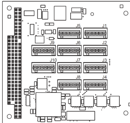
Figure 6-10: 907-DIAG LED Diagnostics Interface Card
