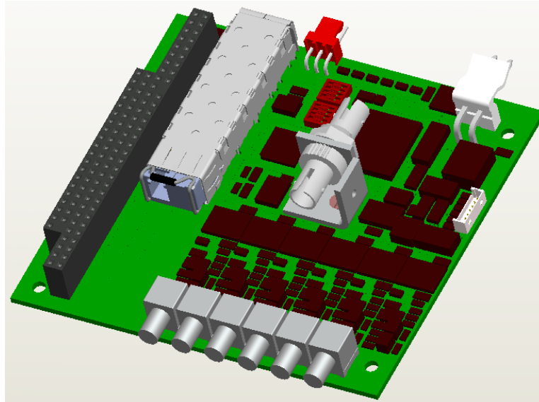
Figure 3-5: Model 907V Multiplexer Motherboard
