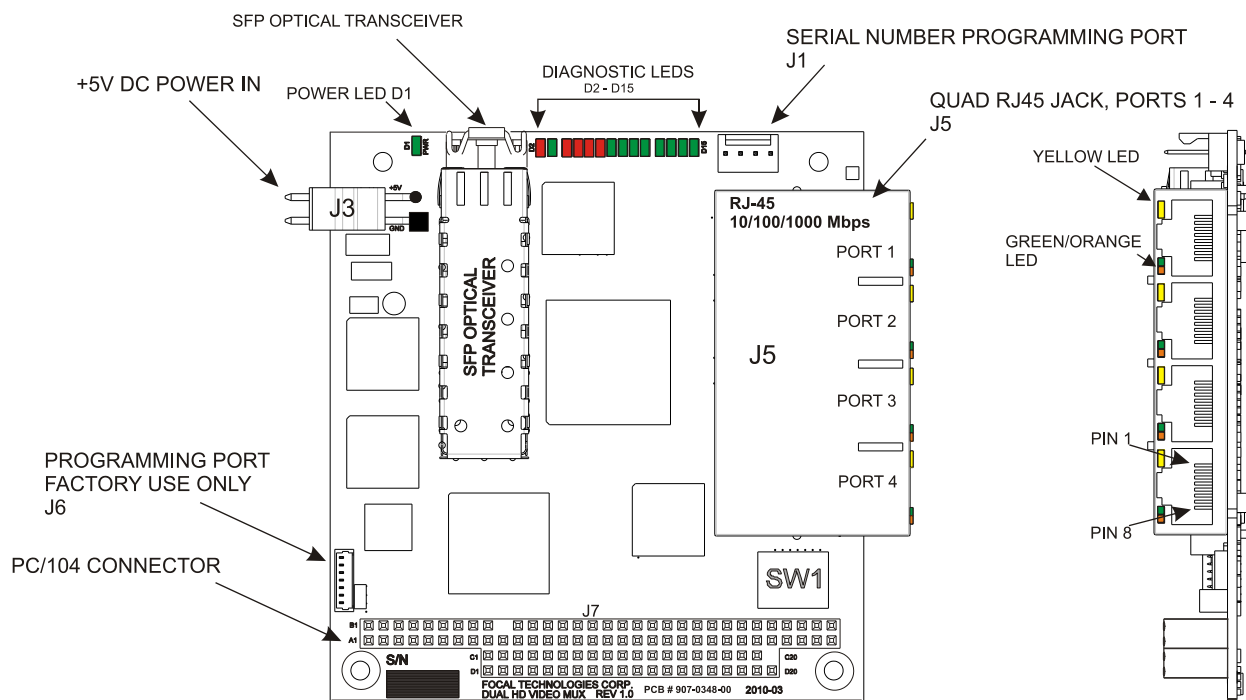
Figure 3-19: 907-GEM-R & 907-GEM-C Multiplexer Card
