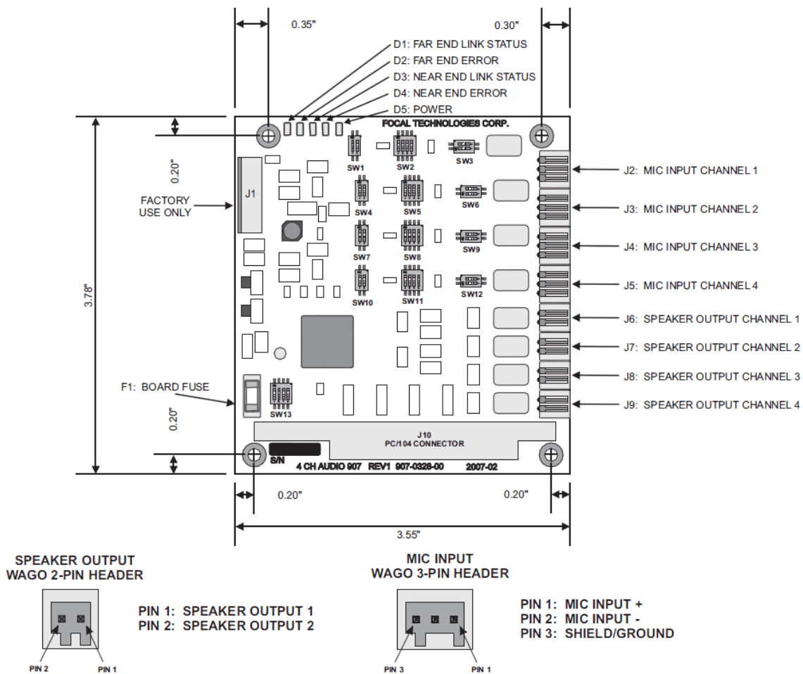
Figure 5-7: 907-AUDIO Expansion Card
