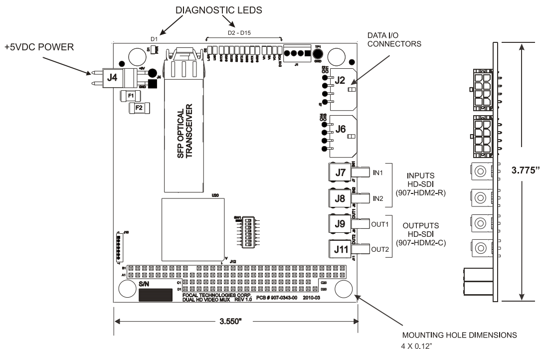
Figure 3-16: 907-HDM2-R & 907-HDM2-C Multiplexer Card
