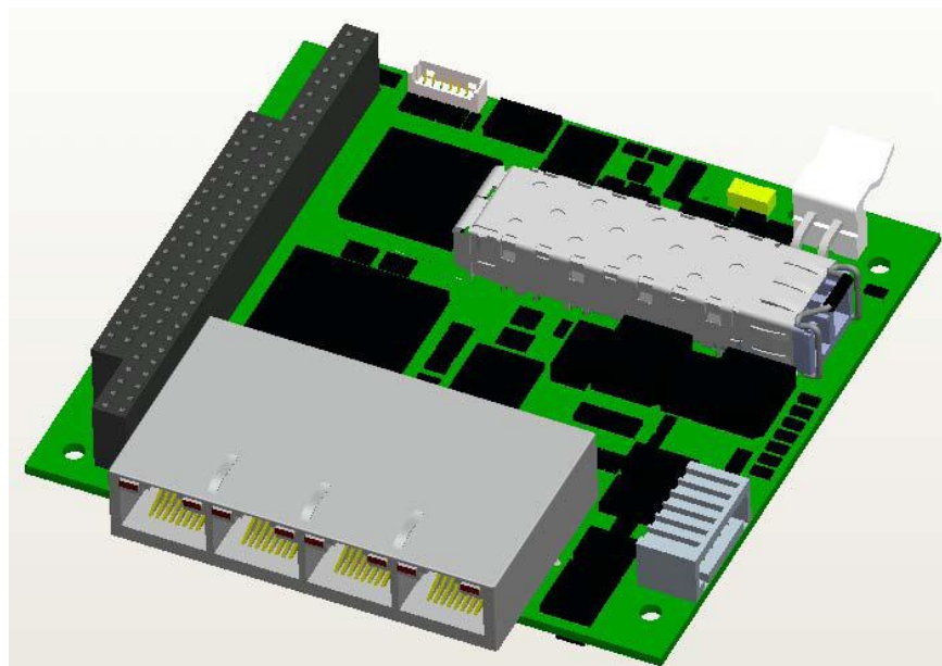
Figure 4-1: Media Converter Card (907-GBES)
