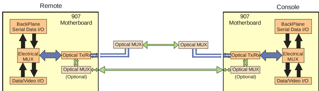
Figure 3-1: Remote & Console Motherboard Optical Configuration
