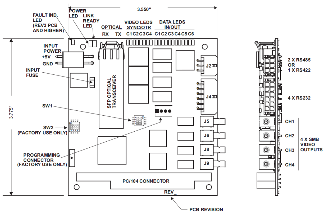
Figure 3-11: 907+C Multiplexer Card
