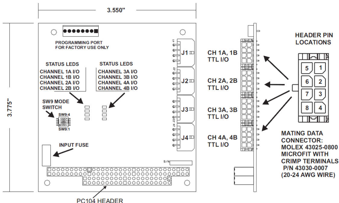
Figure 5-9: 907-TTL Expansion Card
