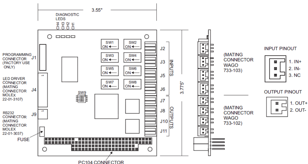
Figure 5-10: 907-CIB Control Channel Expansion Card
