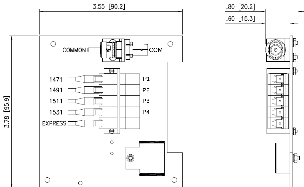
Figure 6-6: 907-CWDM-4, 4-Channel CWDM Optics Card
