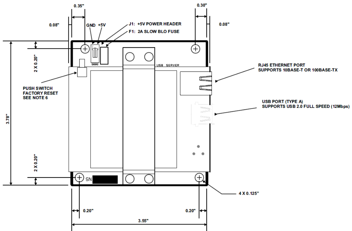
Figure 5-12: 907-USB Expansion Card
