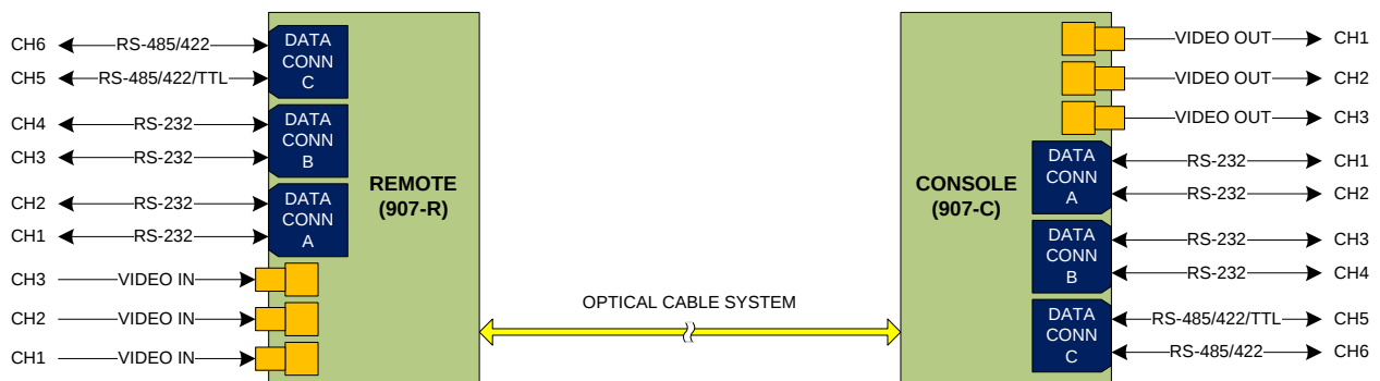
Figure 3-3: On board I/O Channels for 907-R and 907-C Multiplexer Motherboard Cards
