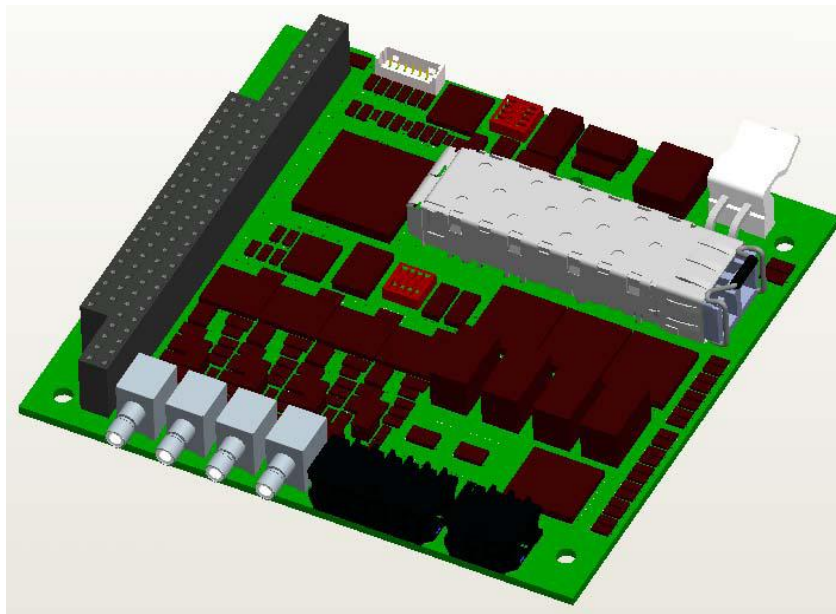
Figure 3-8: Model 907Plus Multiplexer Motherboard
