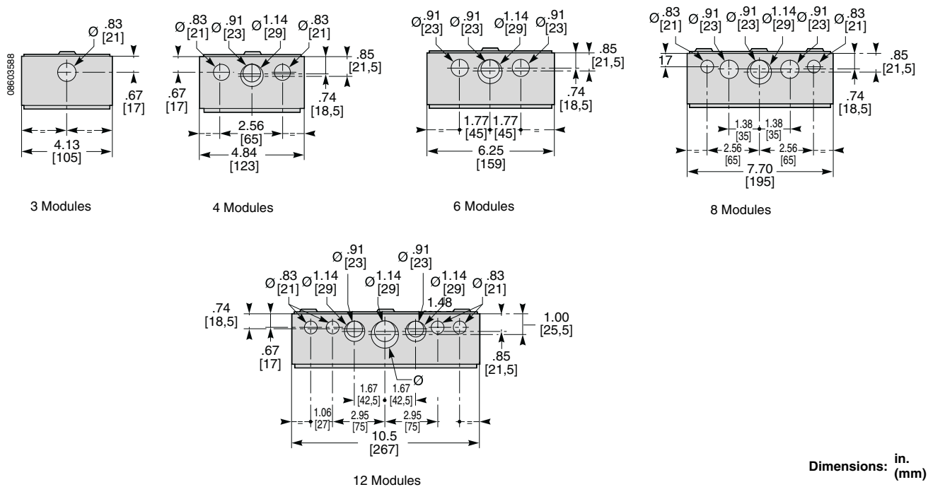
Figure 59: Top View for Kaedra™ Weatherproof Type Mini Enclosures
