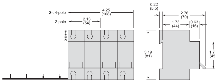
Figure 33: IEC Vigı Ground-Fault Module for C120 Devices
