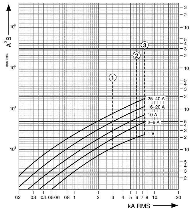
Figure 92: IEC Rated DPN-N (230/240 Vac) Maximum Let-Through I²t Current
