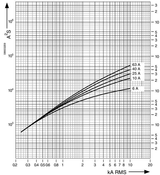
Figure 88: UL 1077 Recognized C60 2P, 3P, and 4P (480Y/277 Vac) Maximum Let-Through I 2 t Current
