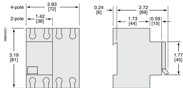
Figure 31: UL GFP Ground-Fault Protector and IEC ID Residual Current Switch
