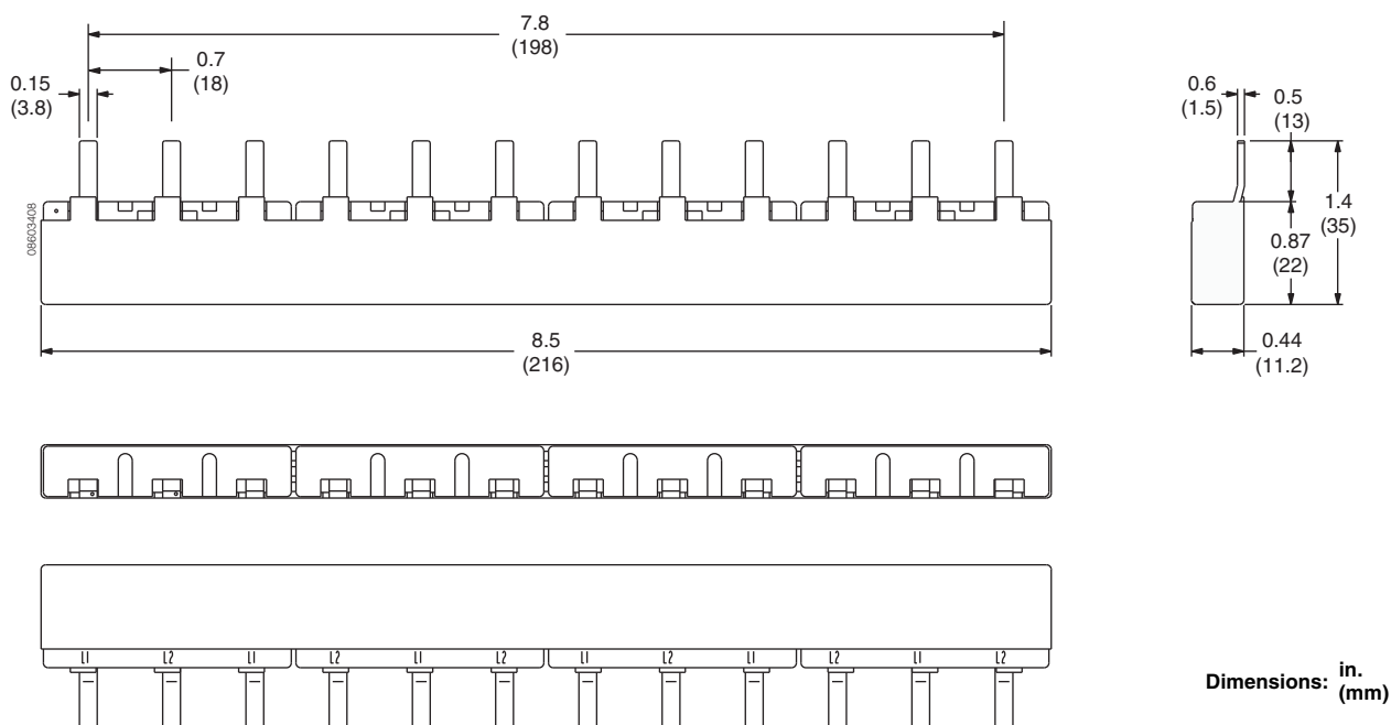
Figure 45: Multi 9 UL C60 Mounting Base
