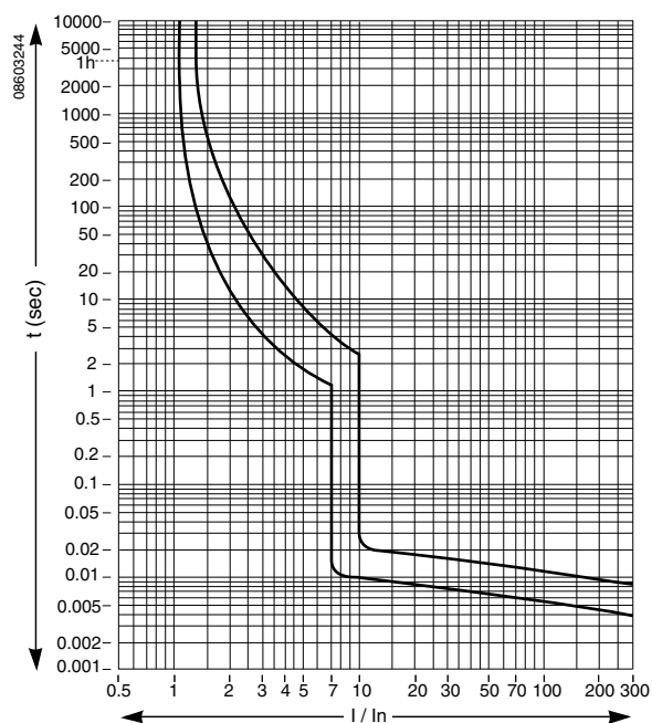
Figure 76: IEC Rated C60N/H/L—C Curve
