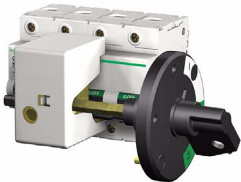
Operating Subassembly with Lateral Rotary Handle
