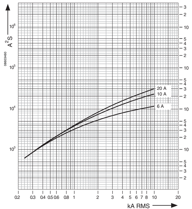
Figure 90: UL 1077 Recognized C60 2P, 3P, and 4P (480 Vac) Maximum Let-Through I 2 t Current
