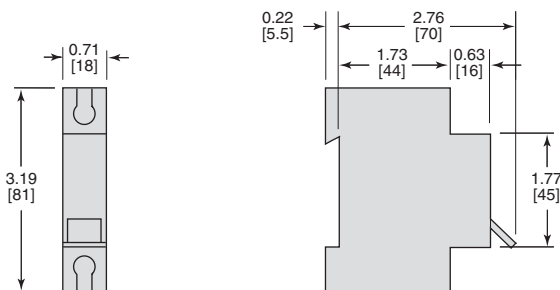
Figure 26: UL 489A Listed C60 60 Vdc Circuit Breakers for DC Telecommunications Applications
