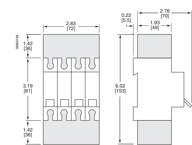
Figure 41: Terminal Cover for UL 489A, UL 1077 and IEC C60 Devices
