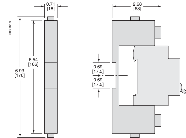
Figure 40: Plug-In Base for UL 489A, UL 1077 and IEC C60 Devices
