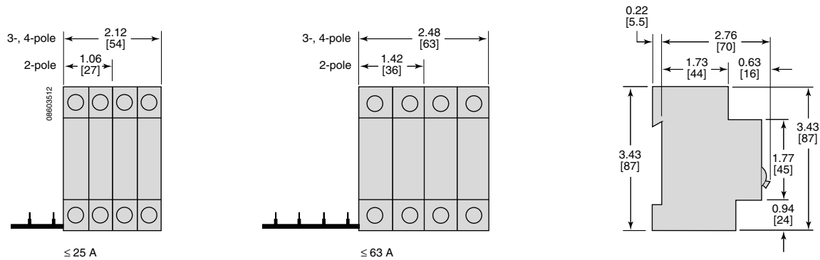
Figure 32: IEC Vigı Ground-Fault Module for C60 Devices
