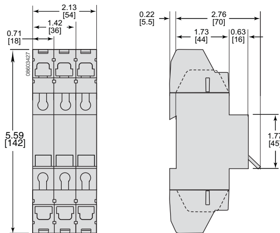
Figure 25: UL 489/CSA C22.2 No.5 C60 480 Vac and 240 Vac Circuit Breaker with Fingersafe Shields
