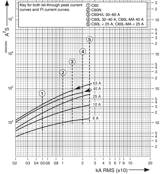
Figure 96: IEC Rated C60 2P, 3P and 4P (230/240 Vac) Maximum Let-Through I^2t Current
