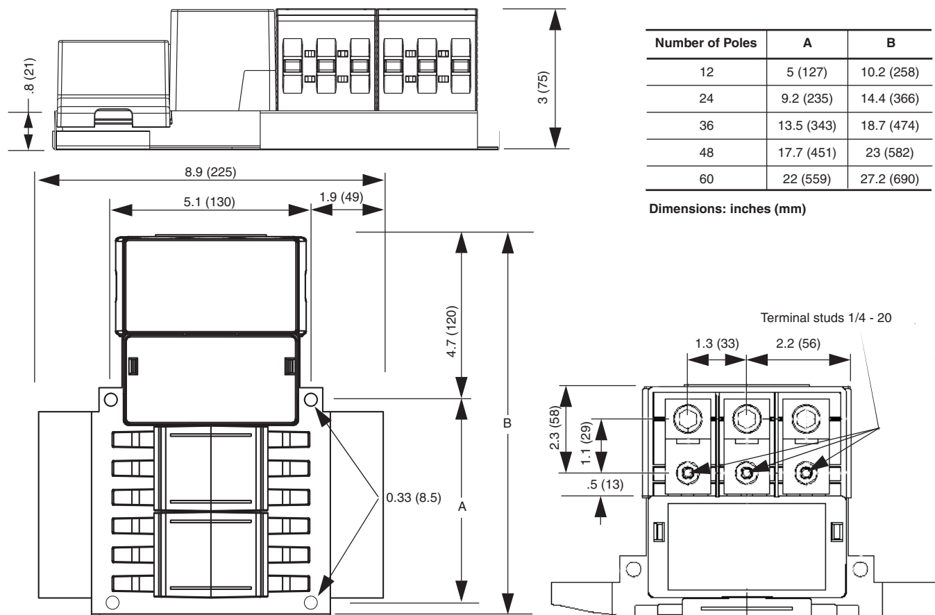
Figure 45: Multi 9 UL C60 Mounting Base
