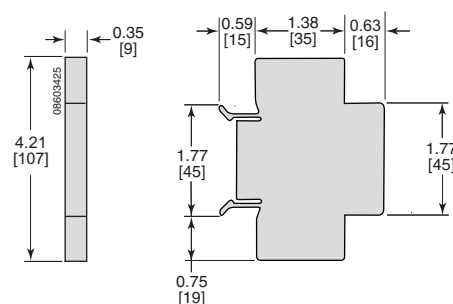
Figure 37: Spacer for C60 and C120 Devices
