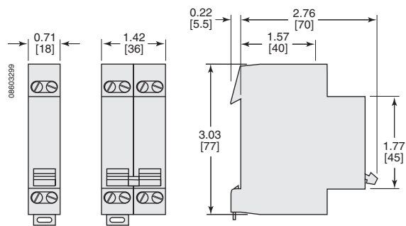
Figure 52: I Switch (20–32 A)
