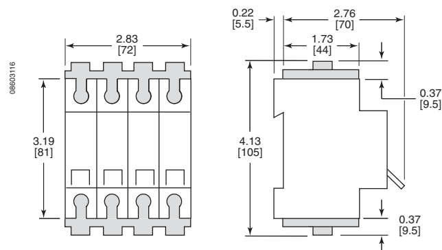
Figure 39: Terminal Screw Shield for UL 489A, UL 1077 and IEC C60 Devices
