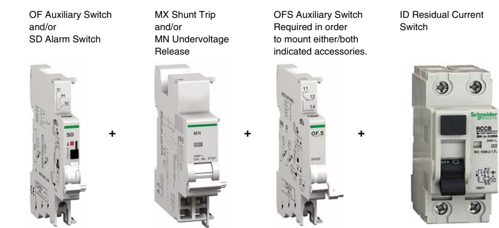
Figure 9: Possible Device Combinations
