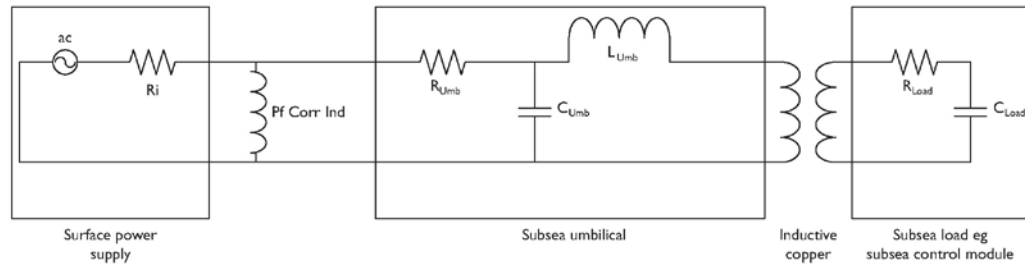
Figure 4 – Schematic of a typical subsea power circuit
