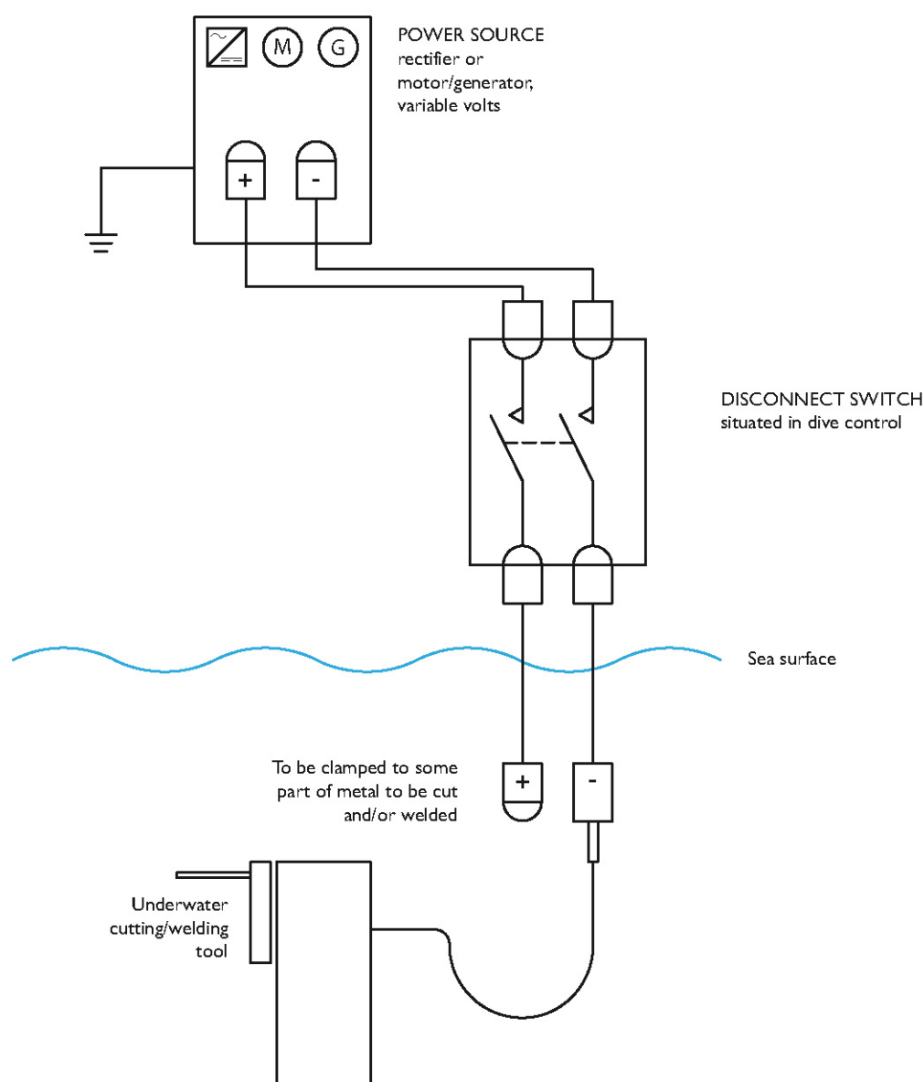
Figure 7 – Schematic of wet welding/cutting
