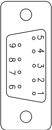
DB9F CONNECTOR PINOUTS (FACE VIEW)
