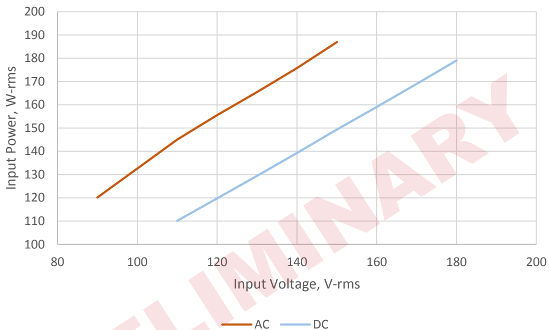
LSL-1000: Real Power vs. RMS Input Voltage
