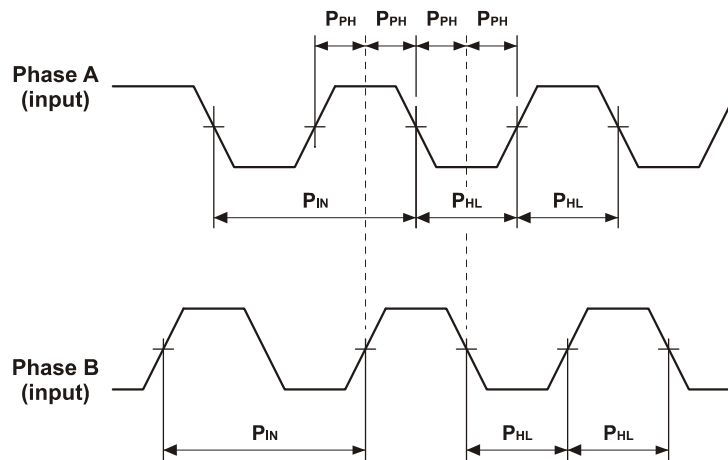
Figure A-2: Auxiliary Feedback - Encoder Phase Diagram
