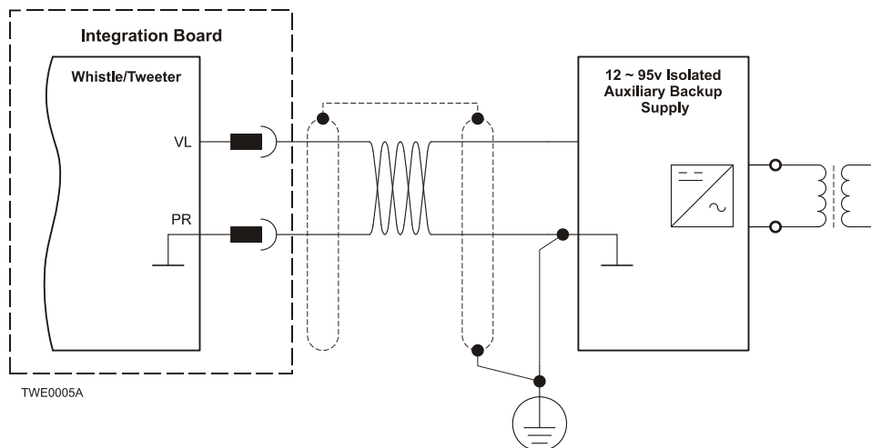
Figure 3-7: Separate Auxiliary Supply Connection Diagram
