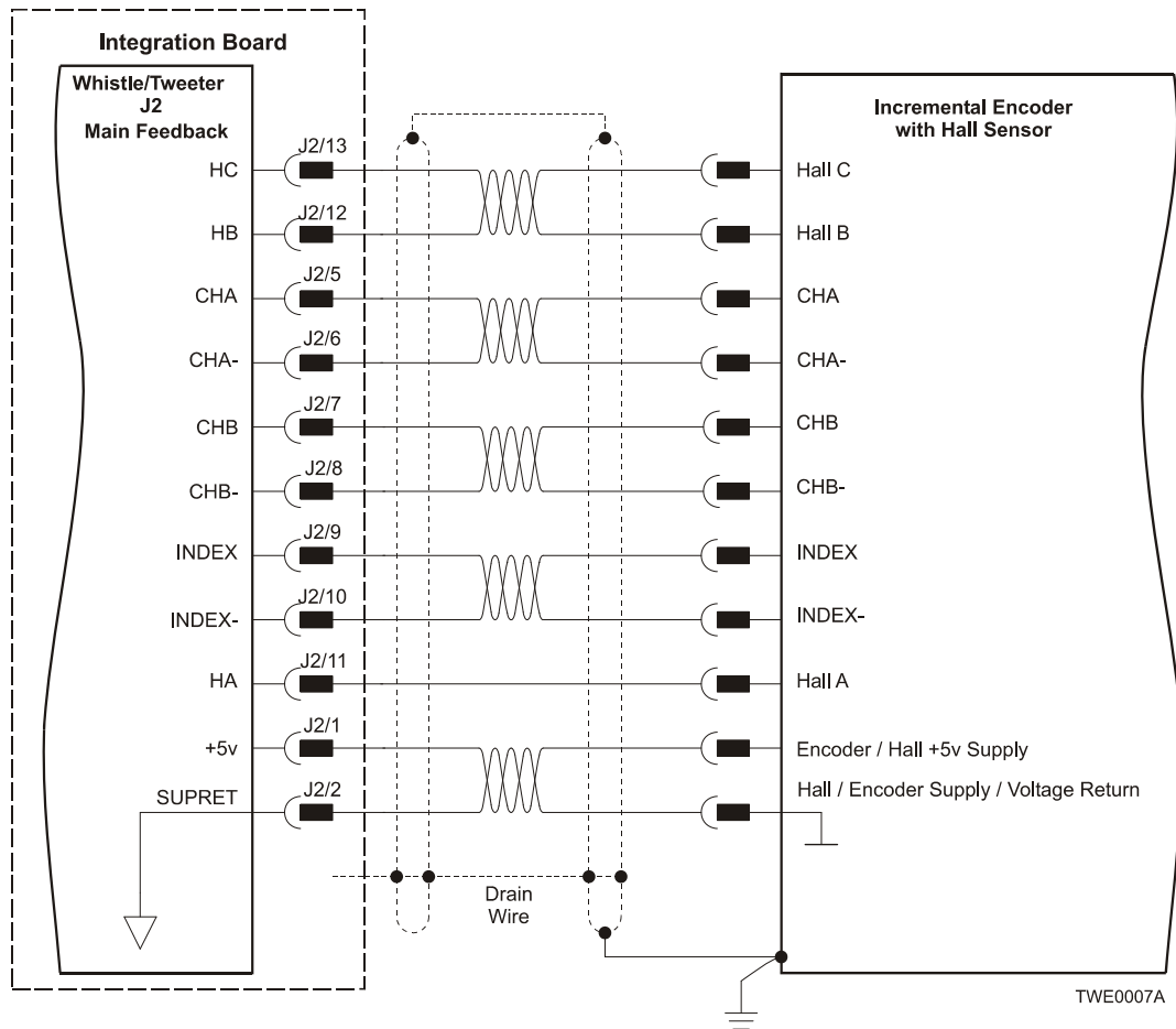
Figure 3-9: Main Feedback- Incremental Encoder Connection Diagram
