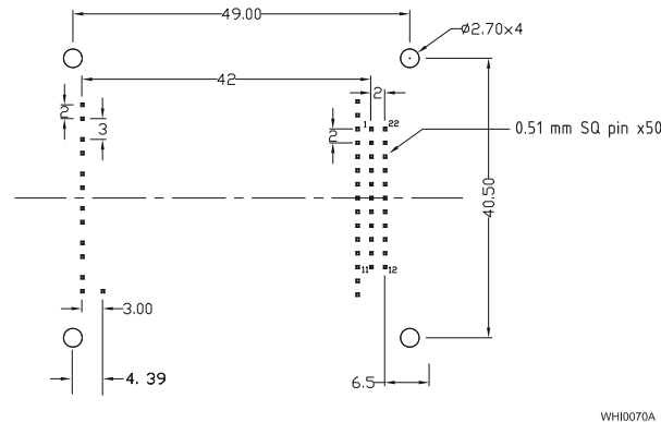
Figure 3-1: The Whistle Footprint
