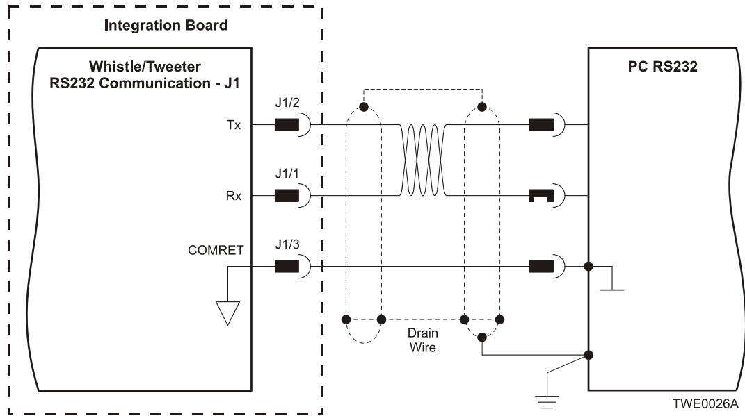
Figure 3-28: RS-232 Connection Diagram
