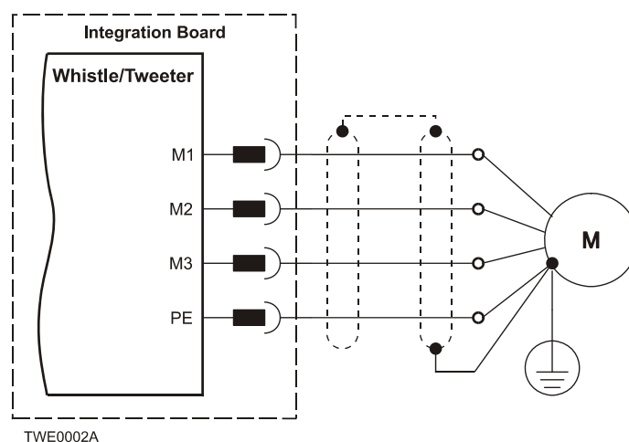
Figure 3-4: AC Motor Power Connection Diagram
