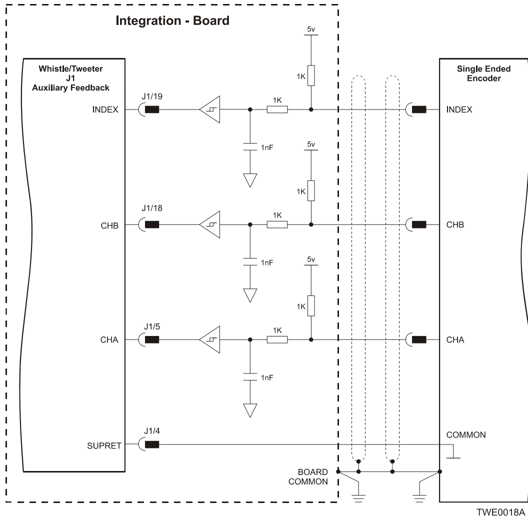
Figure 3-20: Single-ended Auxiliary Encoder Input - Recommended Connection Diagram
