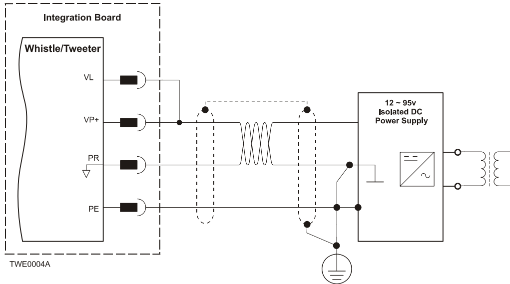
Figure 3-6: Single Supply for both the Main Power Supply and the Auxiliary Supply
