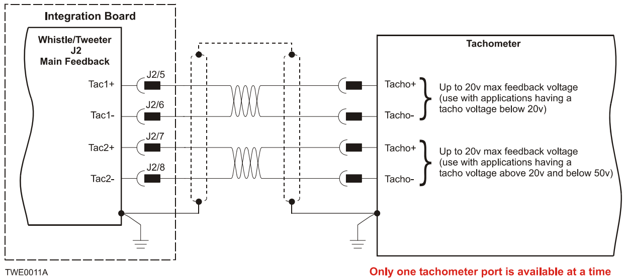
Figure 3-13: Main Feedback - Tachometer Feedback Connection Diagram for Brush Motors
