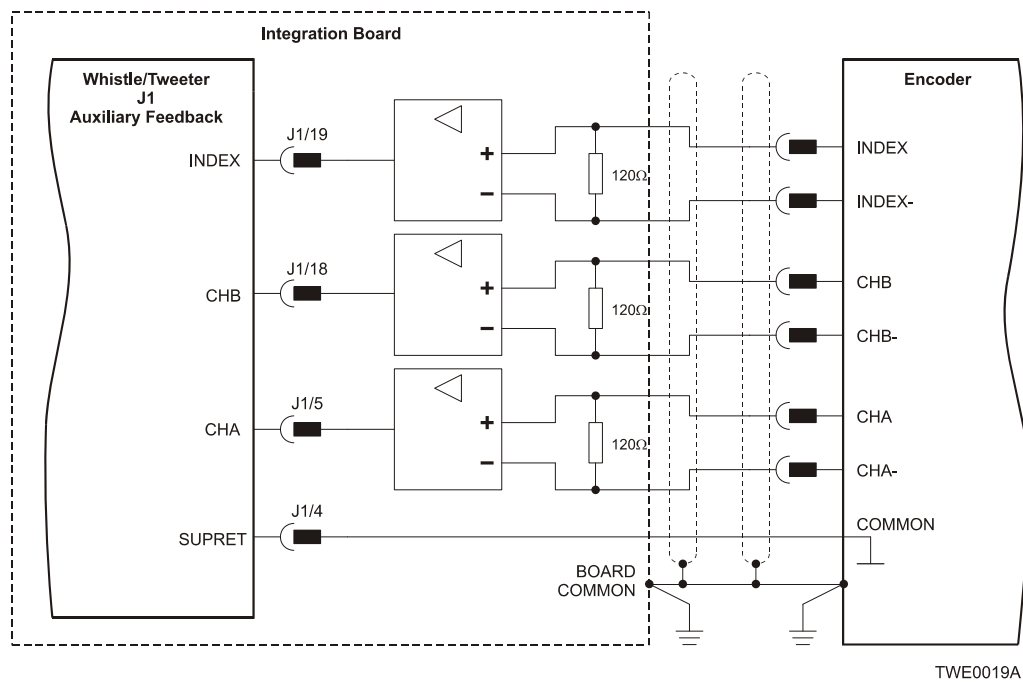
Figure 3-21: Differential Auxiliary Encoder Input - Highly Recommended Connection Diagram
