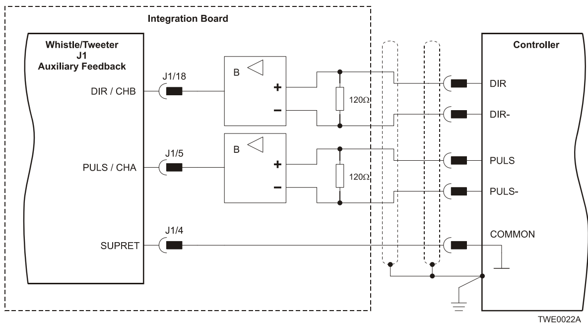
Figure 3-24: Pulse-and-Direction Auxiliary Encoder Input - Differential Connection Diagram
