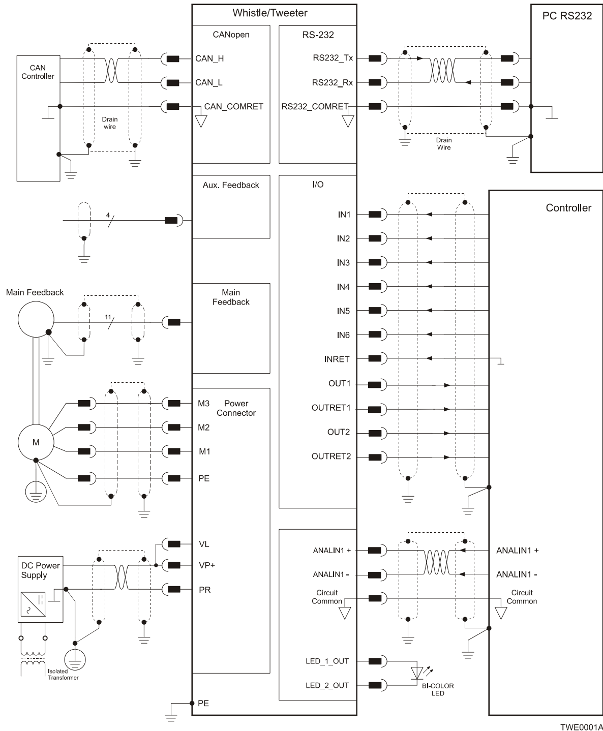
Figure 3-3: Whistle/Tweeter Connection Diagram
