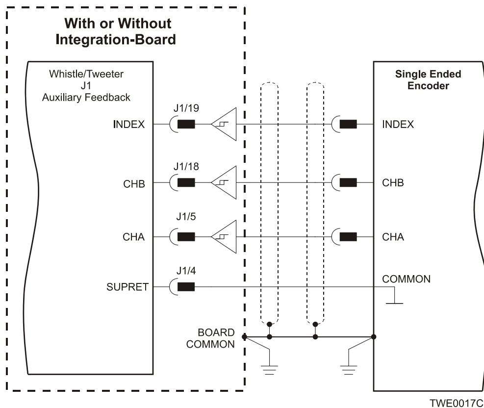
Figure 3-19: Single-ended Auxiliary Encoder Input - Acceptable Connection Diagram
