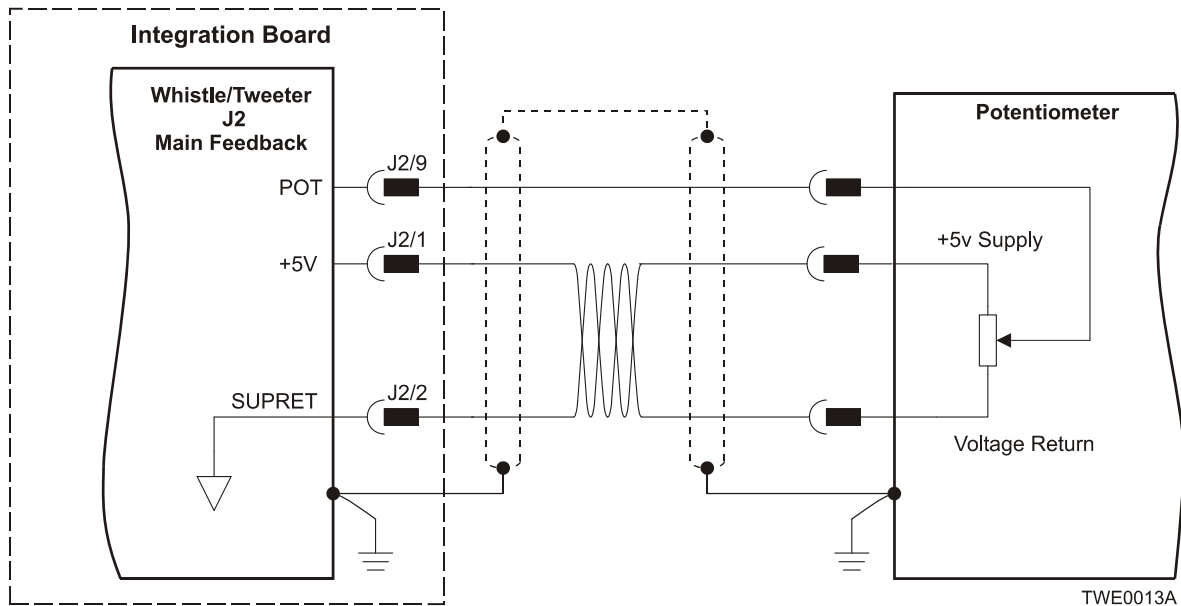
Figure 3-15: Main Feedback – Potentiometer Feedback Connection Diagram for Brush Motors and Voice Coils
