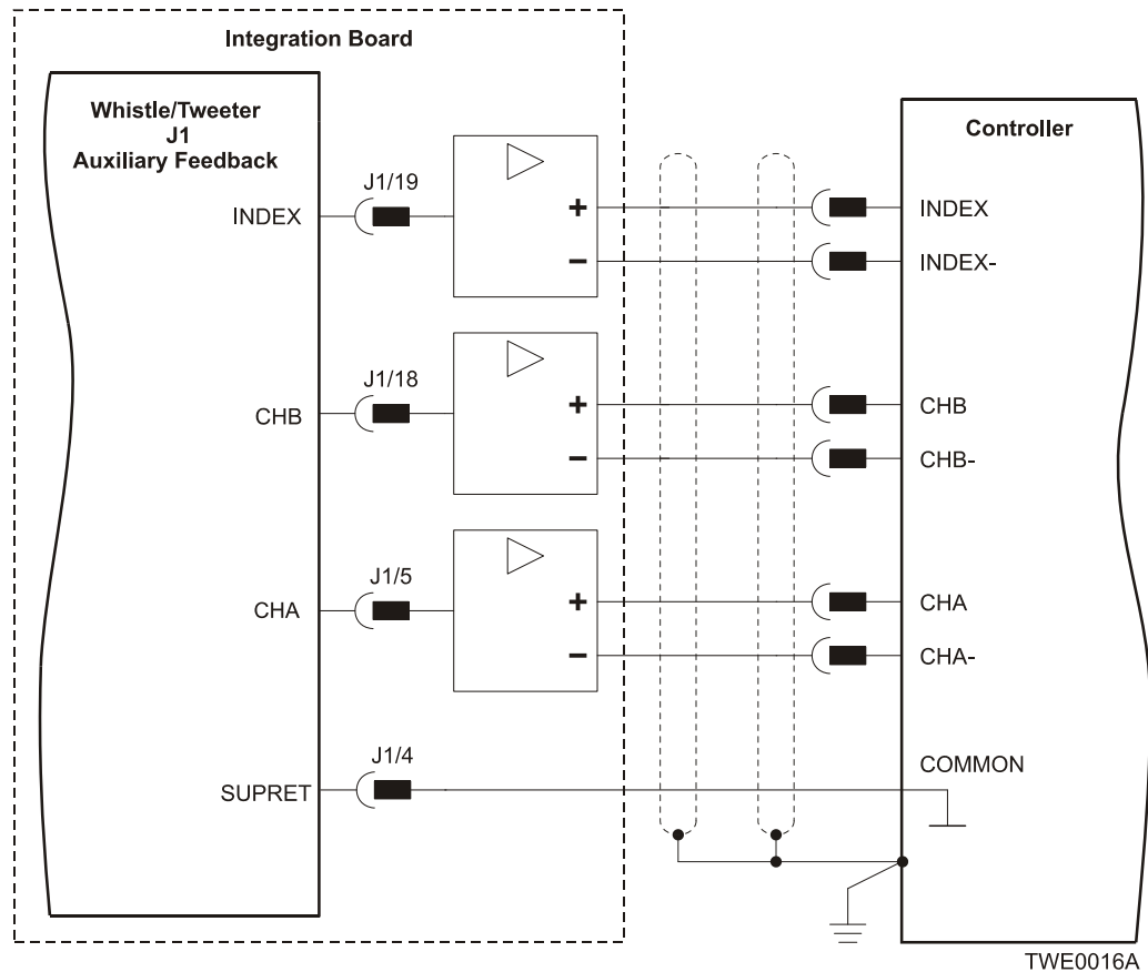
Figure 3-18: Emulated Encoder Differential Output - Highly Recommended Connection Diagram
