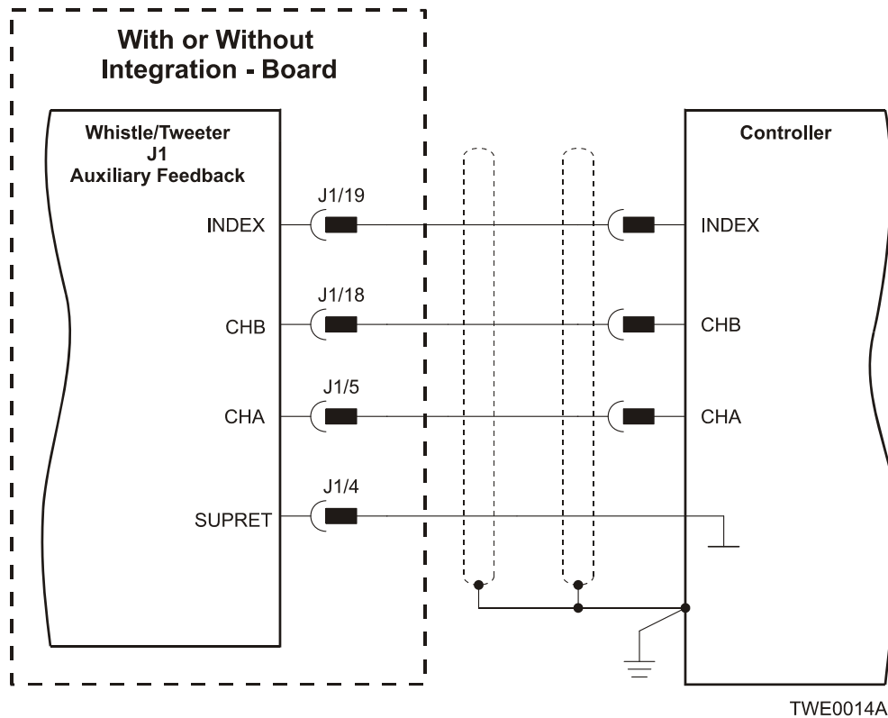
Figure 3-16: Emulated Encoder Direct Output - Acceptable Connection Diagram
