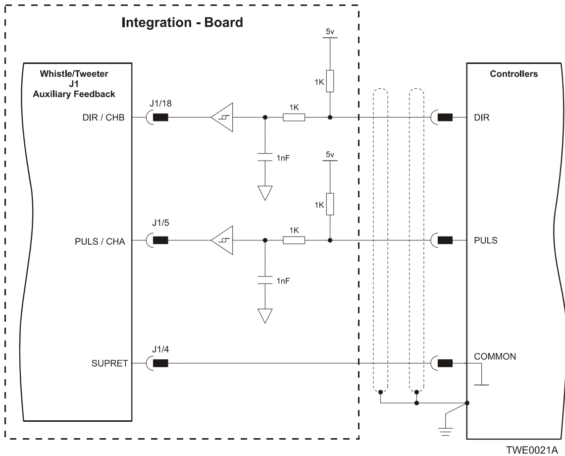
Figure 3-23: Pulse-and-Direction Auxiliary Encoder Input - Buffered Connection Diagram
