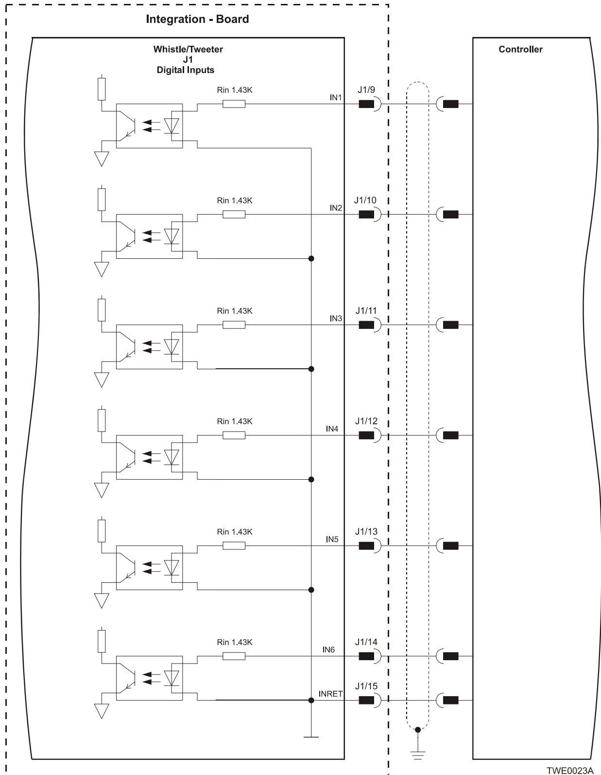
Figure 3-25: Digital Input Connection Diagram
