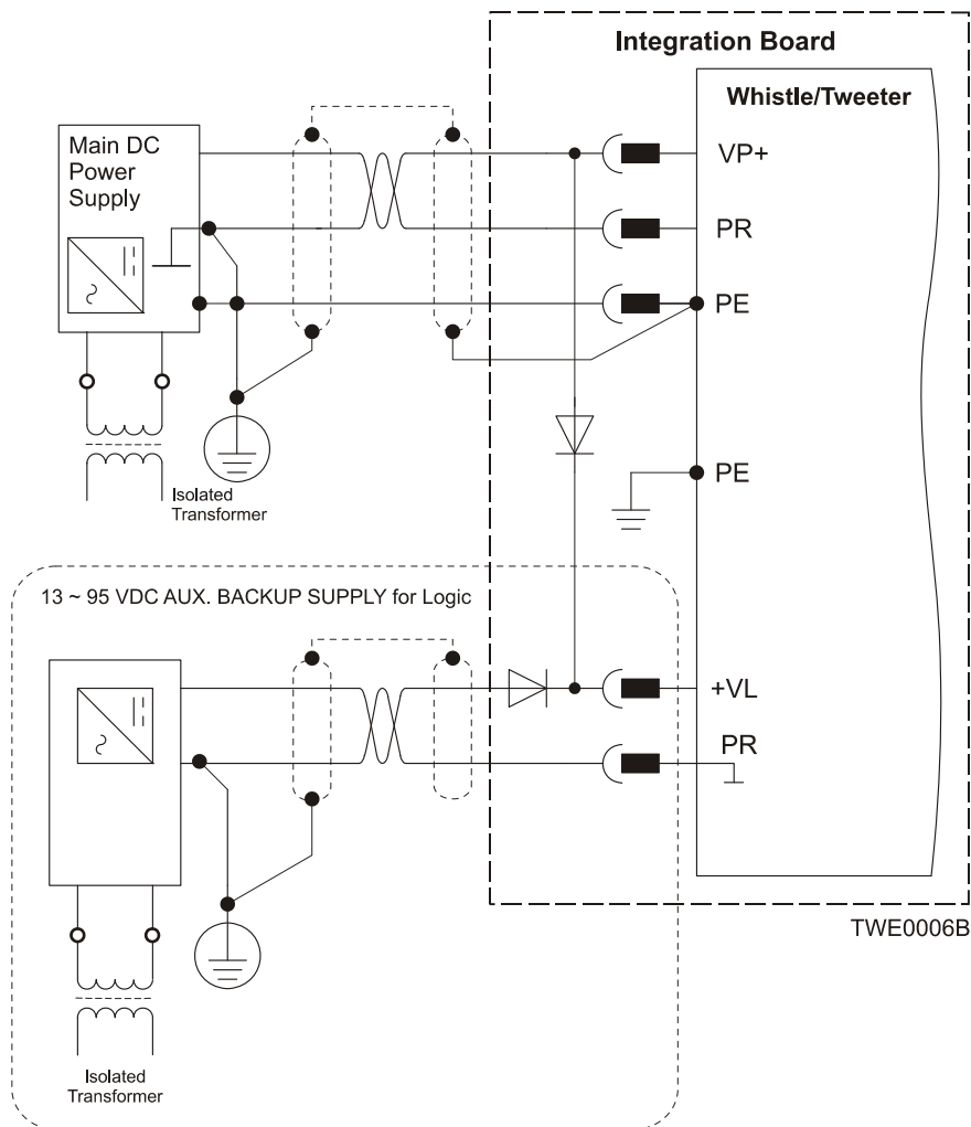
Figure 3-8: Shared Supply Connection Diagram
