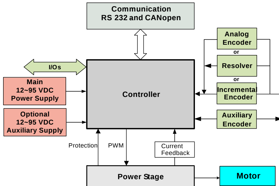
Figure 2-1: Whistle/Tweeter System Block Diagram
