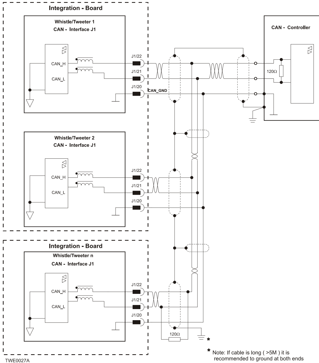
Figure 3-29: CANopen Network Diagram
