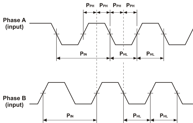
Figure A-3: Auxiliary Feedback - Encoder Phase Diagram
