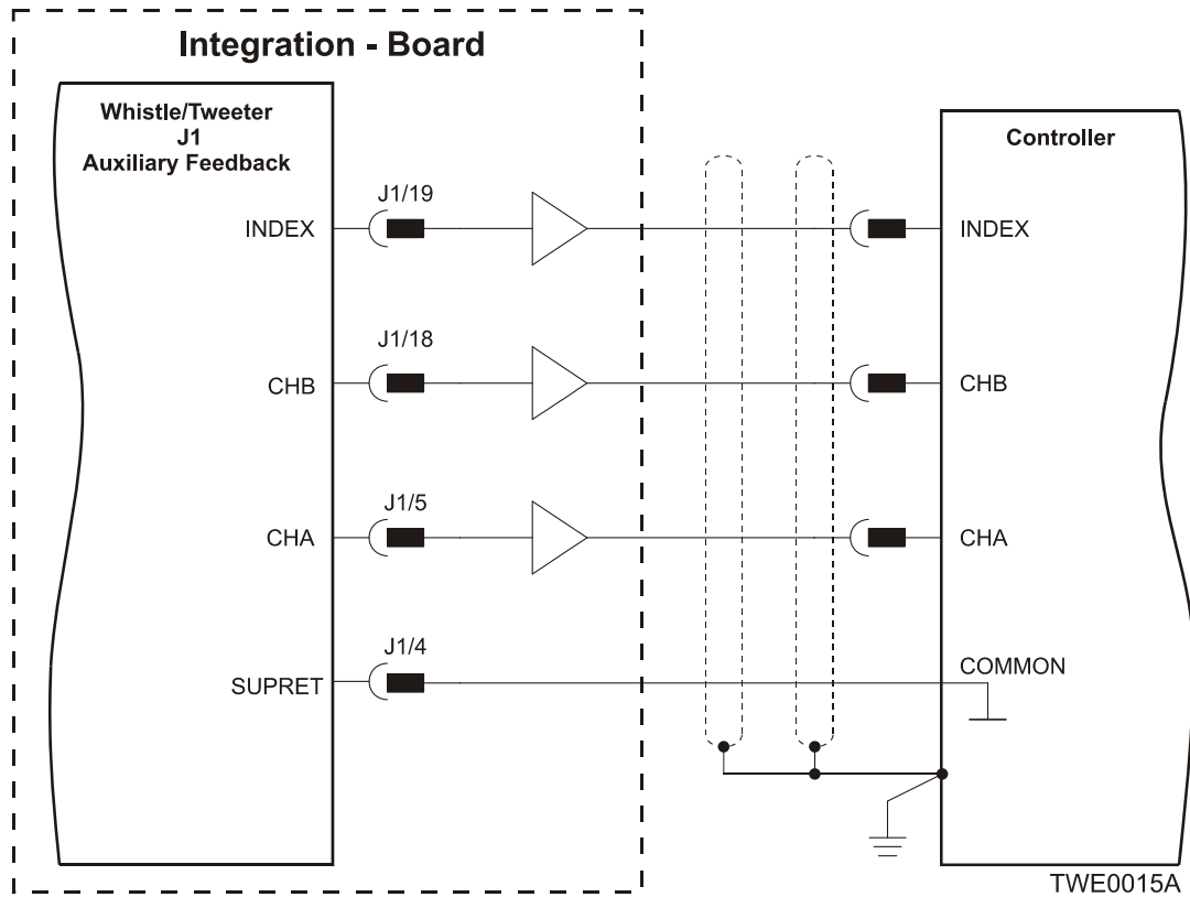
Figure 3-17: Emulated Encoder Buffered Output - Recommended Connection Diagram
