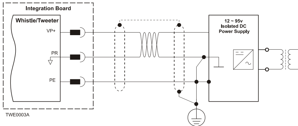
Figure 3-5: Main Power Supply Connection Diagram
