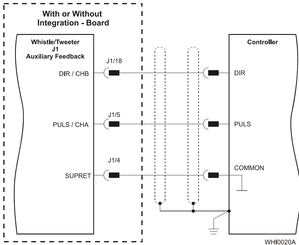
Figure 3-22: Pulse-and-Direction Auxiliary Encoder Input - Direct Connection Diagram
