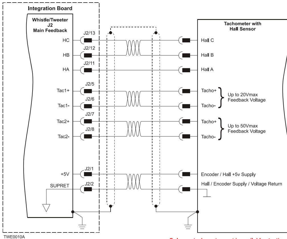
Figure 3-12: Main Feedback - Tachometer Feedback with Digital Hall Sensor Connection Diagram for Brushless Motors
