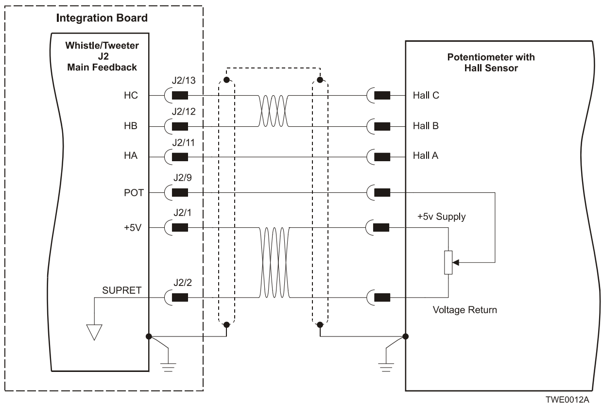
Figure 3-14: Main Feedback - Potentiometer Feedback with Digital Hall Sensor Connection Diagram for Brushless Motors
