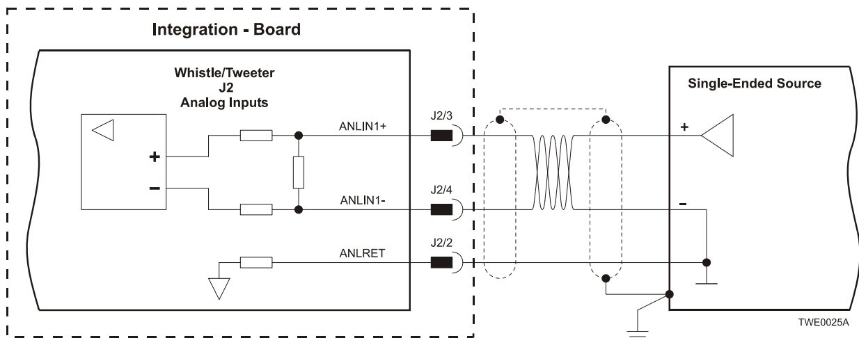
Figure 3-27: Analog Input with Single-ended Source
