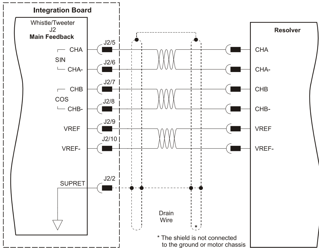
Figure 3-11: Main Feedback - Resolver Connection Diagram
