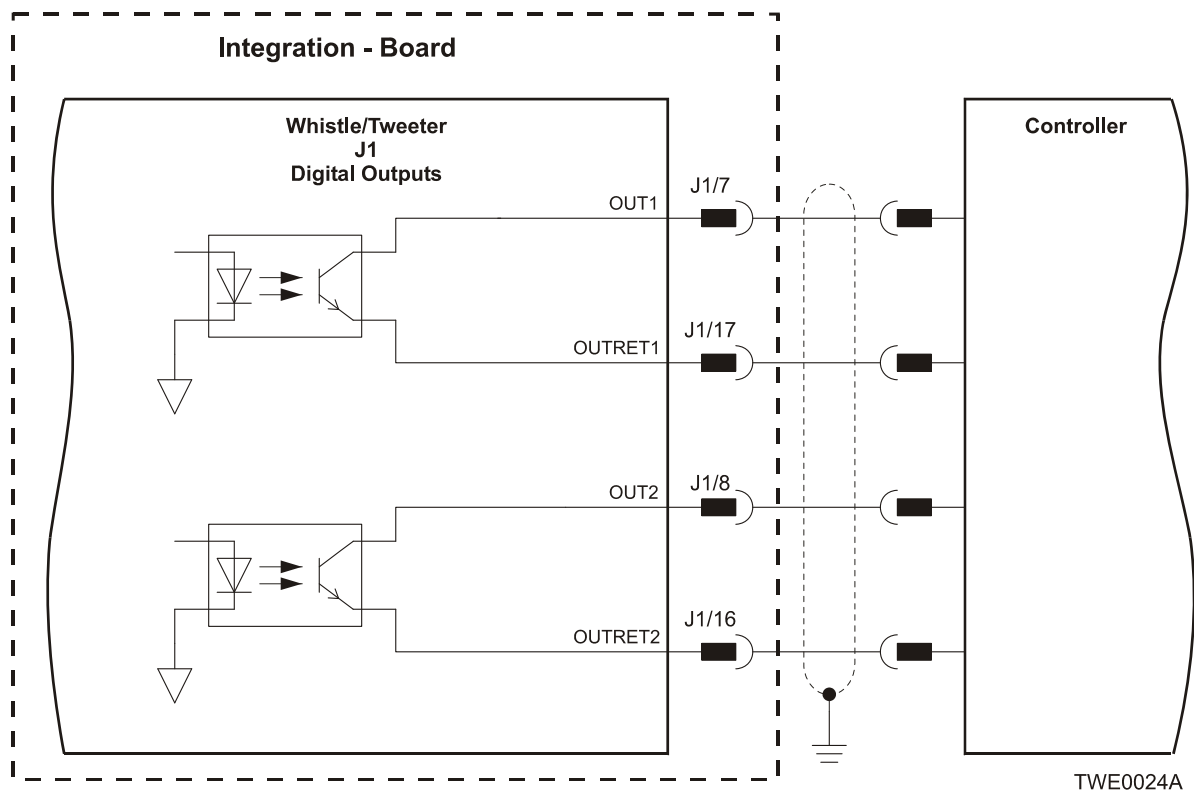
Figure 3-26: Digital Output Connection Diagram
