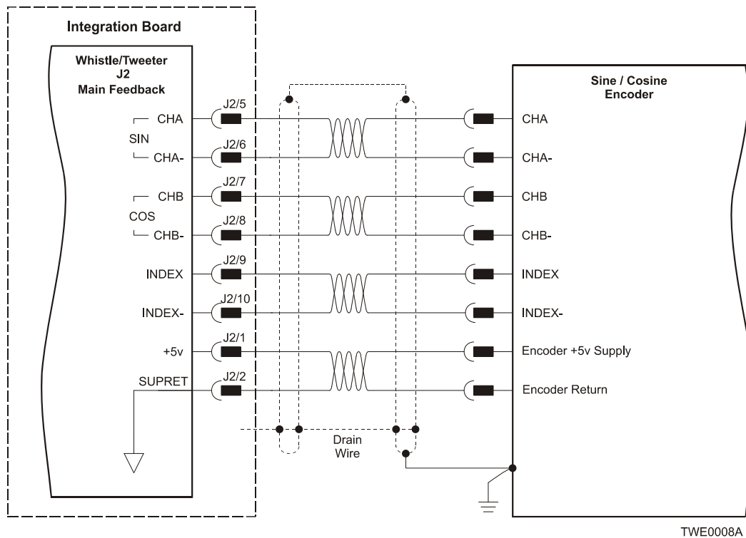
Figure 3-10: Main Feedback - Interpolated Analog Encoder Connection Diagram
