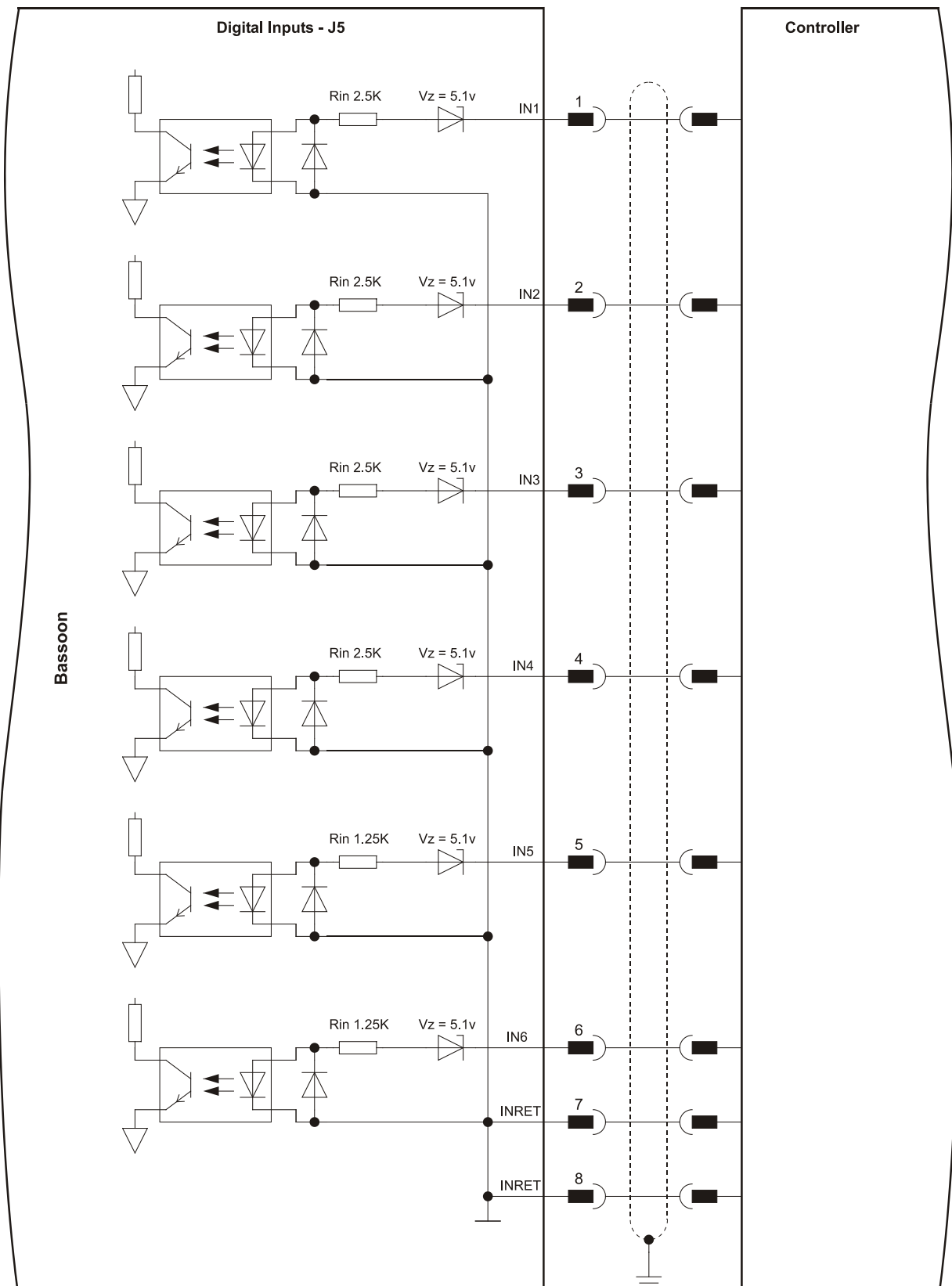
Figure 26: Digital Input Connection Diagram
