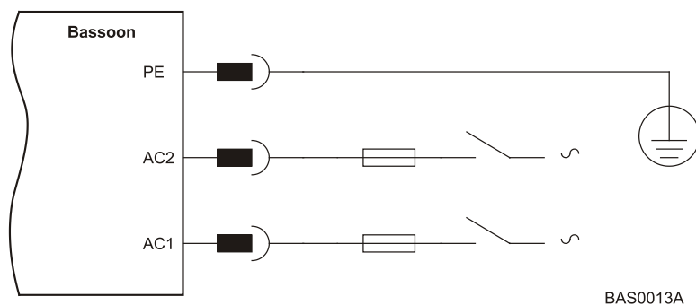
Figure 8: Main Power Supply Connection Diagram
