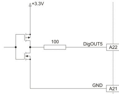
Figure 4-19 DigOUT5 Circuit
