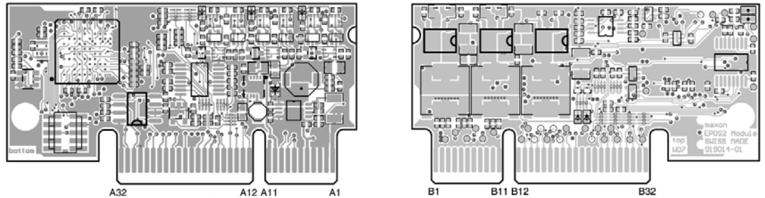
Figure 4-6 EPOS2 Module 36/2 – PCB with Connector Array
