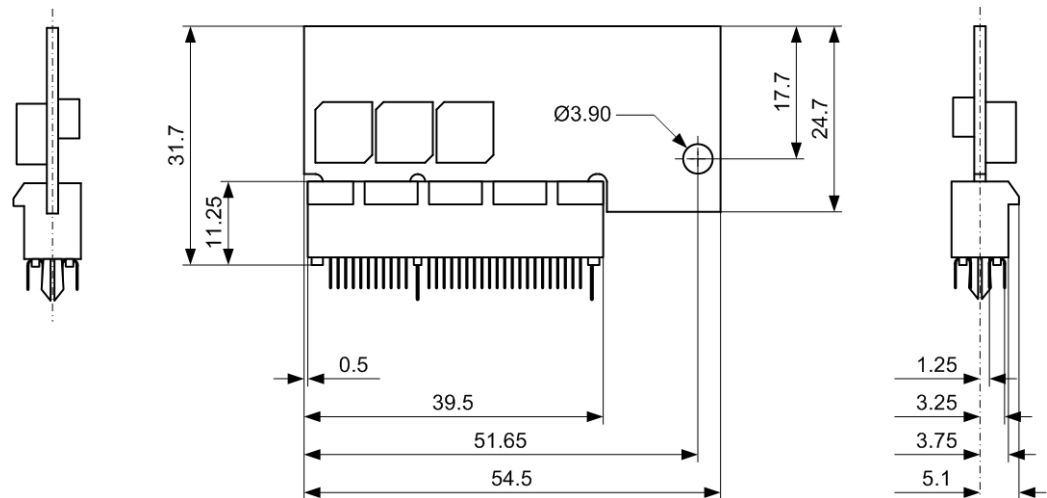
Figure 3-2 Dimensional Drawing (with vertical Connector) [mm]
