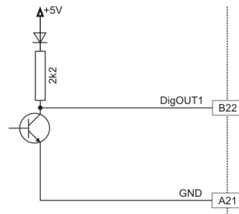
Figure 4-16 DigOUT1 Circuit (analogously valid also for DigOUT2)
