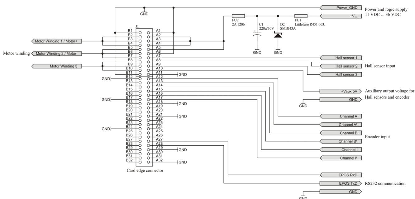
Figure 4-7 Minimum external Wiring
