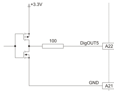
Figure 4-19 DigOUT5 Circuit
