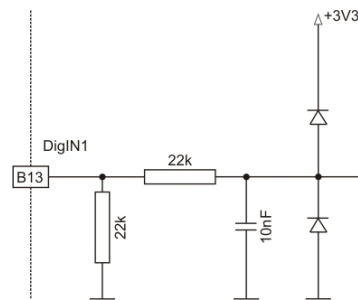
Figure 4-10 DigIN1 Circuit (analogously valid also for DigIN2...4)
