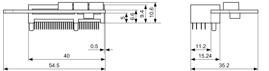
Figure 3-3 Dimensional Drawing (with horizontal connector Meritec 983172-064-2MMF) [mm]
