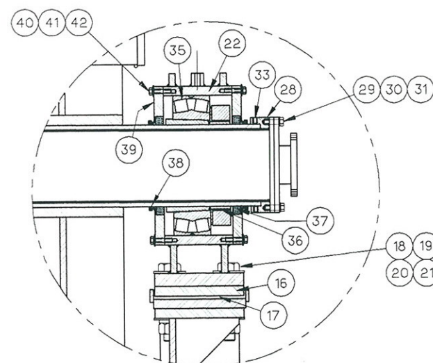
DETAIL E SCALE X3
