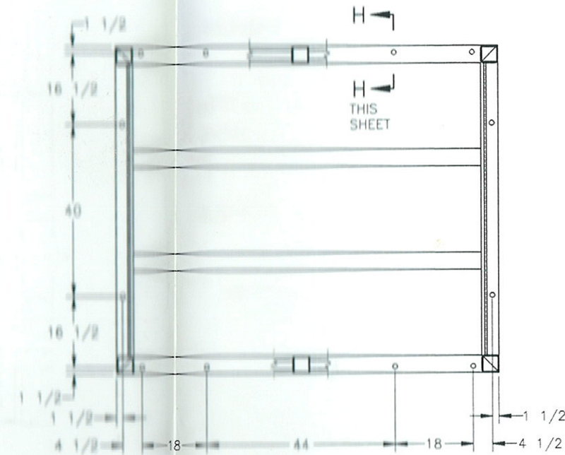
SECTION G-G
