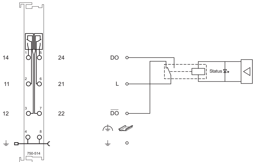
Fig. 2.1.1-3: 2-Channel Relay Output Module 750-514
