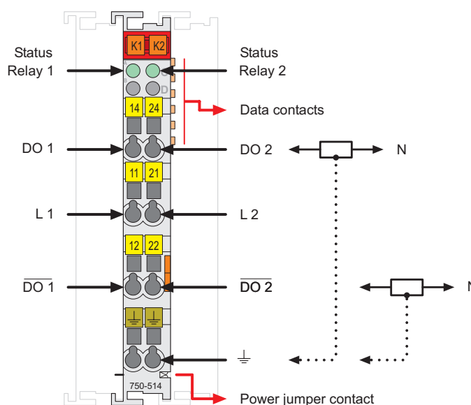
Fig. 2.1.1-1: 2-Channel Relay Output Module 750-514
