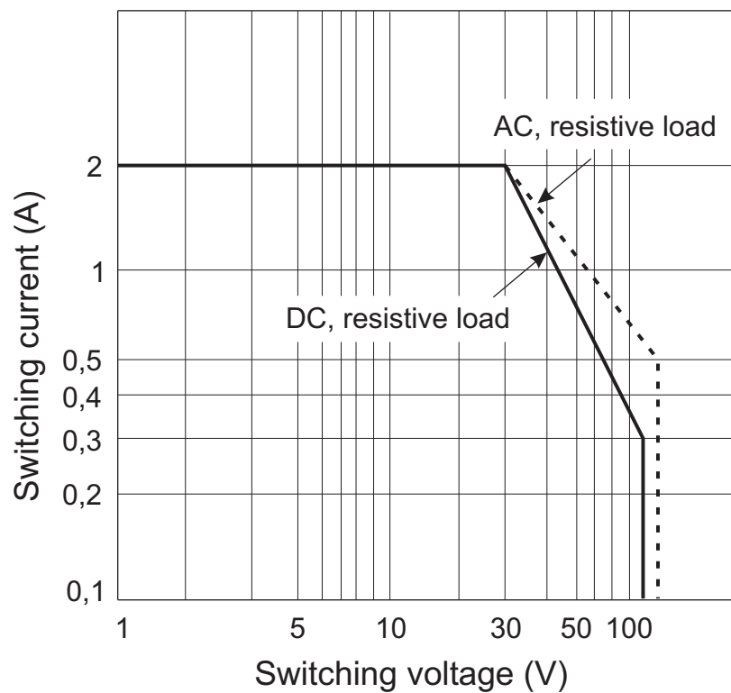
Fig. 2.1.1-4: Load limiting value graph of the relay
