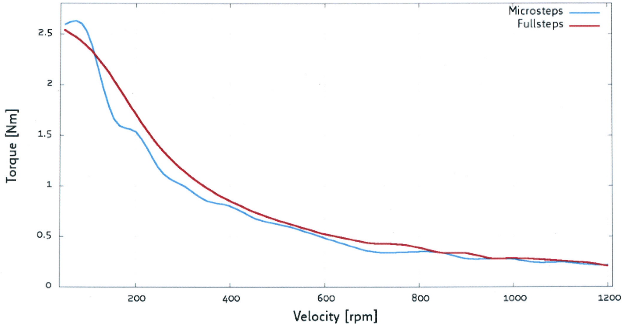
Figure 8.7 Torque curves PD60-4-1160, V_S = 24 V DC
