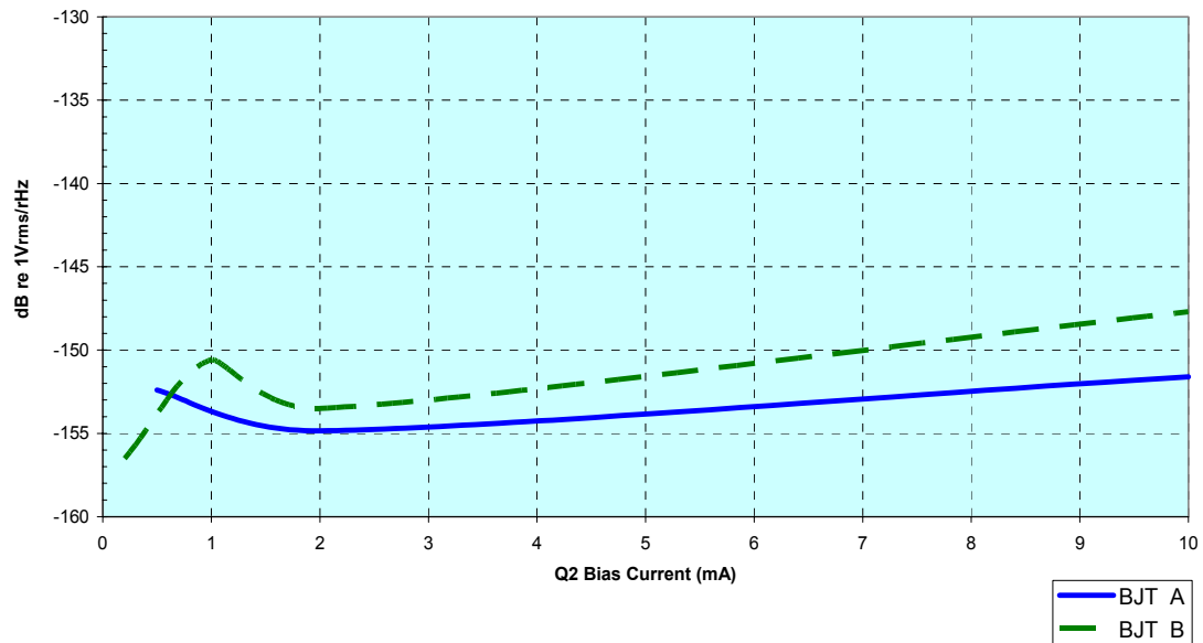
Figure 16. Receiving Results in dB re 1V/Hz 1/2 for Candidate NPN BJTs
