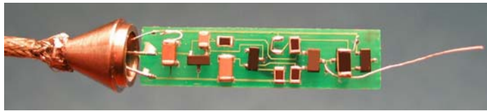
Figure 7. Cable Fitting and Wires Soldered to the Preamplifier
