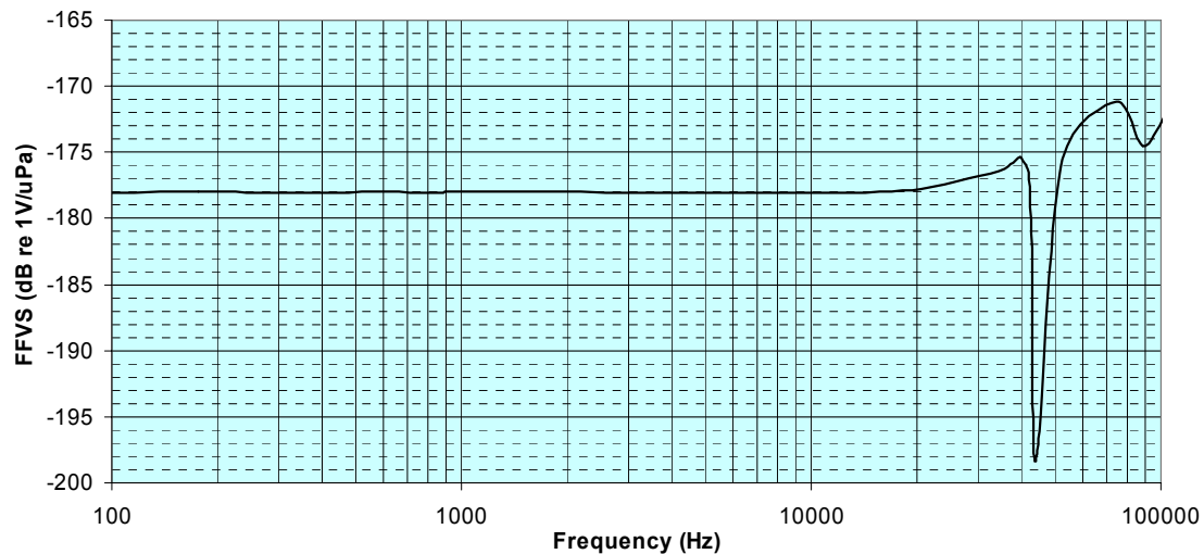
Figure 23. Total Free Voltage Sensitivity of Mini CylinderCan 2-2 Combining Two Different Sound Sources and Two Different Frequency Ranges
