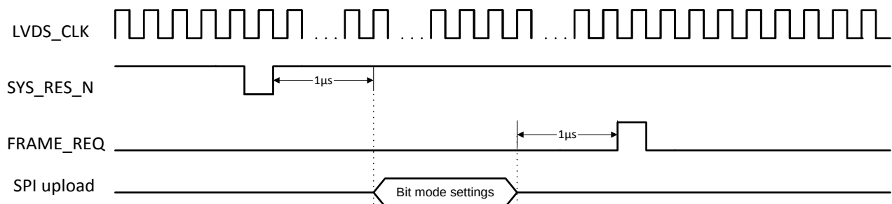
FIGURE 6: RESET SEQUENCE WHEN CHANGING BIT MODE
