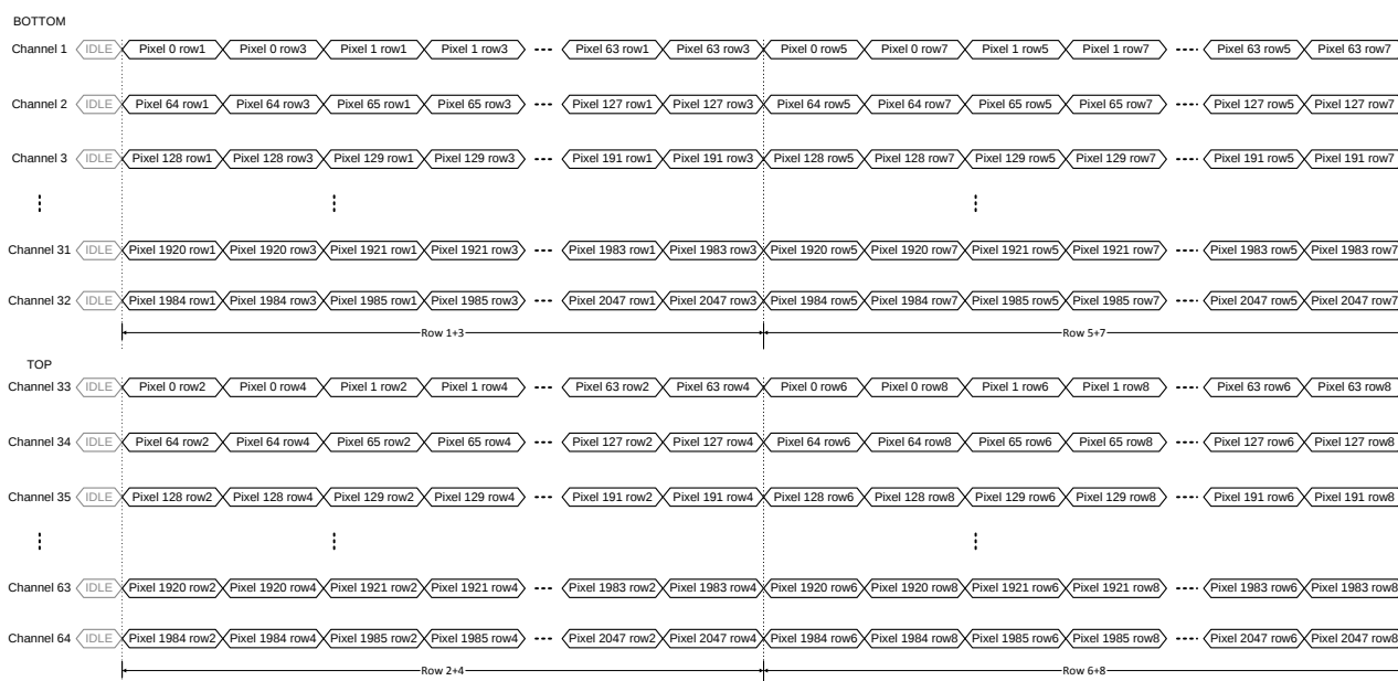
FIGURE 45: MONOCHROME SUBSAMPLING IN X AND Y, PIXEL TO OUTPUT REMAPPING
