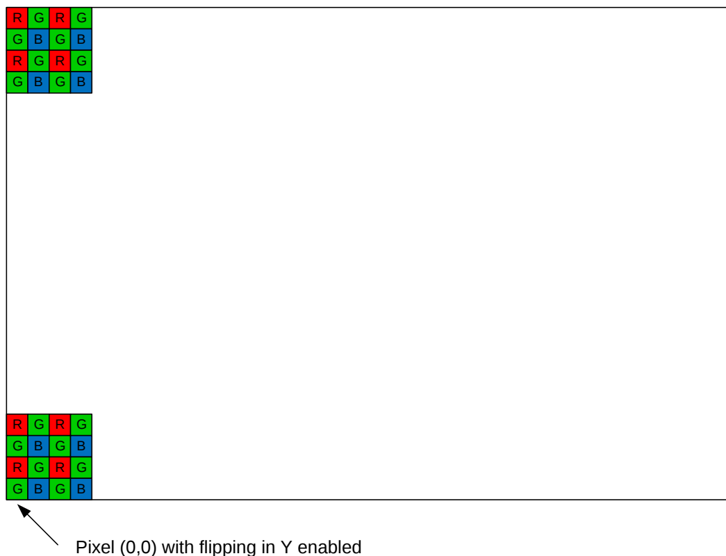
FIGURE 56: COLOR FILTER BAYER PATTERN
