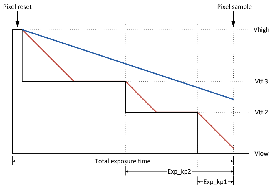
FIGURE 37: MULTIPLE SLOPE DETAILS
