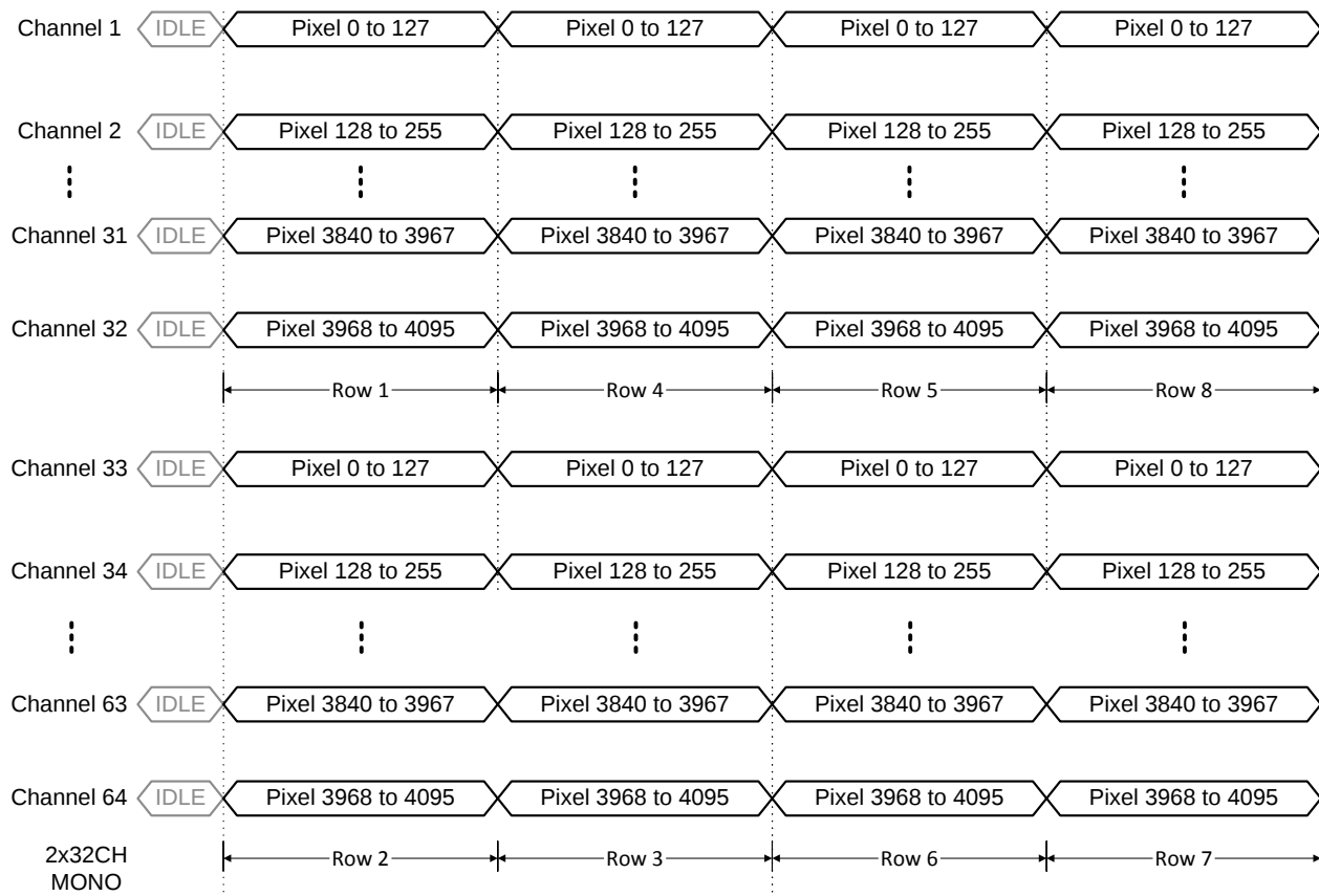
FIGURE 43: MONOCHROME SUBSAMPLING IN Y, PIXEL TO OUTPUT REMAPPING
