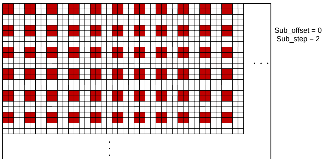
FIGURE 48: COLOR SUBSAMPLING IN X AND Y (SKIP 2X)
