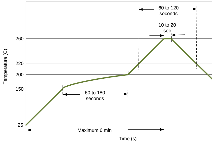
FIGURE 58: REFLOW SOLDERING
