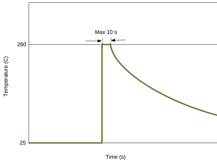
FIGURE 57: WAVE SOLDERING PROFILE
