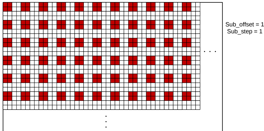
FIGURE 52: COLOR BINNING (SKIP 2X)
