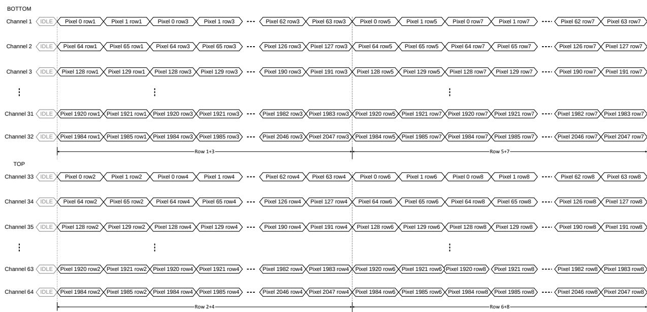
FIGURE 49: COLOR SUBSAMPLING IN X AND Y, PIXEL TO OUTPUT REMAPPING
