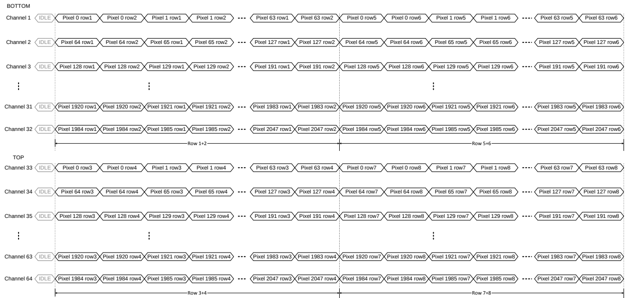
FIGURE 51: MONOCHROME BINNING, PIXEL TO OUTPUT REMAPPING
