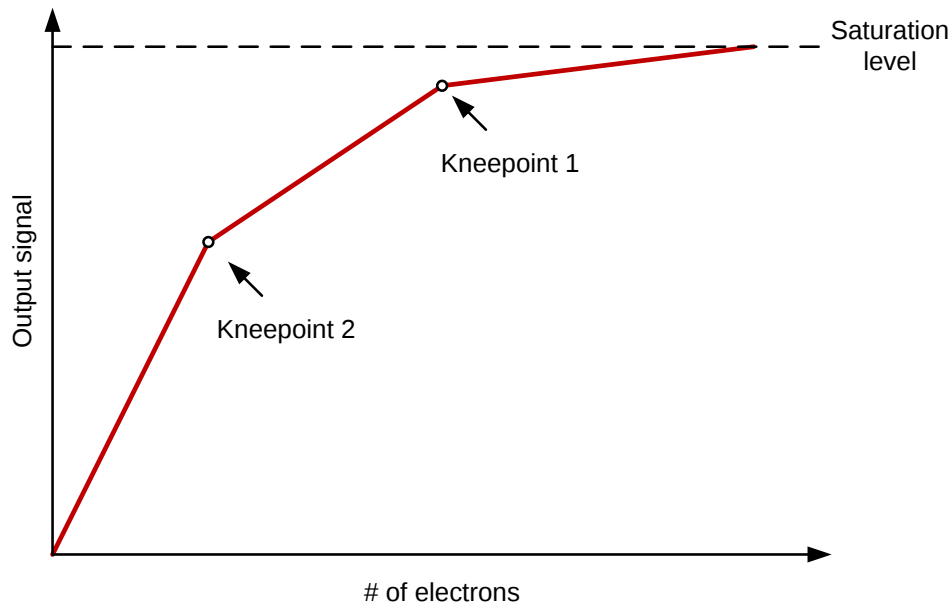
FIGURE 38: MULTIPLE SLOPE RESPONSE
