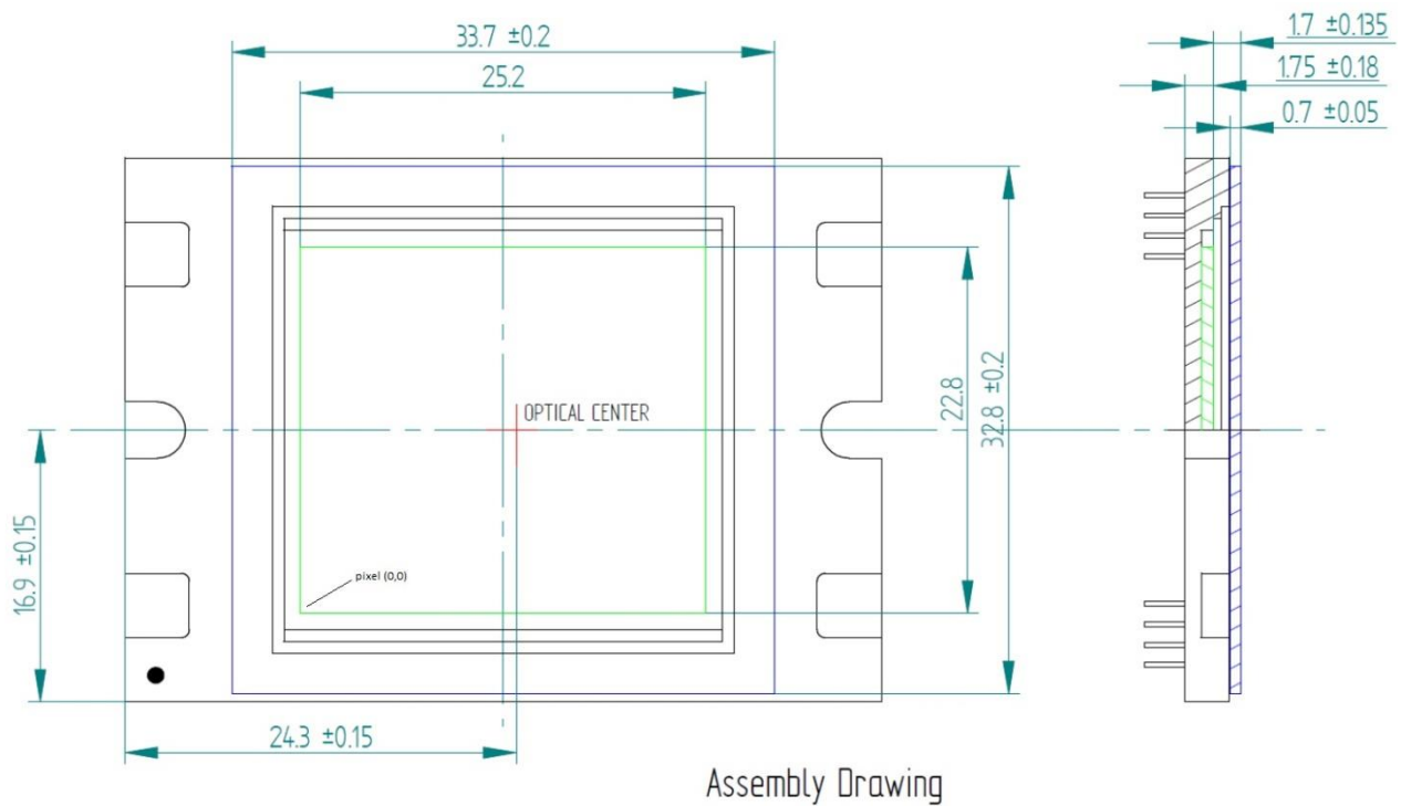
FIGURE 55: ASSEMBLY DRAWING OF CMV12000 WITH COVER GLASS AND SENSOR DIE, ALL DISTANCES IN MM
