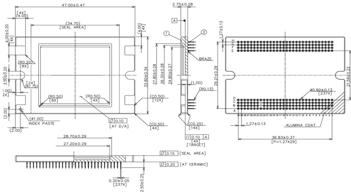
FIGURE 54: PACKAGE DRAWING OF THE CMV12000, ALL DISTANCES IN MM
