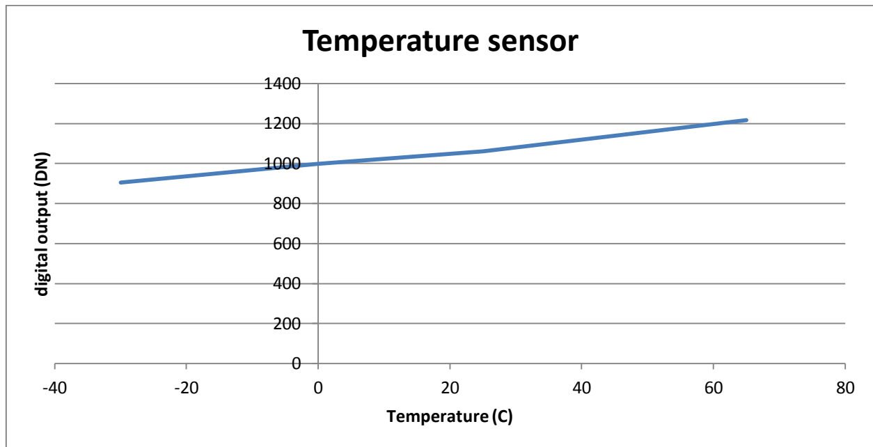
FIGURE 3: TYPICAL OUTPUT OF THE TEMPERATURE SENSOR OF THE CMV12000
