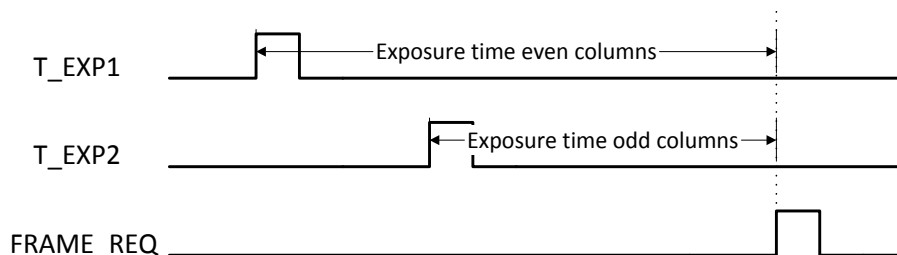
FIGURE 36: INTERLEAVED READ-OUT IN EXTERNAL EXPOSURE MODE
