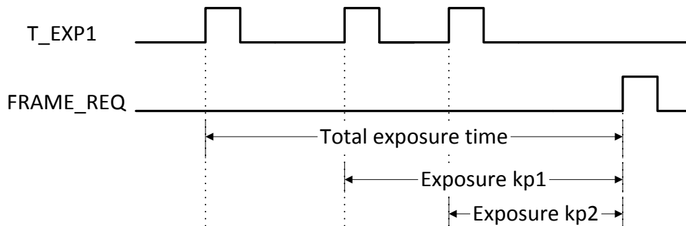
FIGURE 39: MULTIPLE SLOPE IN EXTERNAL EXPOSURE MODE
