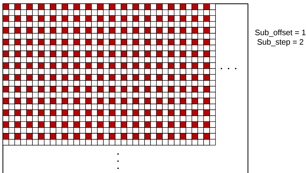
FIGURE 44: MONOCHROME SUBSAMPLING IN X AND Y (SKIP 1X)
