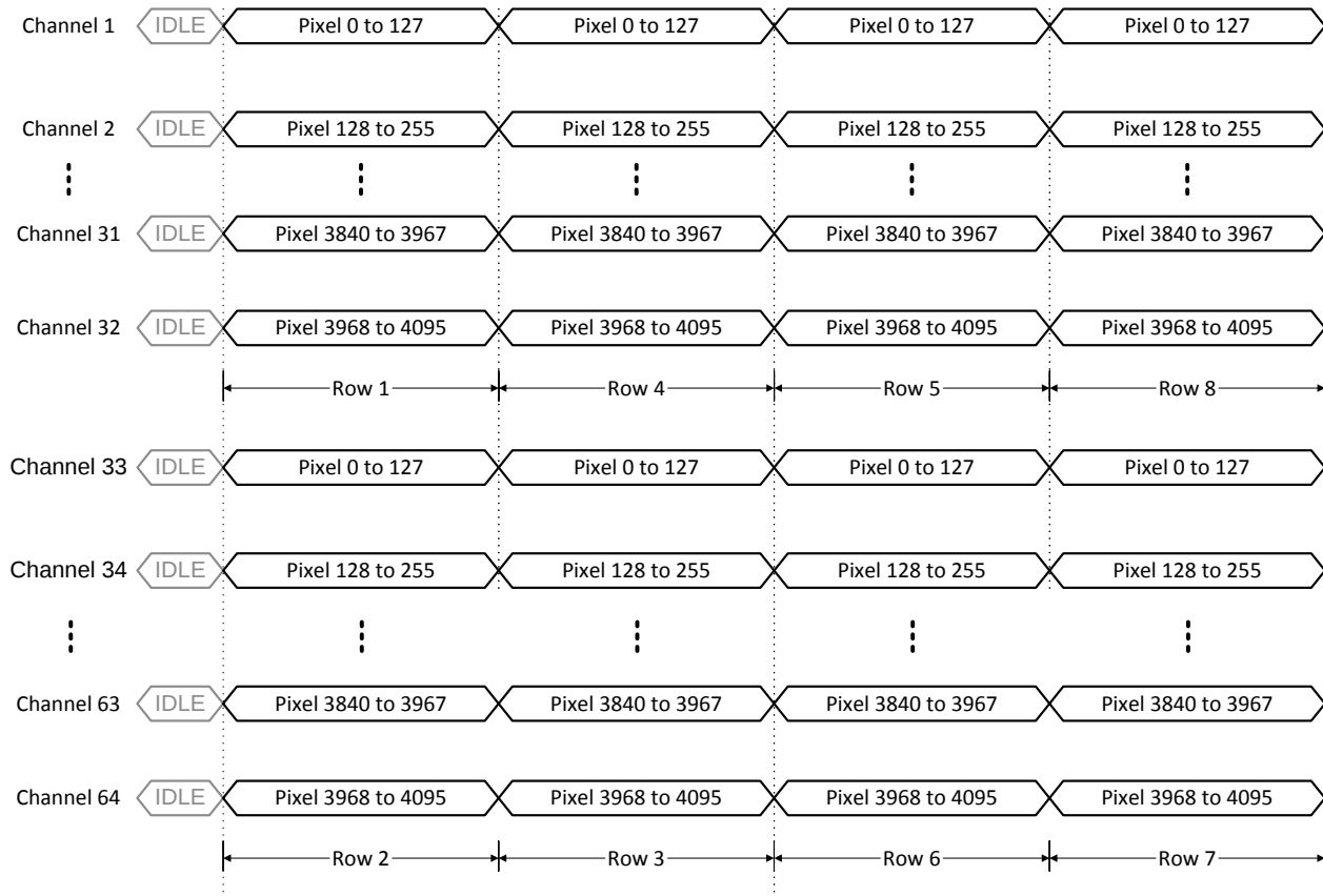
FIGURE 47: COLOR SUBSAMPLING IN Y, PIXEL TO OUTPUT REMAPPING
