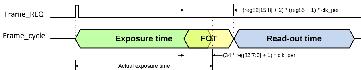
FIGURE 35: EXPOSURE OVERLAP DURING FOT
