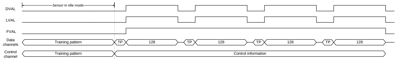
FIGURE 34: TRAINING PATTERN LOCATION IN THE DATA CHANNELS AND CONTROL CHANNEL
