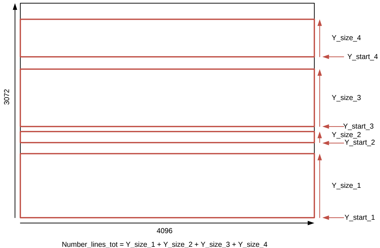
FIGURE 41: EXAMPLE OF 4 SUBWINDOWS READ-OUT
