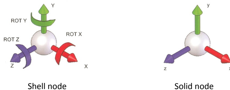
Figure 3-1 Nodal degrees of freedom for frames and shells; solids and trusses
