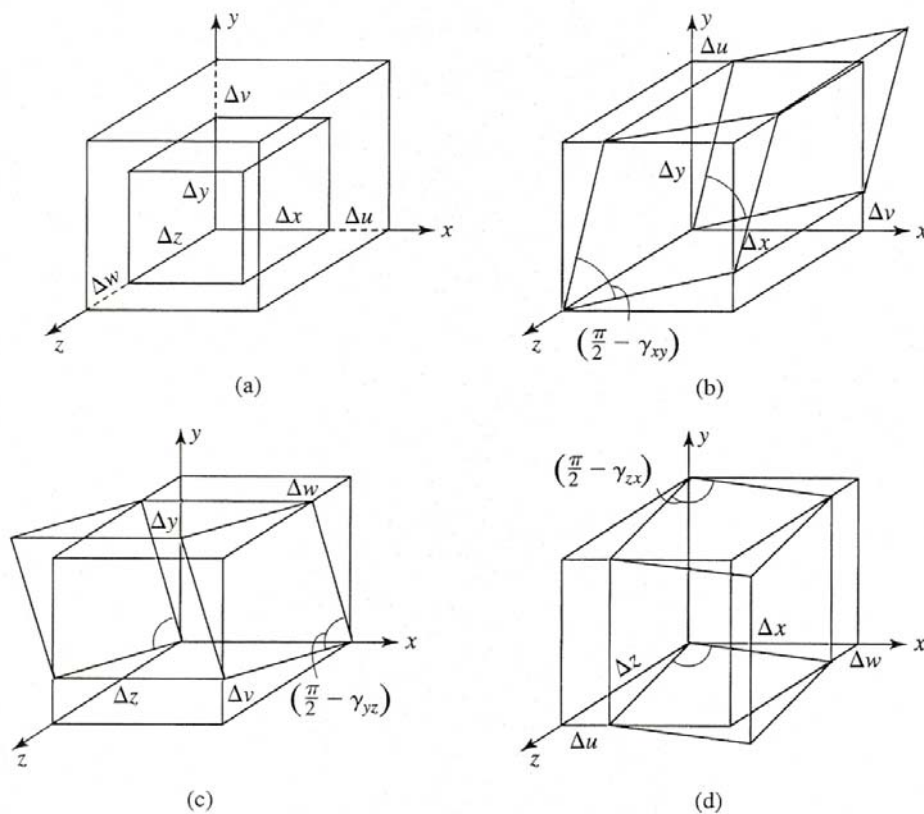
Figure 3-5 Graphical representations of 3D normal strains (a) and shear strains
