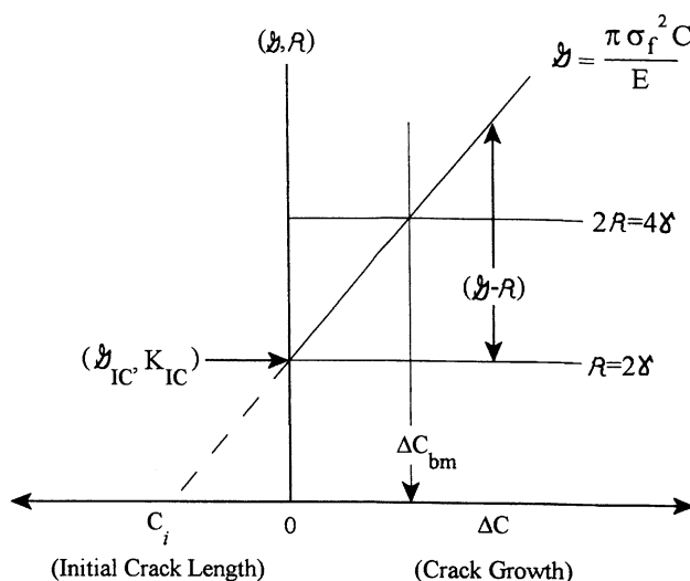
Fig. 11 The G , R versus crack length ( C_i and \Delta C ) diagram for fracture
