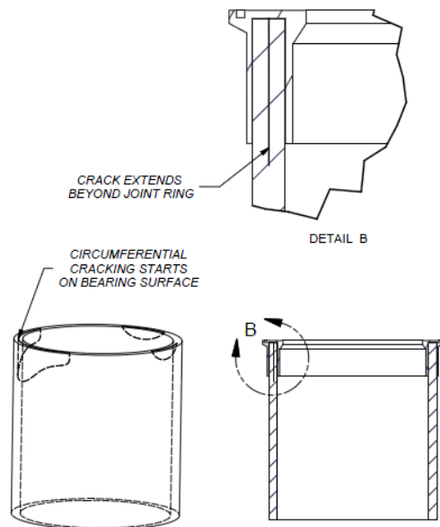
Fig.5 Circumferential cracking initiated by cyclic fatigue [4]
