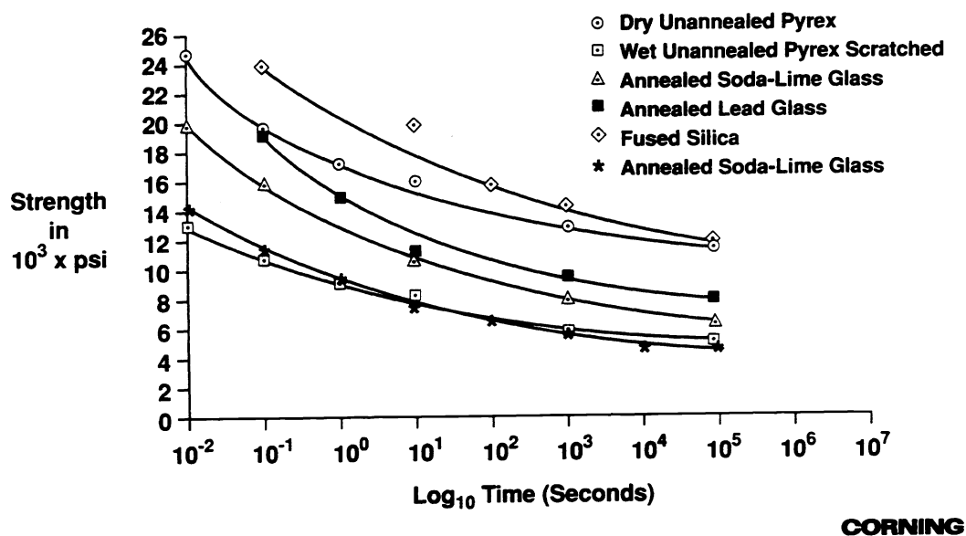
FIG. 6: Strength vs. Time Under Load in Glass
