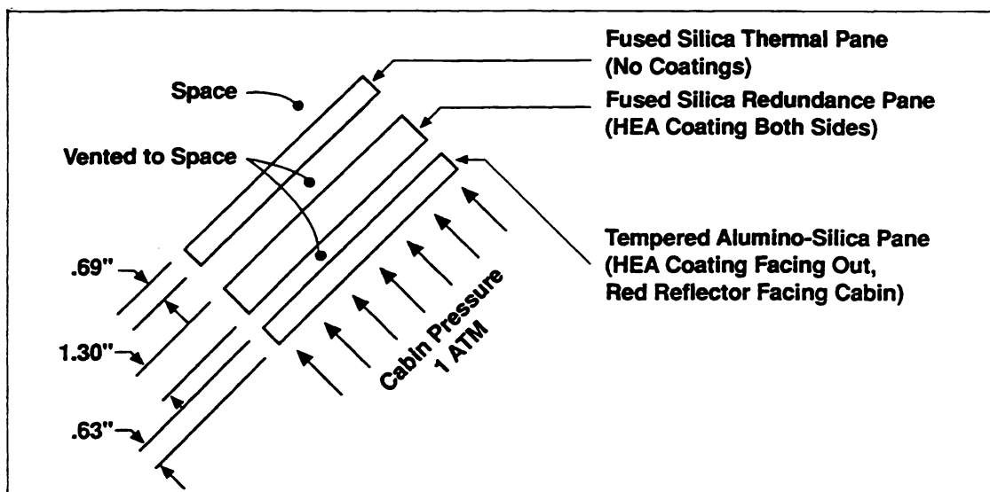
FIG. 5: Typical Design Shuttle Oribeter Forward Windshield
