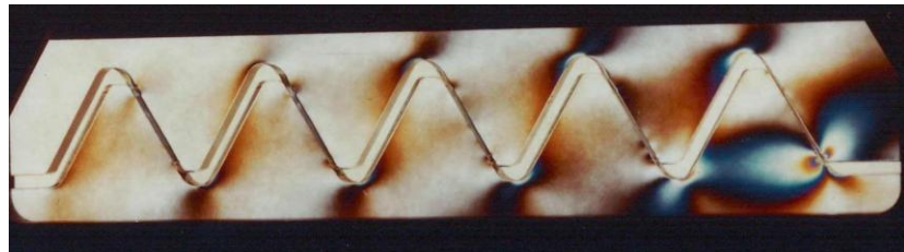
A photoelastic study shows the load distribution in a standard fastener [3]
