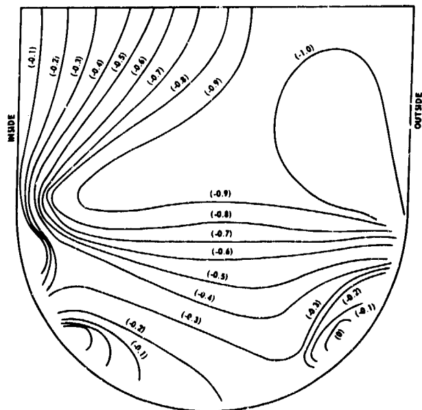
E_1 = 5 \times 10^6 h_1 = 0.010 \nu_1 = 0.30 W = 0.40 E_R = 30 \times 10^6 Model G39a
