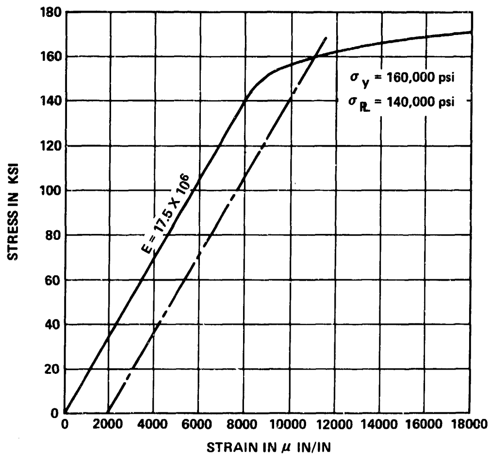
Figure 9 - Compressive Stress-Strain Curve for 662 Titanium
