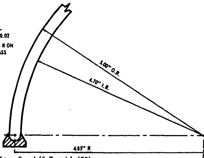
Figure 6c - R = h/2 Toroid (G3)
