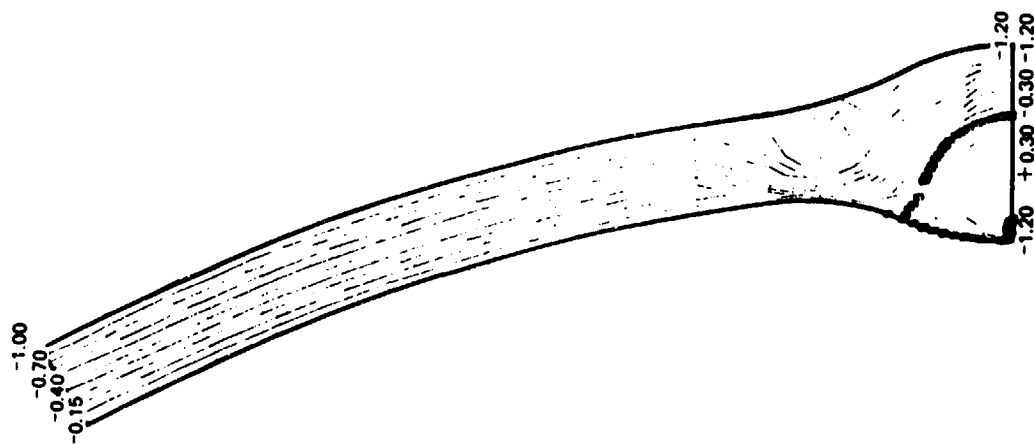
Figure 4b - Radial Stress
