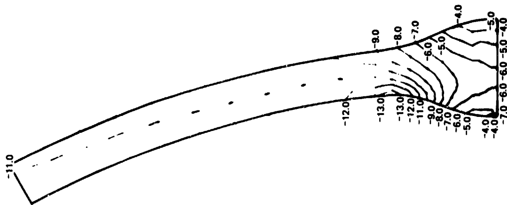
Figure 4c - Meridional Stress
