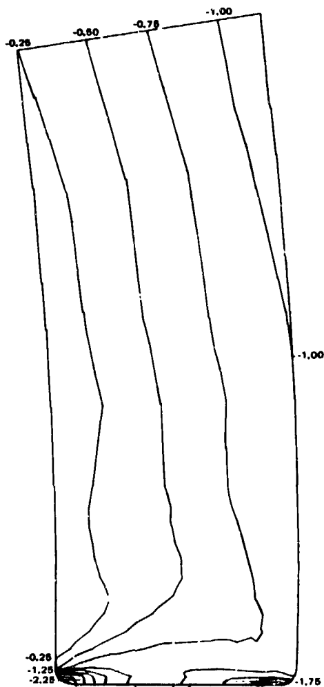
Figure 10e - Mod 1 Radial Stress
