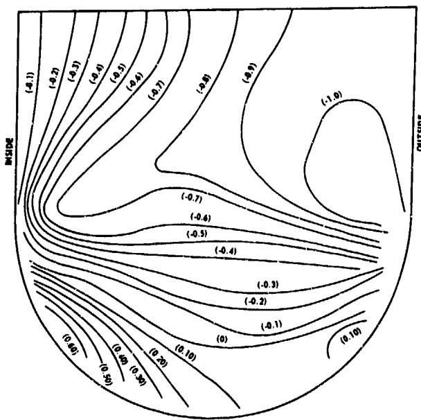
E_1 = 5 \times 10^6 h_1 = 0.010 \nu_1 = 0.30 W = 0.40 E_R = 15 \times 10^6 Model G39
