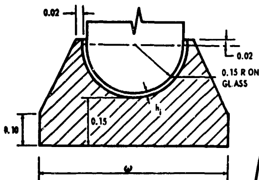
Figure 6b - R = h Toroid (G2)
