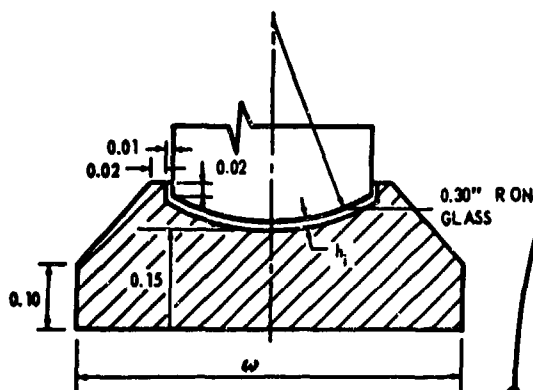
Figure 6a - Flat Juncture (G1)
