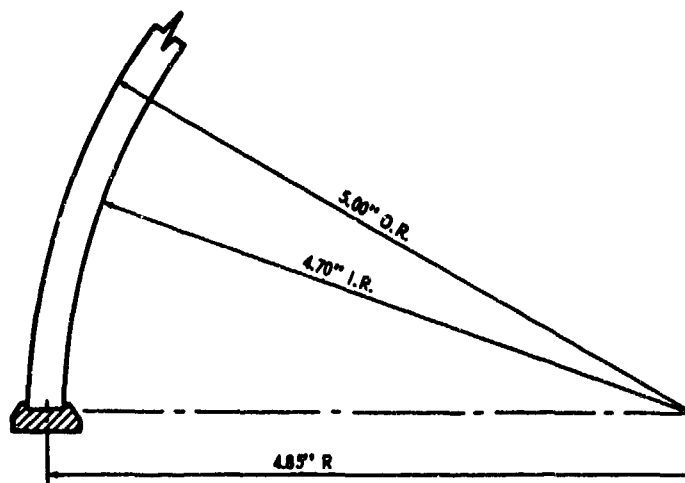
Figure 6a - Flat Juncture (G1)
