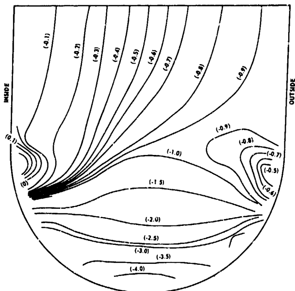
E_1 = 0.5 \times 10^6 \nu_1 = 0.45 h_1 = 0.040 Model G38a
