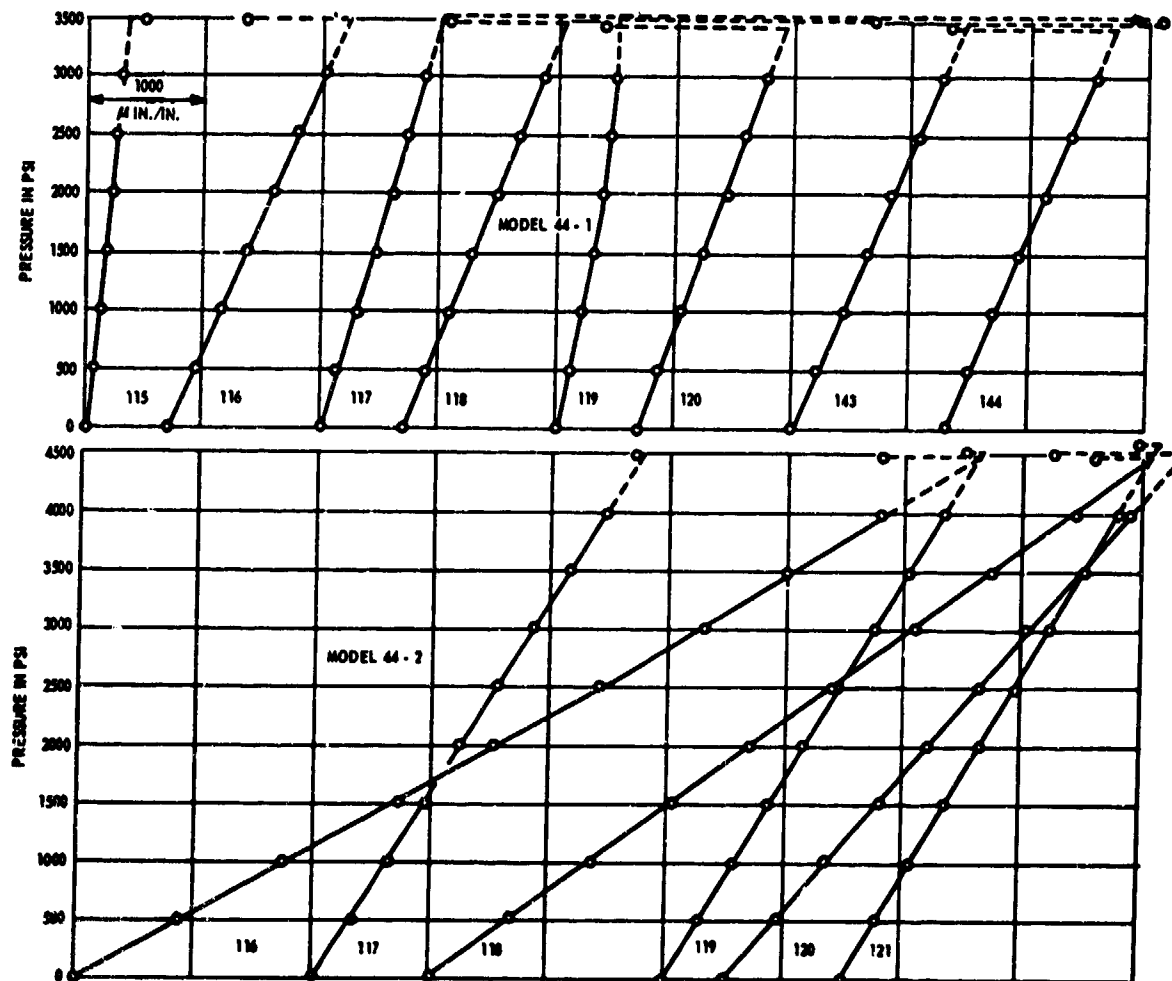
Figure 24 - Pressure Strain Plots for 44 Inch Glass Sphere
