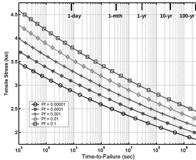
Figure 4.4 BK7 Design Strength Curve
