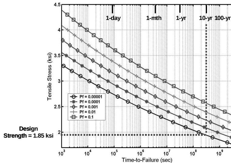
Figure 6.1 Corrector Design Strength Curves
