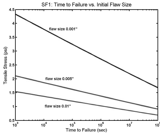
Figure 4.2 Time-to-Failure vs. Initial Flaw Size
