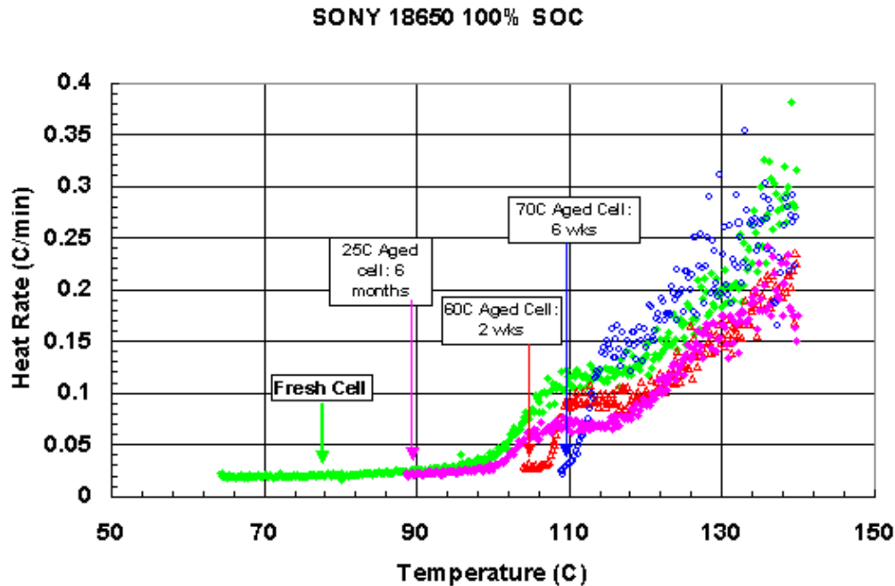
Figure 29. ARC runs of fresh and aged Sony cells at 100% SOC 37
