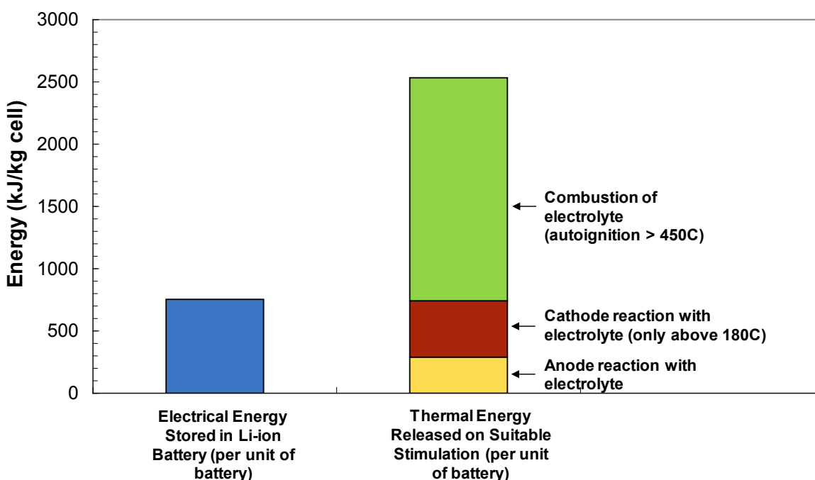
Figure 22. Comparison of stored electrical energy and energy released from decomposition reactions. 7
