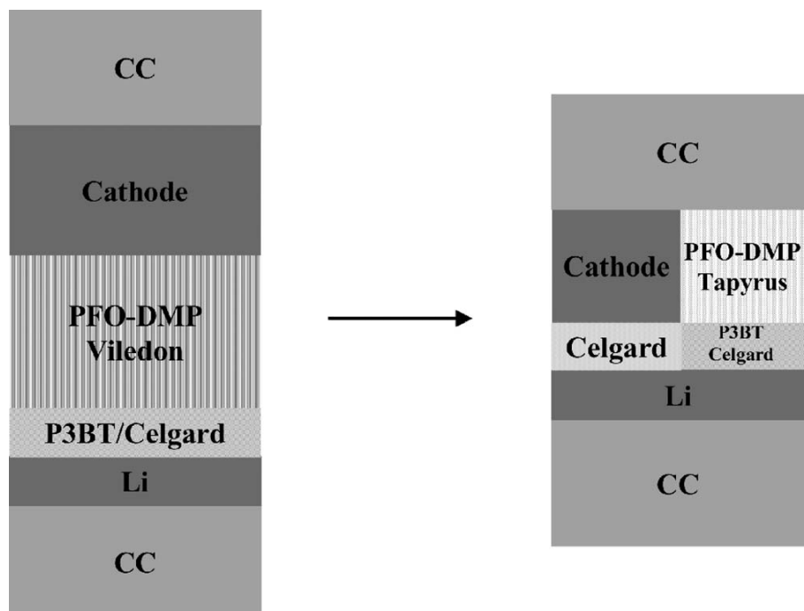
Figure 37. Schematic of alternative designs using electroactive separator for overcharge protection. 139
