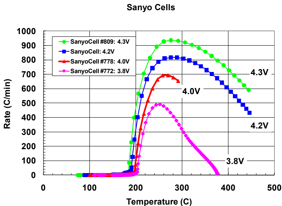
Figure 28. ARC profiles of Sanyo 18650 cells at increasing SOC.
