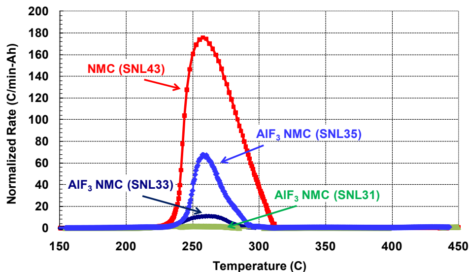
Figure 34. ARC profiles of 18650 cells with \text{AlF}_3 -coated and uncoated NMC cathodes.
