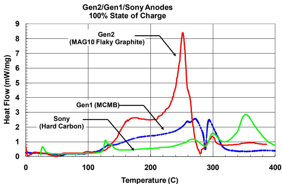
Figure 16. DSC profiles of anode carbon materials with different morphologies. 58
