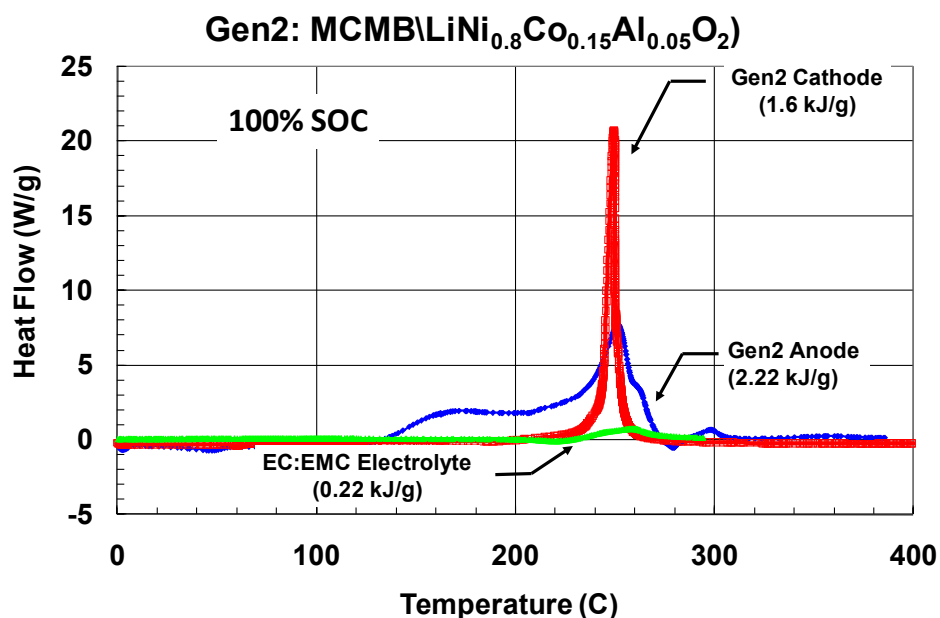
Figure 17. DSC profiles showing contribution of anode, cathode and electrolyte to cell thermal reactions. 57
