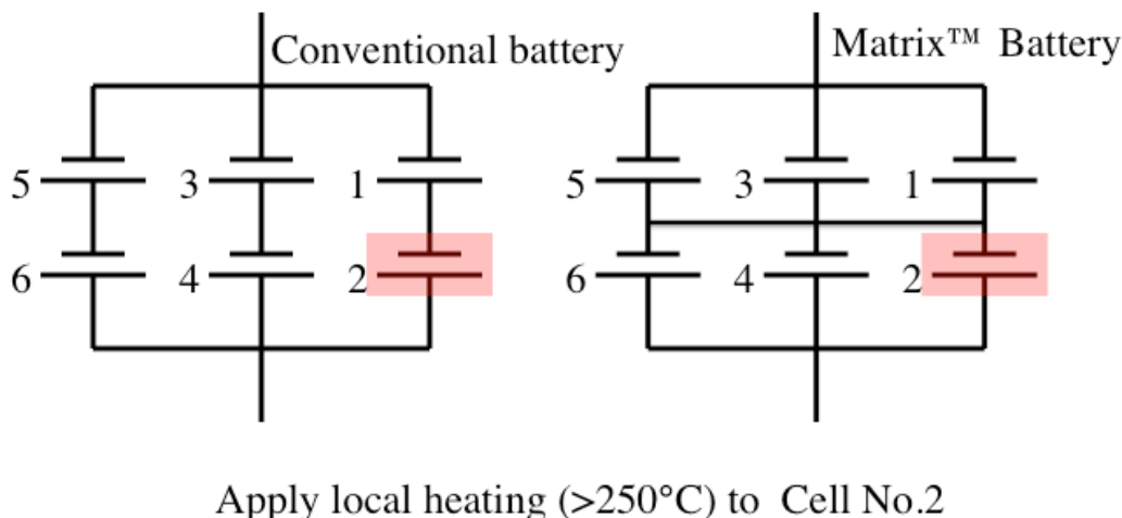
Figure 42. Wiring diagram of conventional and “Matrix” design in two battery packs. Cell No. 2 was driven into thermal runaway. The failure propagates to the entire battery in the conventional pack, but propagation DID NOT proceed in the “Matrix” pack. 176
