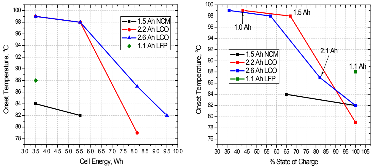
Figure 31. Self-heating onset temperature as a function of cell energy and SOC. 87
