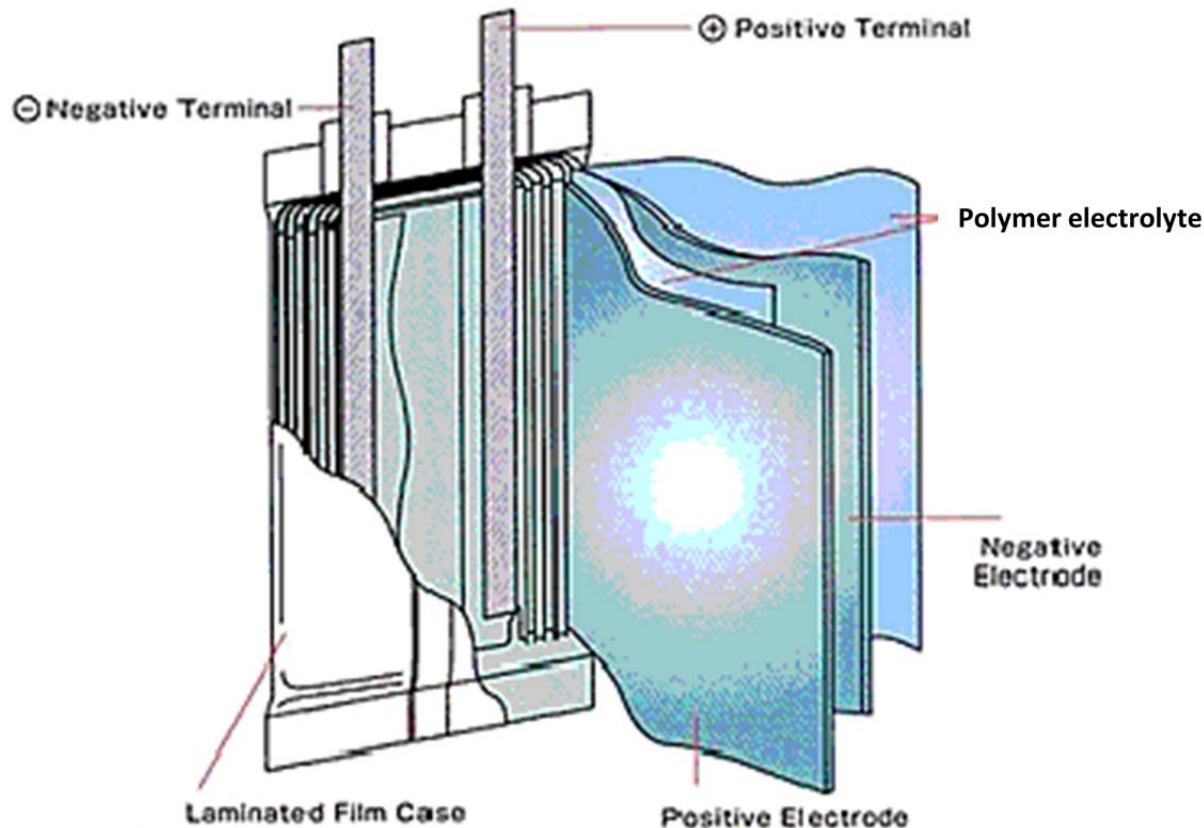
Figure 5. Illustration of Li-polymer battery. 11
