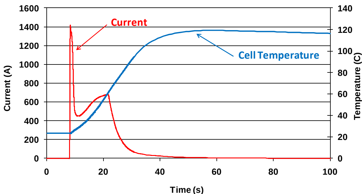
Figure 12. A 1-mOhm short circuit at room temperature of a Li-ion cell at 100% SOC. 69
