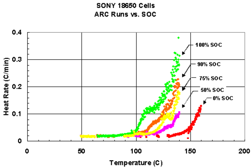
Figure 26. ARC runs for Sony 18650 cells versus SOC. 58
