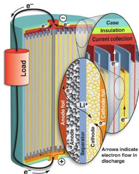
Figure 8. Cut-away drawing of cylindrical spirally wound Li-ion cell. 24
