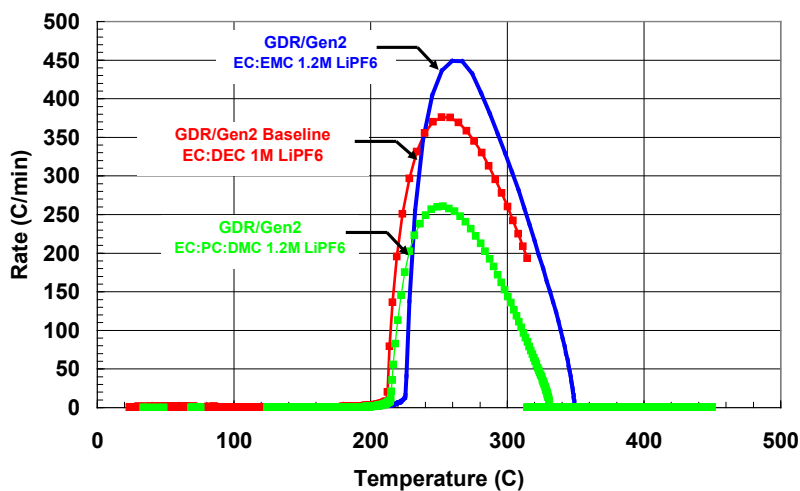
Figure 19. ARC profiles of GEN2 18650 cells with different solvent electrolyte species. 58
