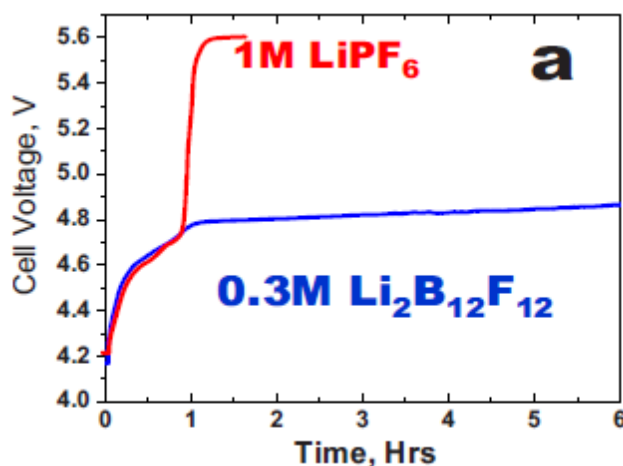
Figure 40. Effect of overcharge shuttle compared to normal cell during overcharge. The cell (MCMB anode and LiCoO2 cathode) was charged at 1C overcharge rate. 158
