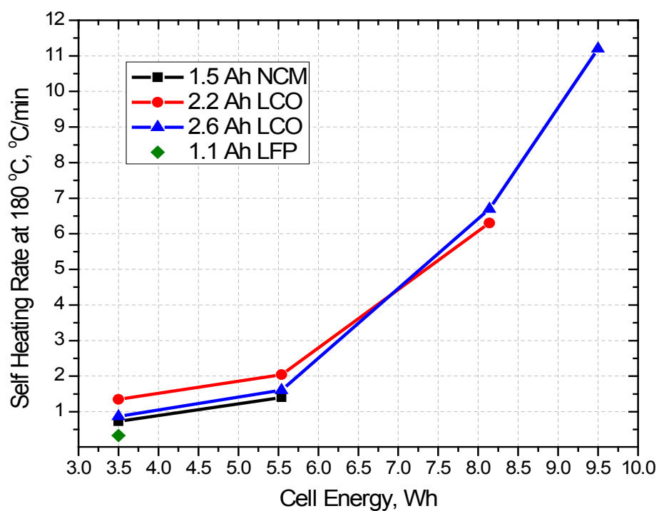
Figure 32. Self-heating rate at 180°C. 87
