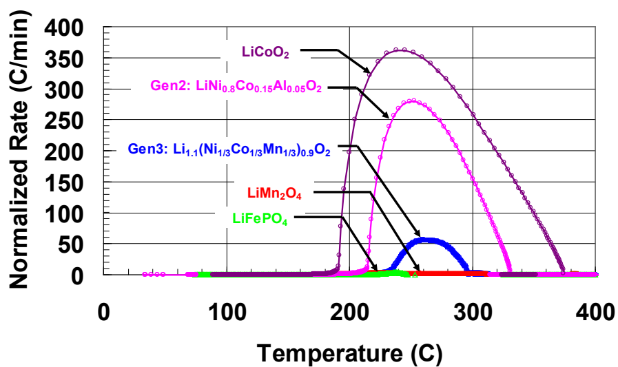
Figure 13. Self-heating rate of 18650 full cell measured by ARC. Improved cathode stability results in higher thermal runaway temperature (increased stability) and reduced peak heating rate. 69
