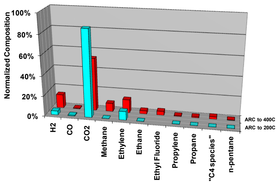
Figure 25. Gas generation species for EC:EMC 1.2 M LiPF 6 electrolyte at 200°C and 400°C. (Unpublished SNL data)
