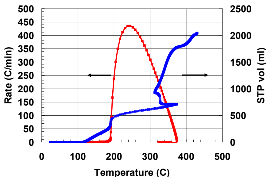
Figure 23. ARC thermal runaway profile of an 18650 cell (5 mL electrolyte) showing heat and gas generation.
