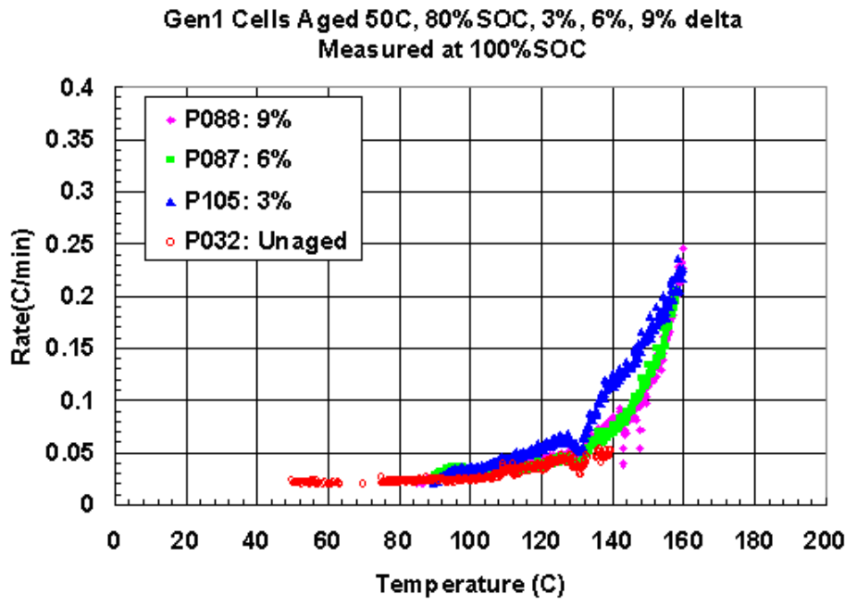
Figure 30. ARC runs of GEN1 cells (100% SOC) aged at 50°C, 8% SOC, at 2%, 6% and 9% delta SOC. 37
