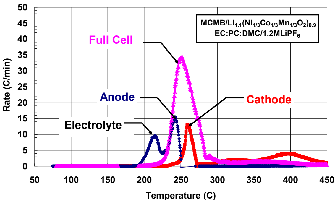
Figure 21. ARC profiles of anode and cathode electrodes in electrolyte compared to full cell response. 58
