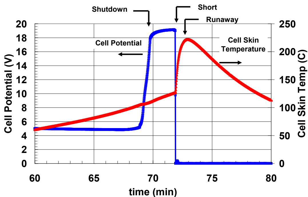
Figure 10. Thermal runaway during overcharge due to separator failure following separator shutdown. 67
