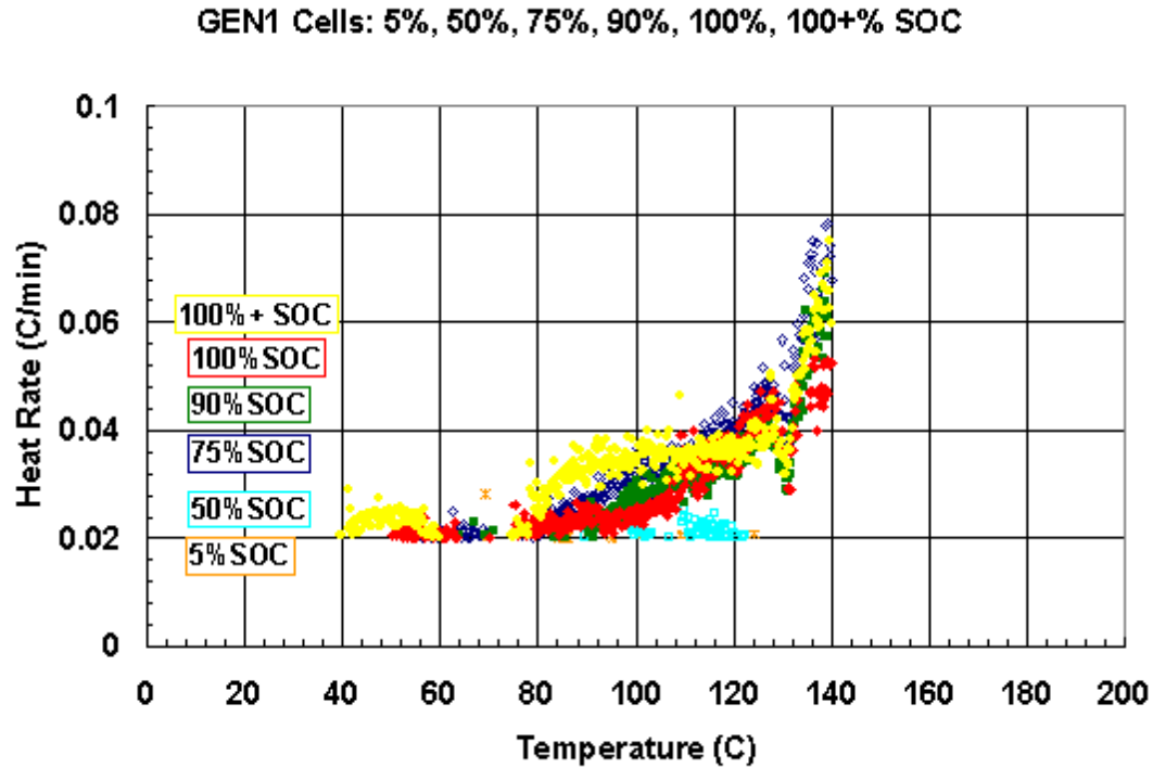
Figure 27. ARC runs for GEN1 cells vs. SOC. 37
