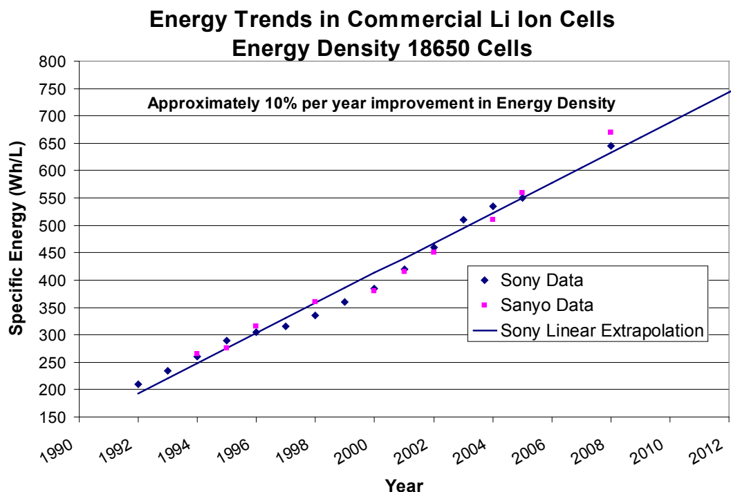
Figure 4. Energy density trends for commercial Li-ion cells. 9
