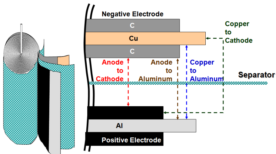
Figure 41. Sources of variability in internal short circuit test arise because there are four kinds of internal short circuit conditions. 85
