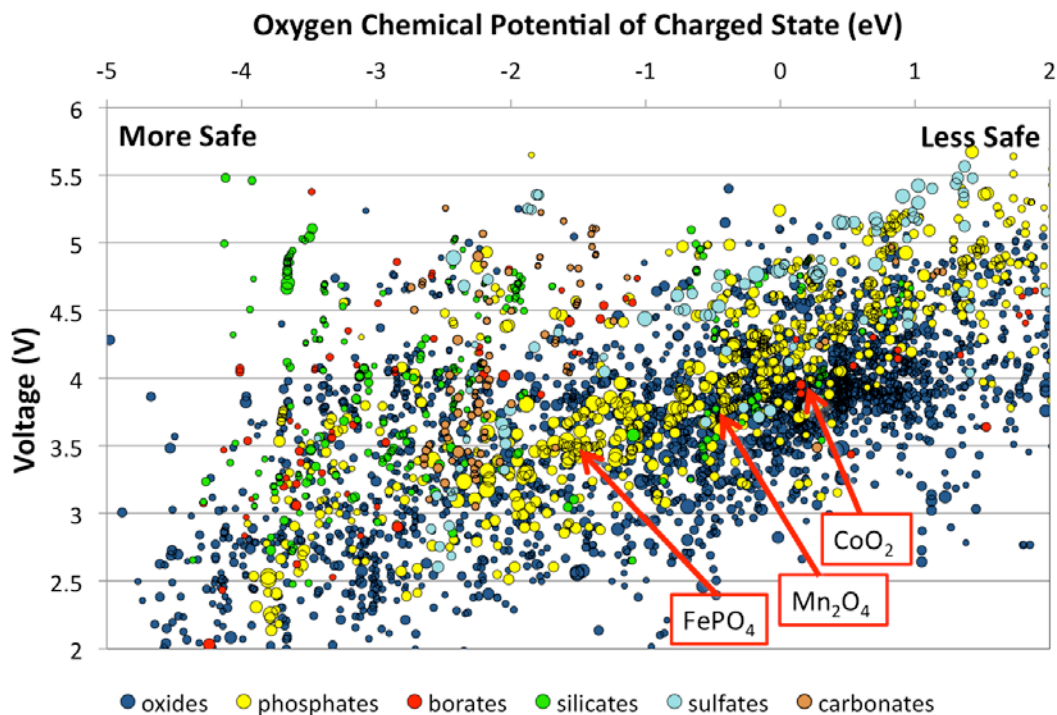
Figure 33. Calculated relationship between oxygen chemical potential at full charge and voltage for many cathodes.
