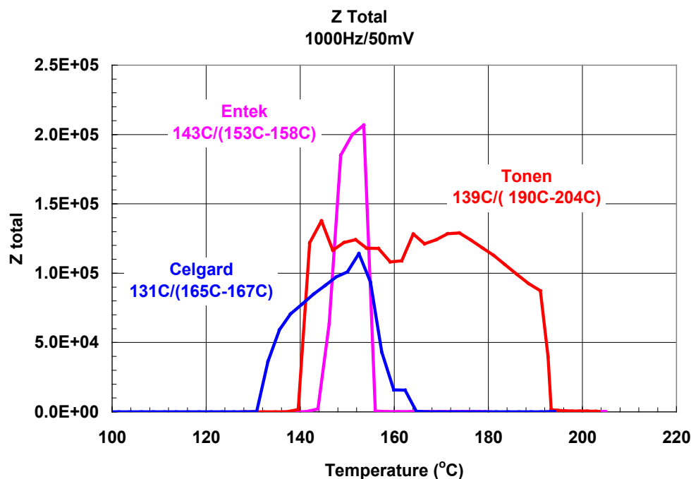
Figure 18. Impedance of electrolyte soaked separator materials showing shutdown and the temperature window of stability. 58
