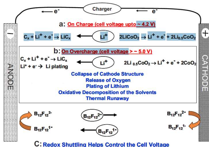
Figure 39. StabiLife Salt used as redox shuttle from Air Products 158
