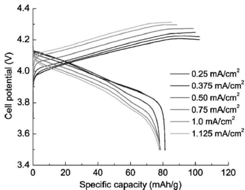
Figure 38. Rate performance of a protected \text{Li}_{1.05}\text{Mn}_{1.95}\text{O}_4 -Li cell with the bilayer, parallel cell configuration. 139
