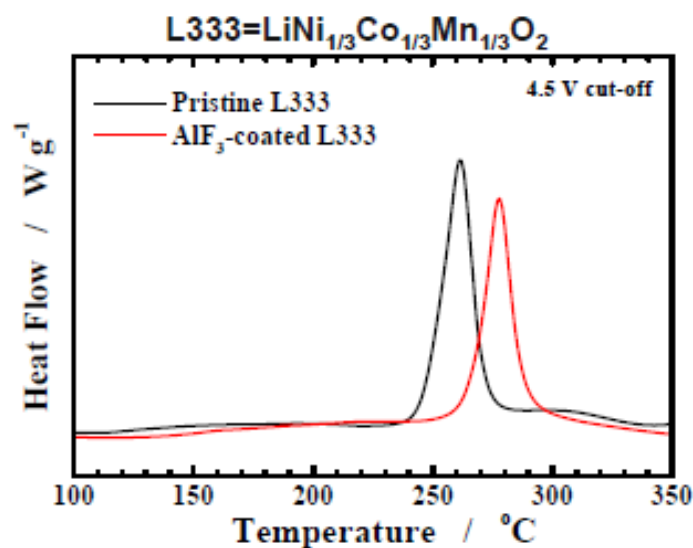
Figure 35. DSC measurements of AlF 3 -coated and uncoated NMC cathodes. 105
