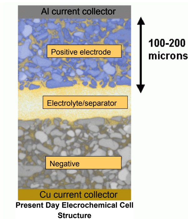
Figure 7. Electrode and cell structure of Li-ion rechargeable batteries. 24
