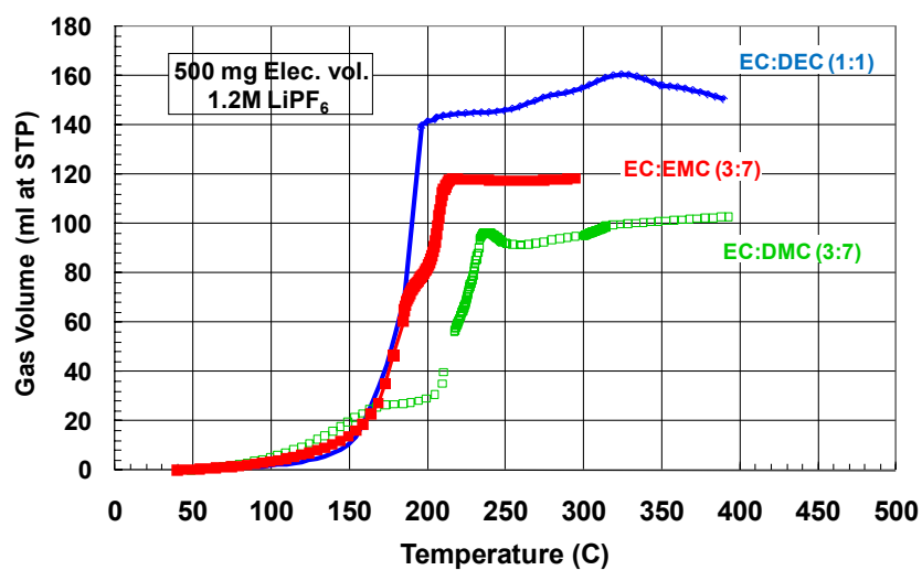
Figure 24. Gas generation of representative electrolyte solutions. (Unpublished SNL data)
