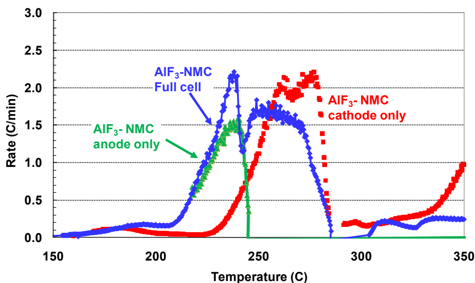
Figure 36. ARC measurements of full cell and individual 18650 electrodes with AlF 3 -coated NMC cathodes.
