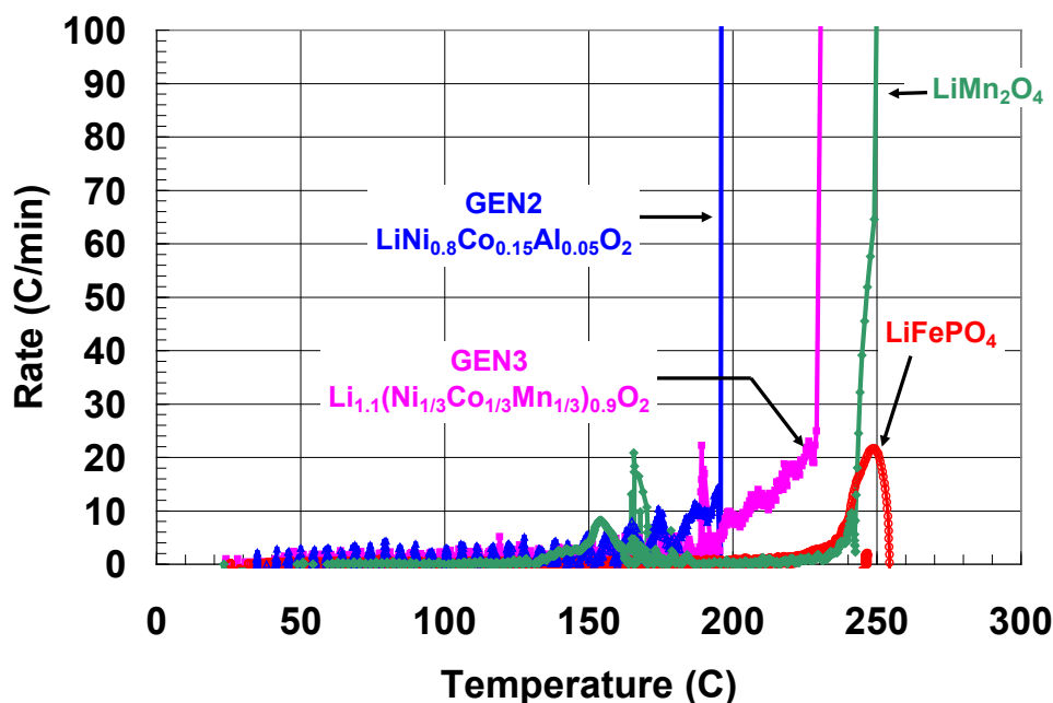
Figure 15. Onset of self-heating in thermal ramp experiment on Li-ion cells. \text{LiFePO}_4 olivine cathodes show the greatest reduction in self-heating rate and increased onset temperature for runaway. 37
