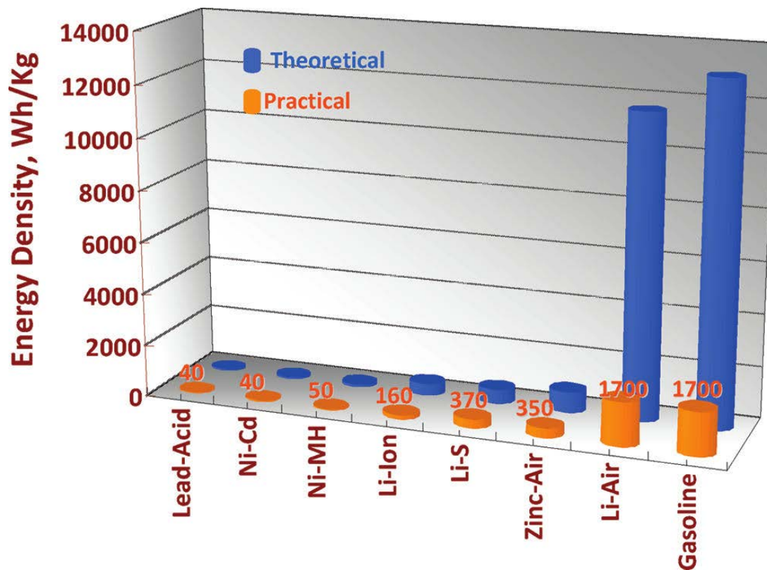
Figure 1. The gravimetric energy densities (Wh/kg) for various types of rechargeable batteries compared to gasoline. 3
