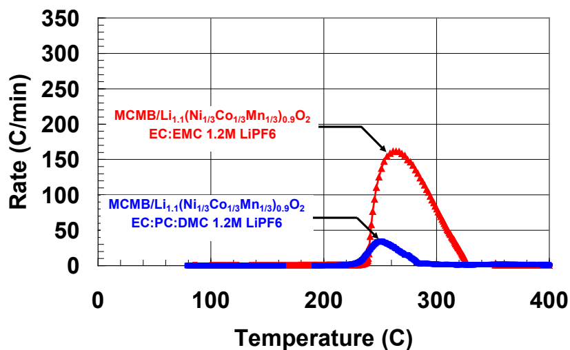
Figure 20. ARC profiles for GEN3 18650 cells with EC:EMC (3:7) and EC:PC:DMC (1:1:3) electrolyte solvents. 58
