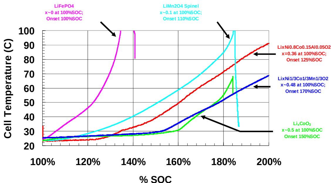
Figure 11. Heat output during overcharge for different cathode oxide chemistries, showing a marked increase in heat output when final lithium is removed from cathode. 68
