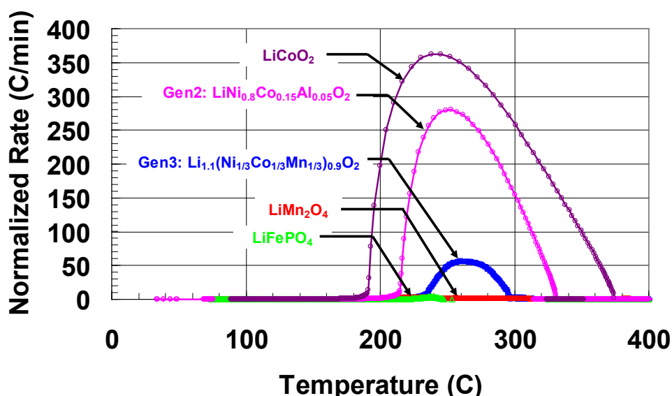
Figure S-1. Self-heating rate of the 18650 full cell as measured by accelerating rate calorimetry (ARC). Improving cathode stability results in a higher thermal runaway temperature (increased stability) and a reduced peak heating rate.
