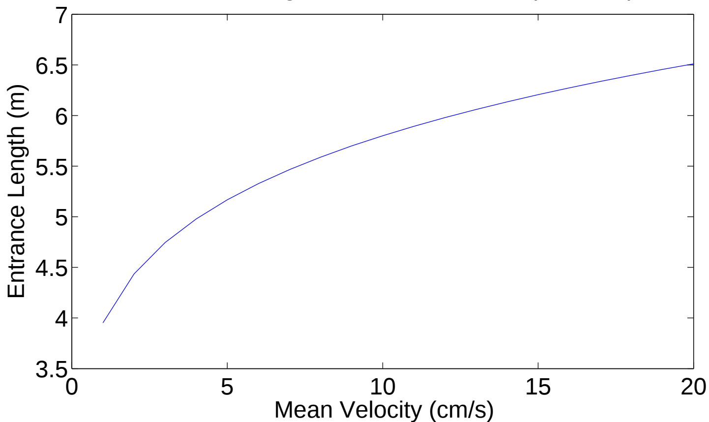
Turbulent Entrance Lengths for 10" Diameter Pipe Flow (seawater)
