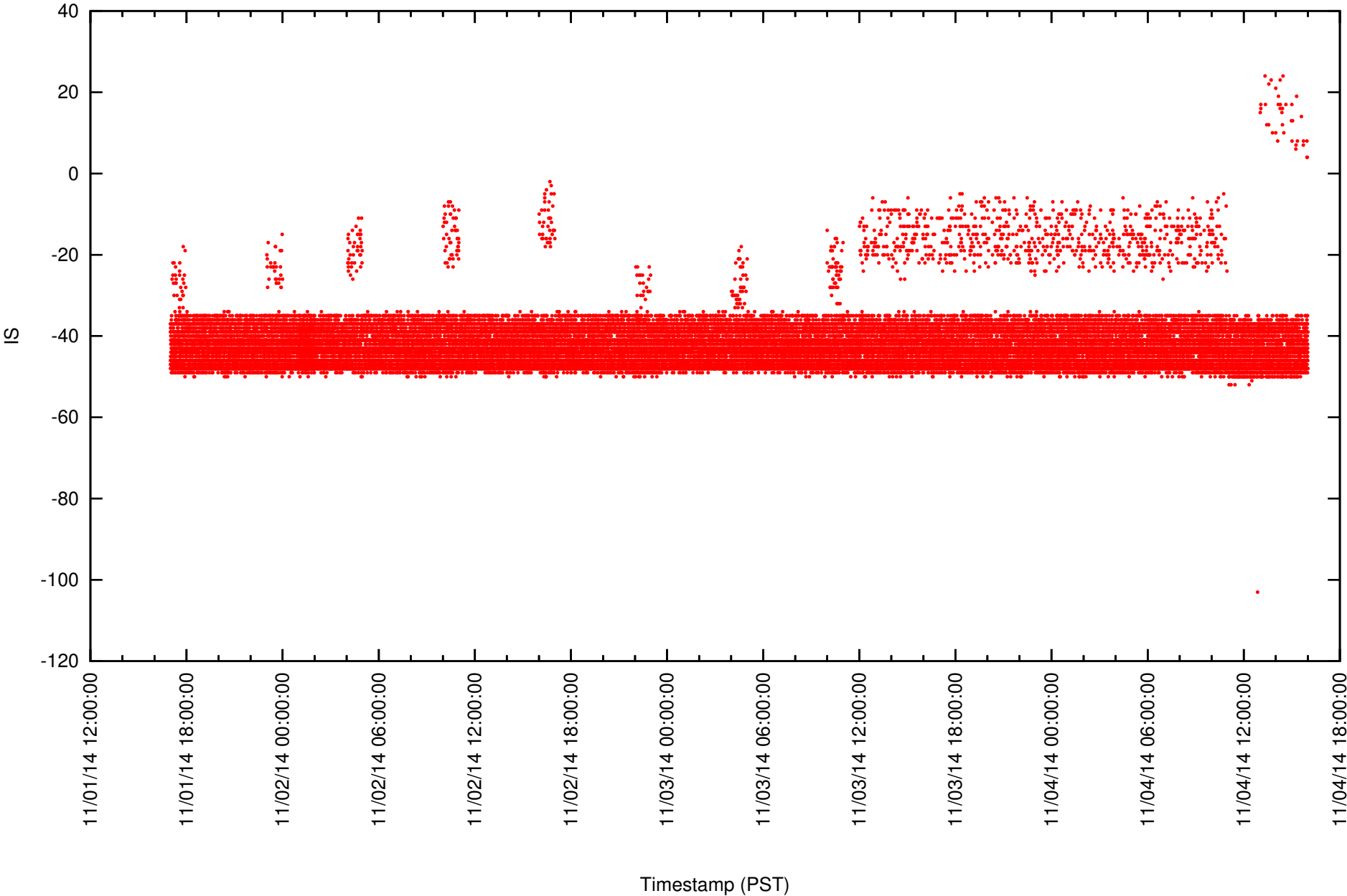
Motor Controller IS (counts) vs Time
