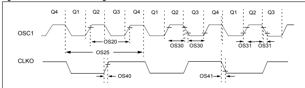
Figure 6-10: External Clock Timing
