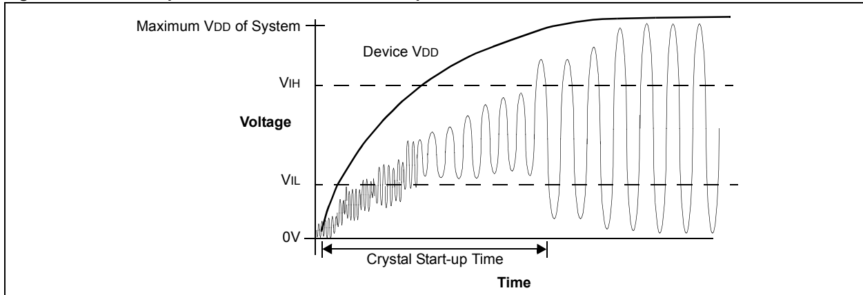
Figure 6-4: Example Oscillator/Resonator Start-up Characteristics
