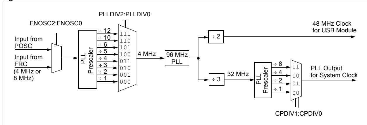
Figure 6-8: USB PLL Block
