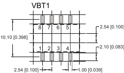
RECOMMENDED FOOTPRINT Top view, grid: 2.54mm(0.1inch)
