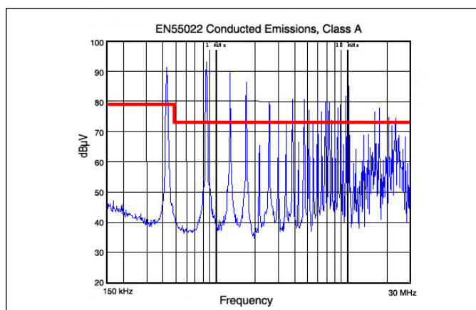
Figure 4-2 — V48B28H250BN without bypass caps (330 μF across input)
