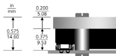
Figure 15-4 — Through-hole or threaded baseplate; Height above board with standoff
